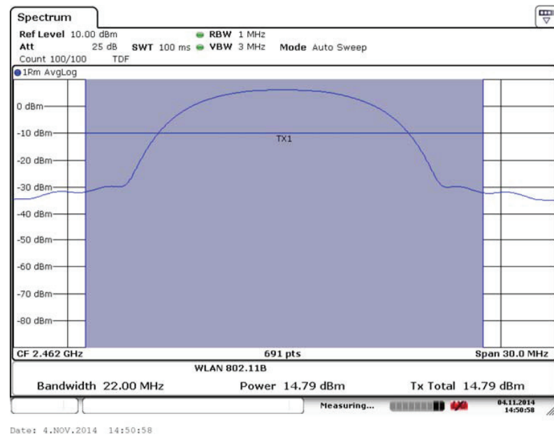
Fig. 9 Maximum Average Output Power (802.11b, Ch 11,5Mbps)
