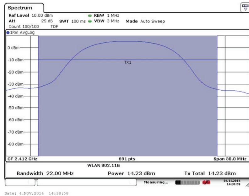
Fig. 10 Maximum Average Output Power (802.11b, Ch 1,1Mbps)
