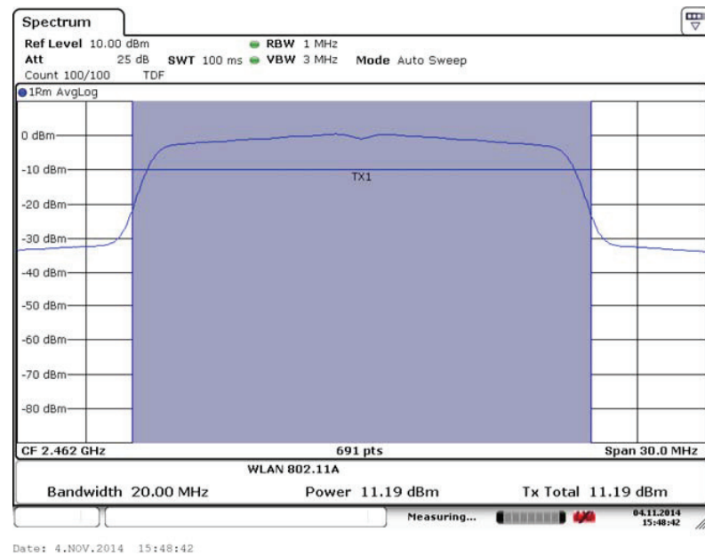
Fig. 42 Maximum Average Output Power (802.11n-20MHz, Ch 11,MCS1)
