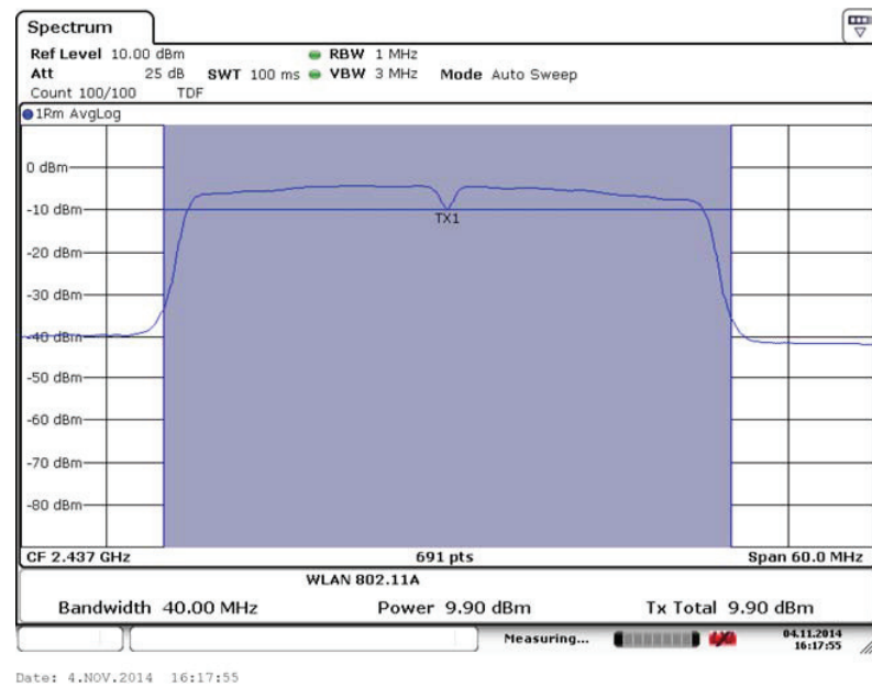
Fig. 74 Maximum Average Output Power (802.11n- 40MHz,Ch6,MCS4)
