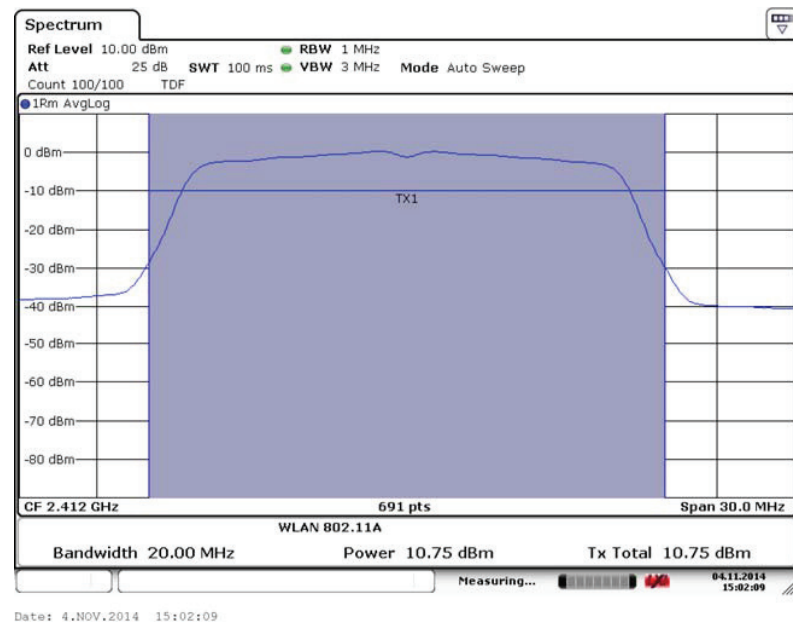
Fig. 31 Maximum Average Output Power (802.11g, Ch 1,48Mbps)
