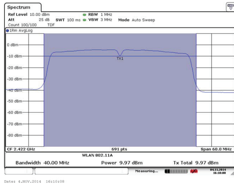
Fig. 64 Maximum Average Output Power (802.11n- 40MHz,Ch1,MCS1)
