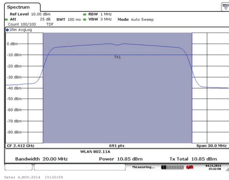
Fig. 43 Maximum Average Output Power (802.11n-20MHz, Ch 1,MCS2)
