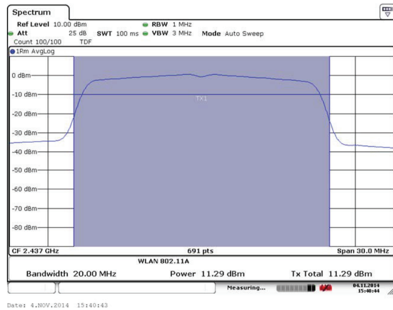
Fig. 47 Maximum Average Output Power (802.11n-20MHz, Ch 6,MCS3)
