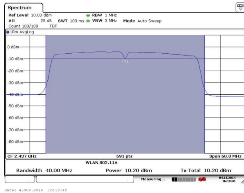
Fig. 65 Maximum Average Output Power (802.11n- 40MHz,Ch6,MCS1)
