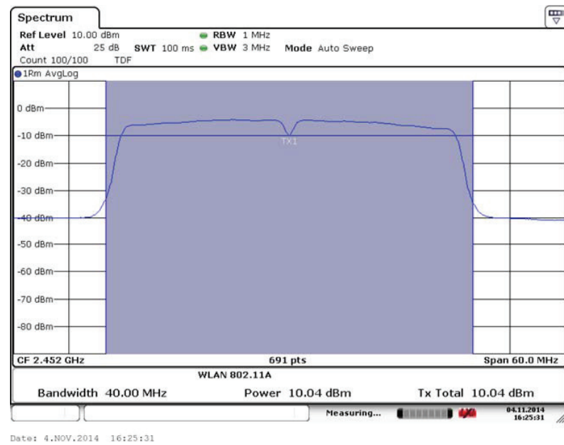
Fig. 69 Maximum Average Output Power (802.11n- 40MHz,Ch11,MCS2)
