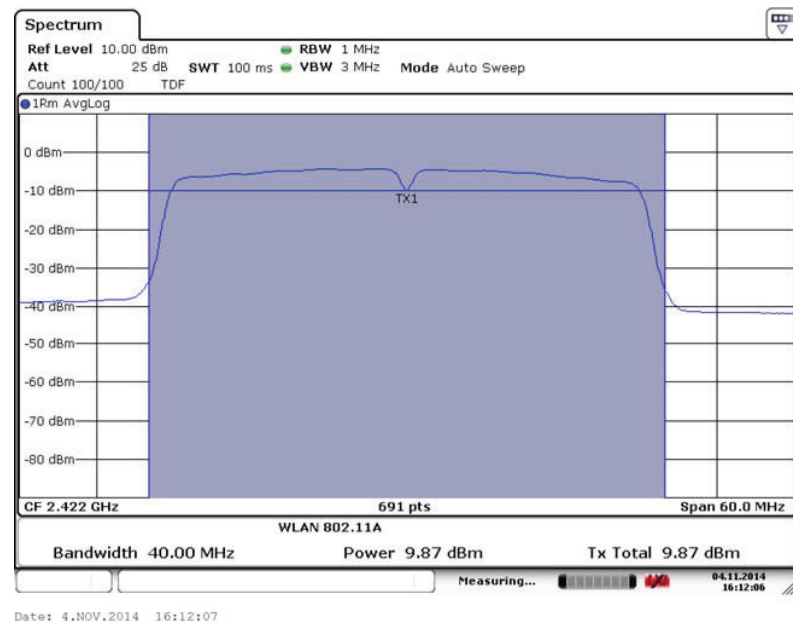
Fig. 70 Maximum Average Output Power (802.11n- 40MHz,Ch1,MCS3)
