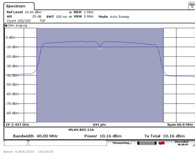
Fig. 71 Maximum Average Output Power (802.11n- 40MHz,Ch6,MCS3)
