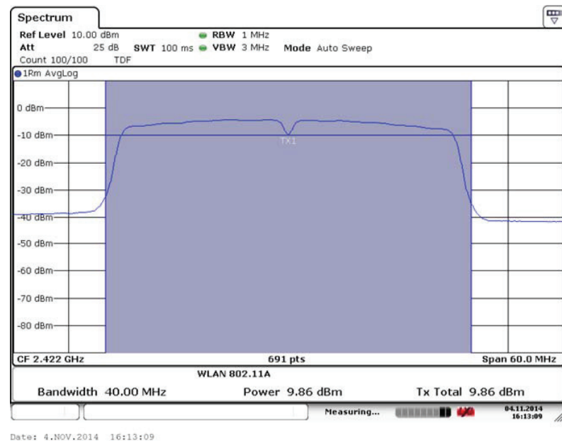
Fig. 76 Maximum Average Output Power (802.11n- 40MHz,Ch1,MCS5)
