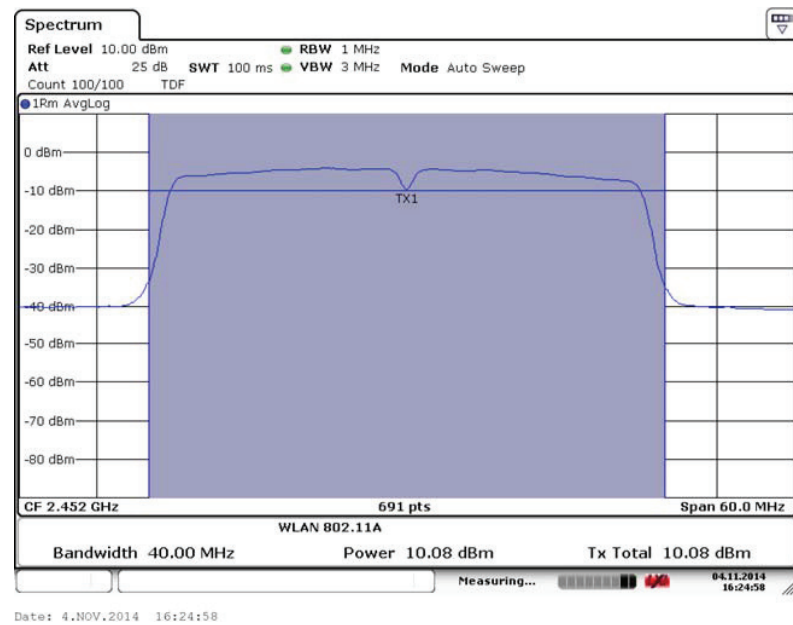
Fig. 66 Maximum Average Output Power (802.11n- 40MHz,Ch11,MCS1)
