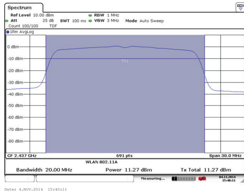
Fig. 50 Maximum Average Output Power (802.11n-20MHz, Ch 6,MCS4)
