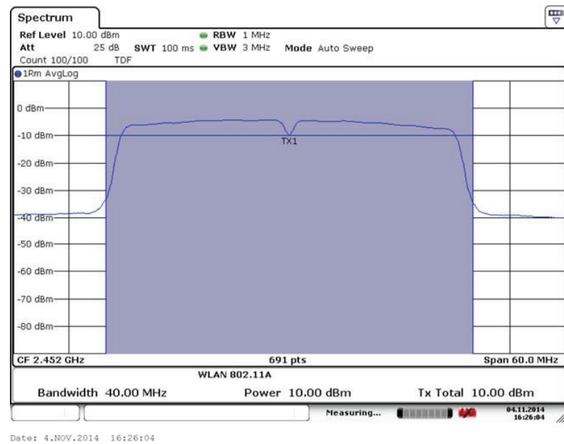
Fig. 72 Maximum Average Output Power (802.11n- 40MHz,Ch11,MCS3)
