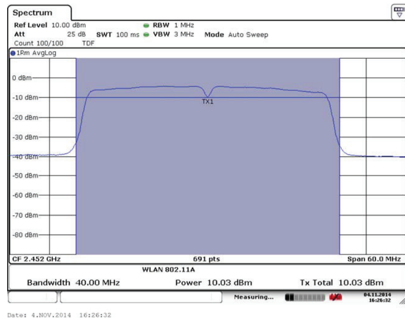
Fig. 75 Maximum Average Output Power (802.11n- 40MHz,Ch11,MCS4)
