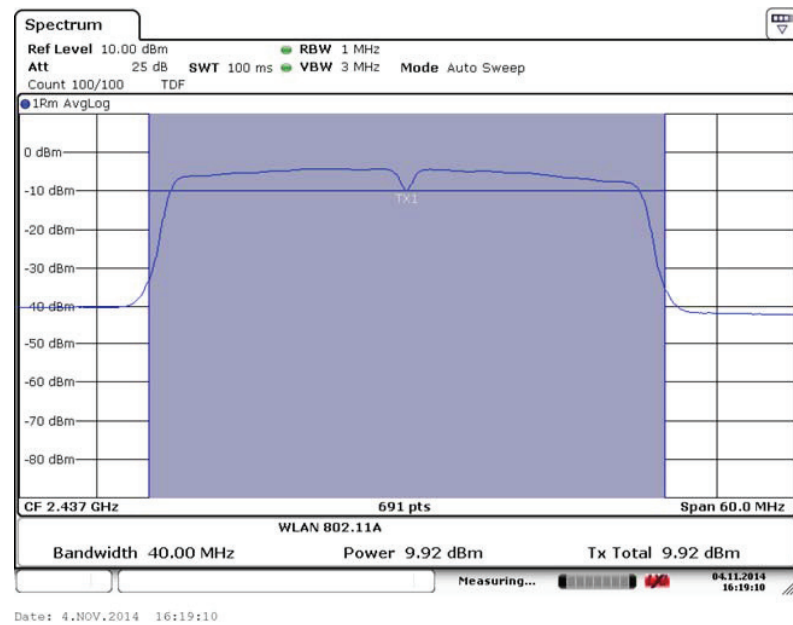
Fig. 68 Maximum Average Output Power (802.11n- 40MHz,Ch6,MCS2)
