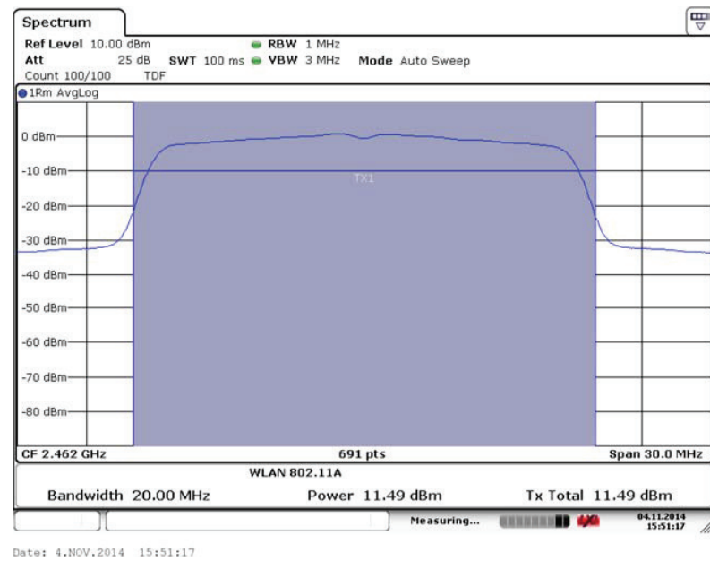
Fig. 51 Maximum Average Output Power (802.11n-20MHz, Ch 11,MCS4)
