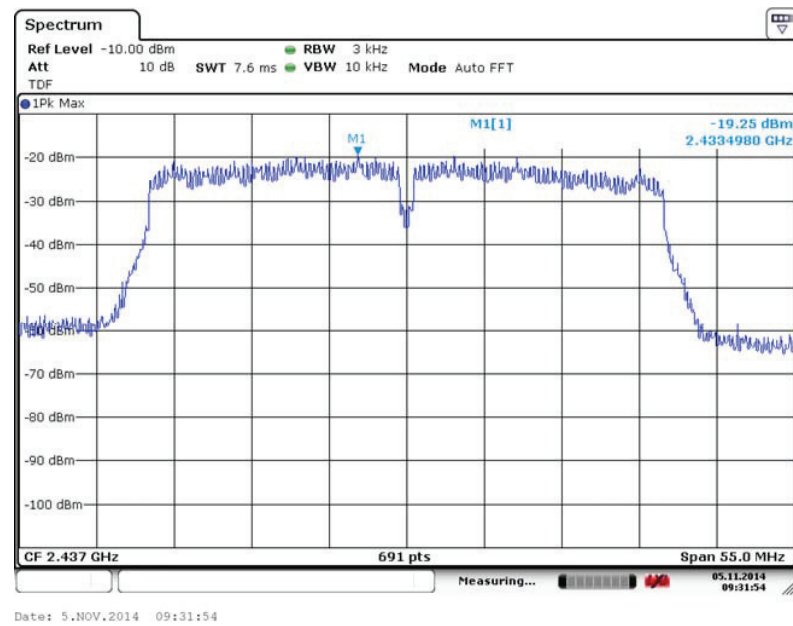
Fig. 95 Power Spectral Density (802.11n-40MHz, Ch 6)
