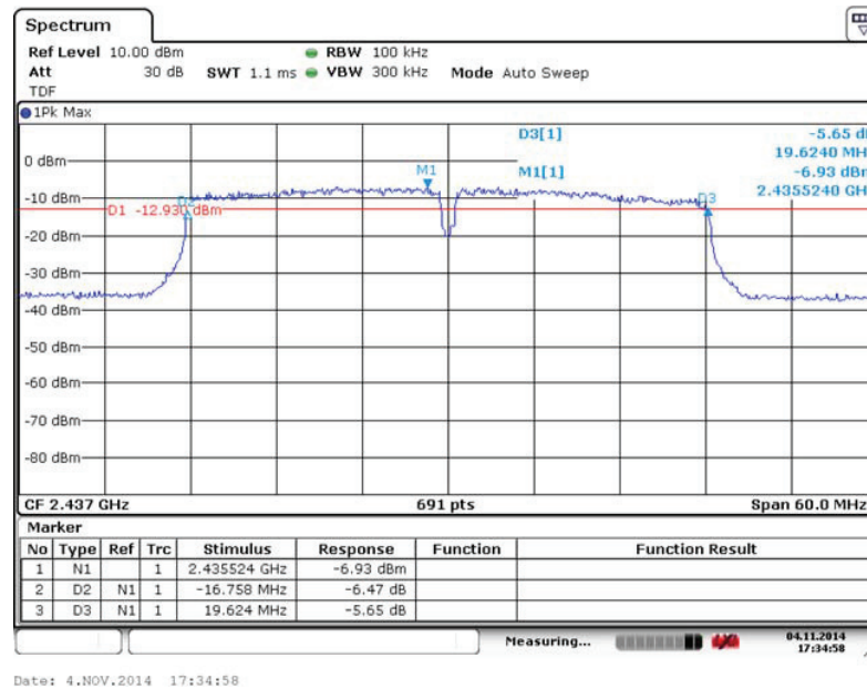
Fig. 107 Occupied 6dB Bandwidth (802.11n-40MHz, Ch 6)
