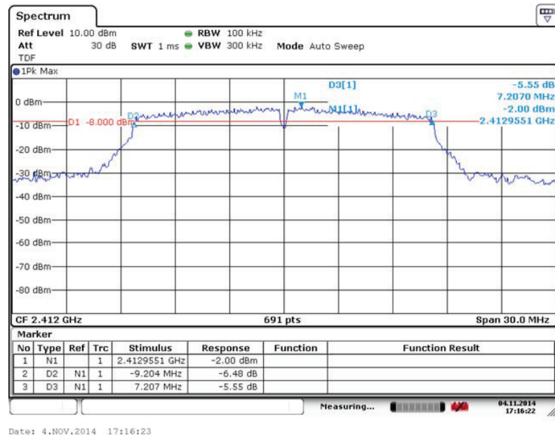
Fig. 100 Occupied 6dB Bandwidth (802.11g, Ch 1)
