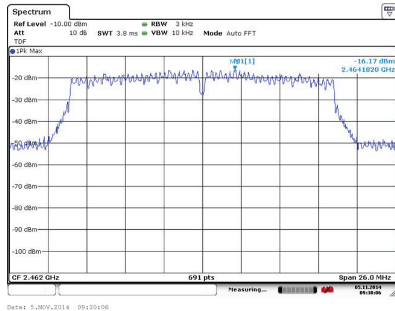
Fig. 93 Power Spectral Density (802.11n-20MHz, Ch 11)
