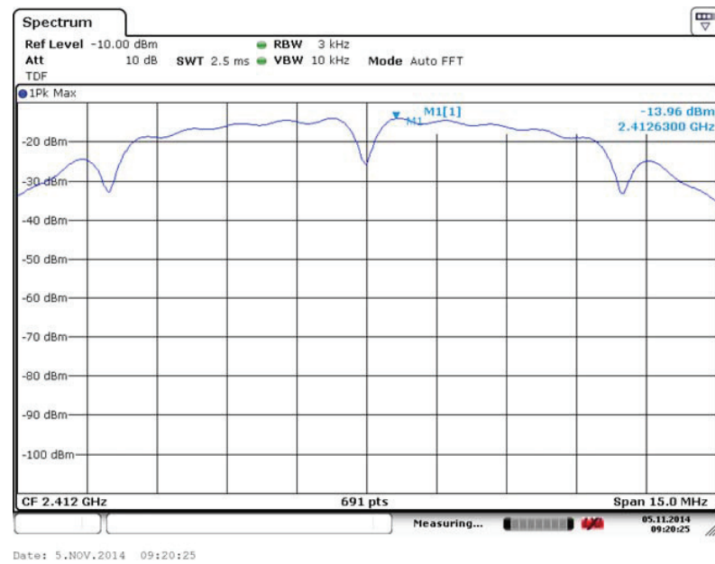
Fig. 85 Power Spectral Density (802.11b, Ch 1)
