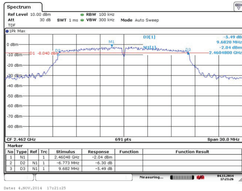
Fig. 102 Occupied 6dB Bandwidth (802.11g, Ch 11)
