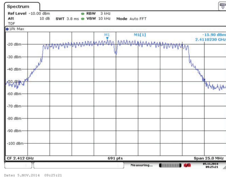
Fig. 88 Power Spectral Density (802.11g, Ch 1)
