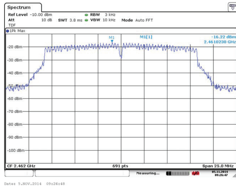
Fig. 90 Power Spectral Density (802.11g, Ch 11)
