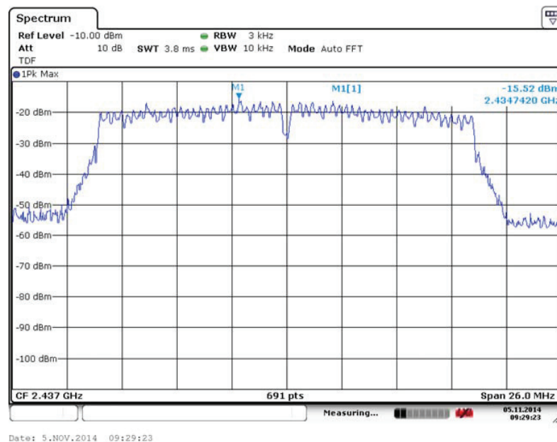
Fig. 92 Power Spectral Density (802.11n-20MHz, Ch 6)
