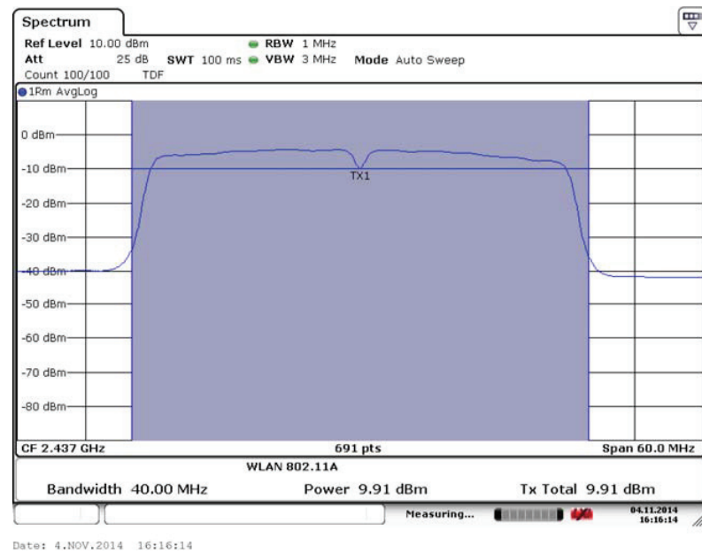
Fig. 80 Maximum Average Output Power (802.11n- 40MHz,Ch6,MCS6)
