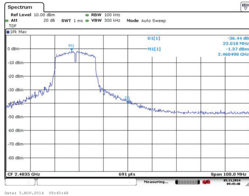
Fig. 112 Band Edges (802.11g, Ch 11)
