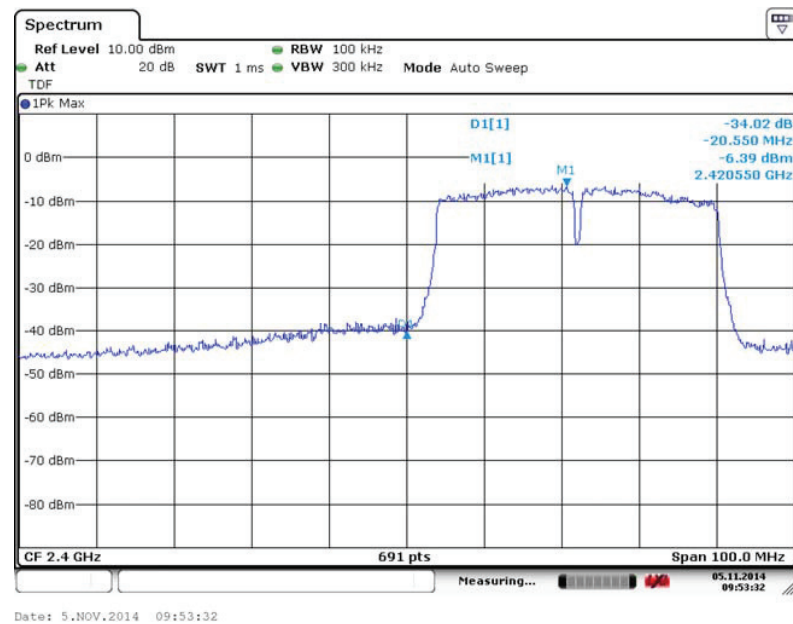
Fig. 115 Band Edges (802.11 n-40MHz, Ch 3)
