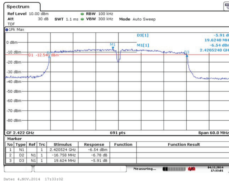
Fig. 106 Occupied 6dB Bandwidth (802.11n-40MHz, Ch 3)
