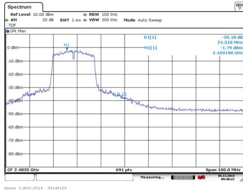
Fig. 114 Band Edges (802.11 n-20MHz, Ch 11)
