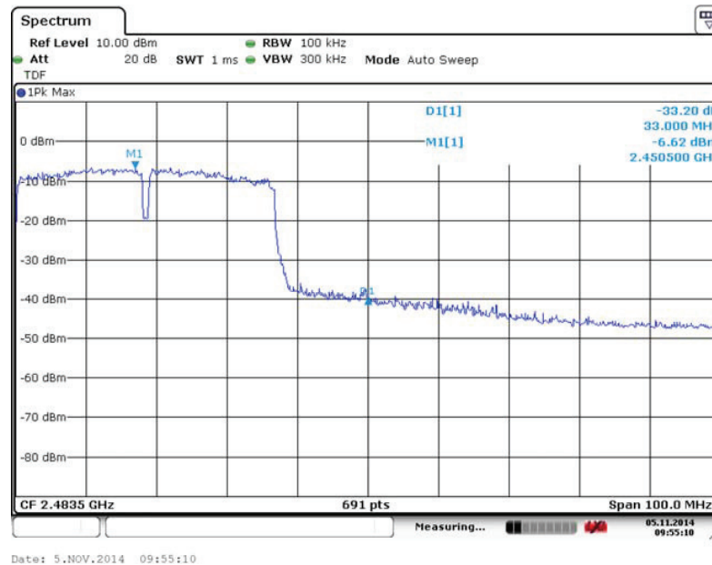
Fig. 116 Band Edges (802.11 n-40MHz, Ch 9)
