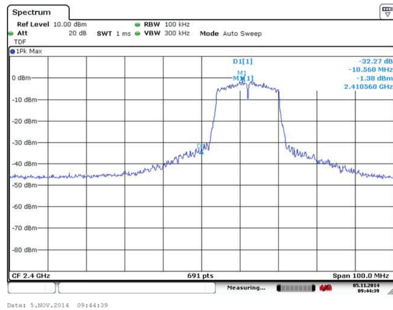
Fig. 111 Band Edges (802.11g, Ch 1)
