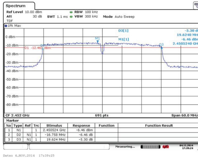
Fig. 108 Occupied 6dB Bandwidth (802.11n-40MHz, Ch 9)
