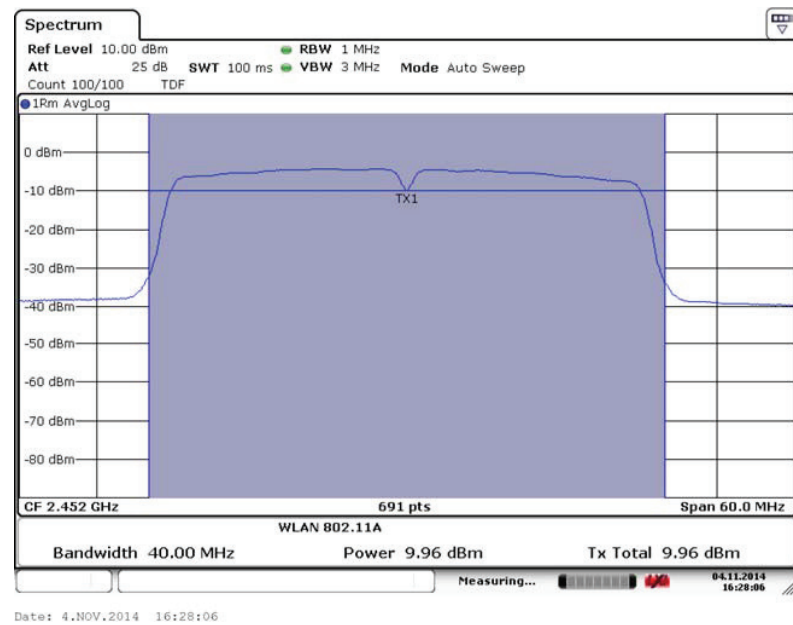
Fig. 78 Maximum Average Output Power (802.11n- 40MHz,Ch11,MCS5)
