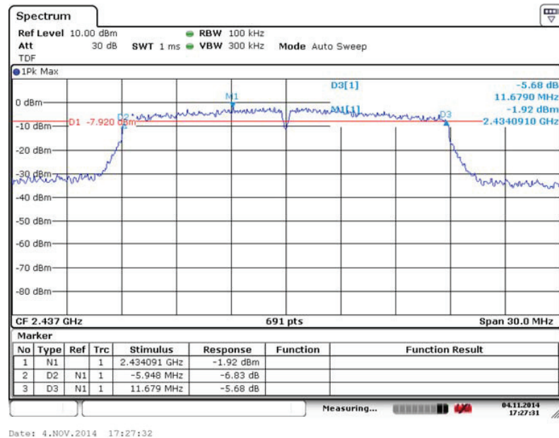
Fig. 104 Occupied 6dB Bandwidth (802.11 n-20MHz, Ch 6)
