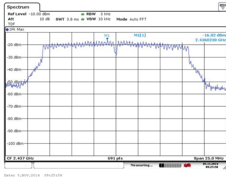
Fig. 89 Power Spectral Density (802.11g, Ch 6)
