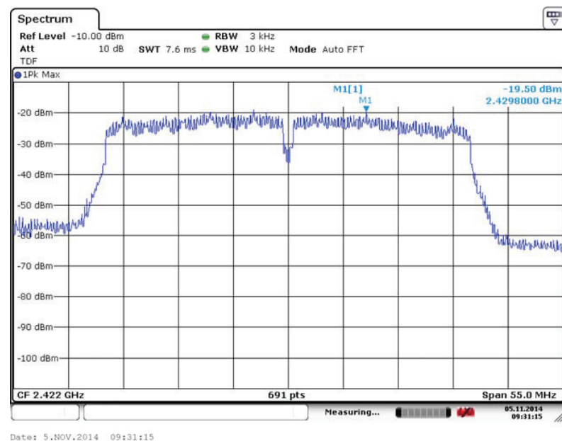
Fig. 94 Power Spectral Density (802.11n-40MHz, Ch 3)
