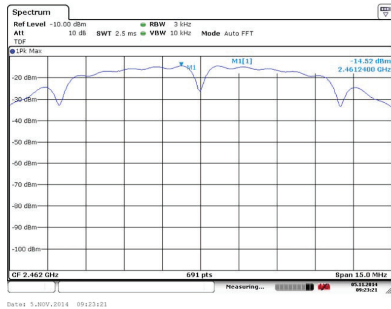
Fig. 87 Power Spectral Density (802.11b, Ch 11)
