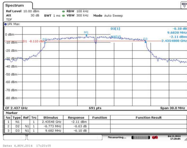
Fig. 101 Occupied 6dB Bandwidth (802.11g, Ch 6)
