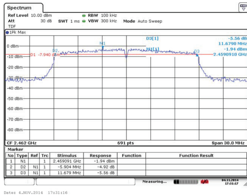
Fig. 105 Occupied 6dB Bandwidth (802.11n-20MHz, Ch 11)
