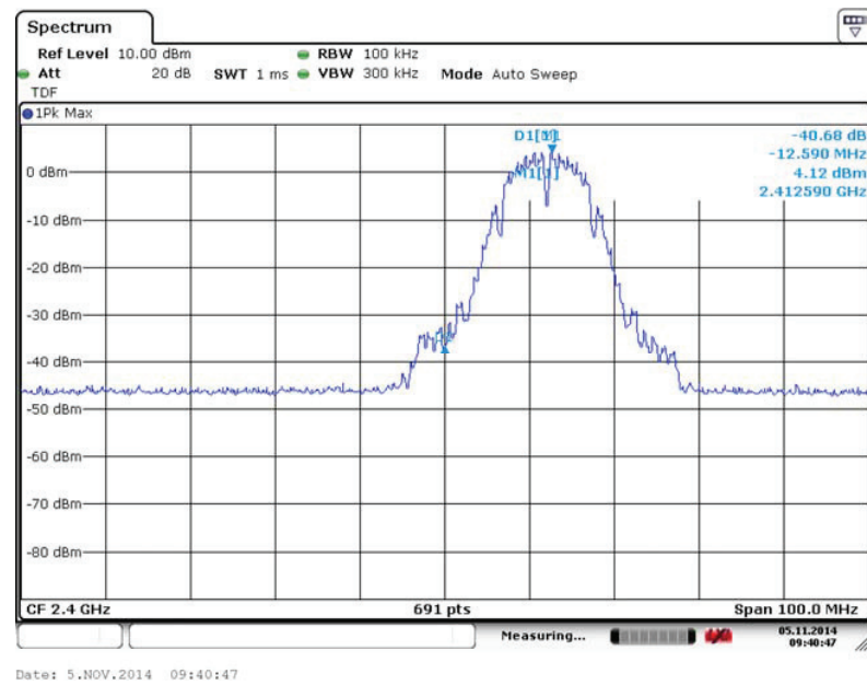
Fig. 109 Band Edges (802.11b, Ch 1)
