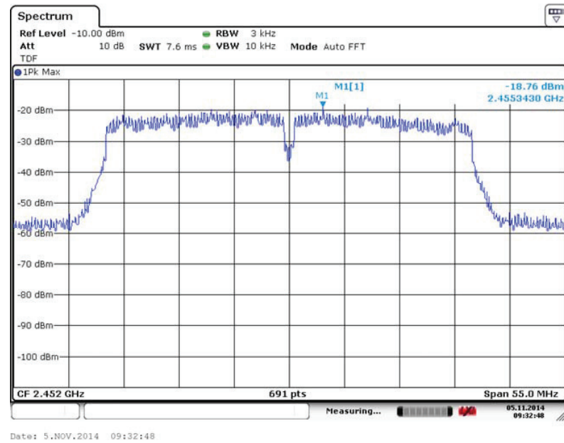
Fig. 96 Power Spectral Density (802.11n-40MHz, Ch 9)
