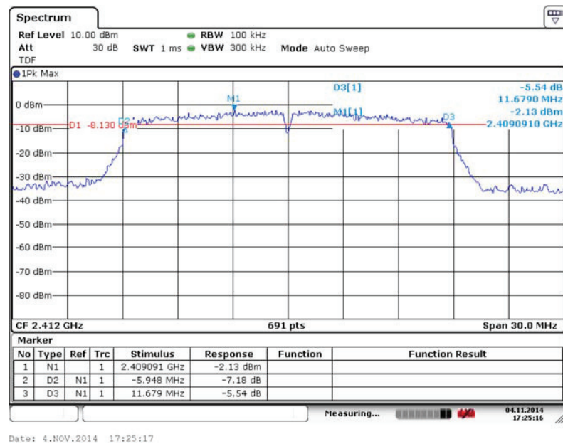
Fig. 103 Occupied 6dB Bandwidth (802.11 n-20MHz, Ch 1)
