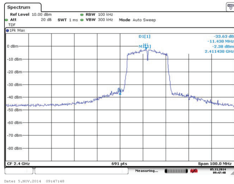
Fig. 113 Band Edges (802.11 n-20MHz, Ch 1)
