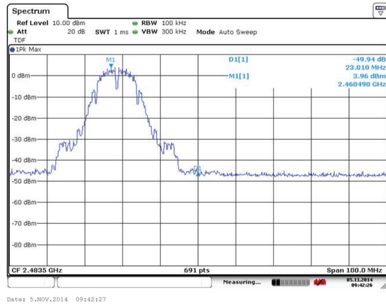
Fig. 110 Band Edges (802.11b, Ch 11)
