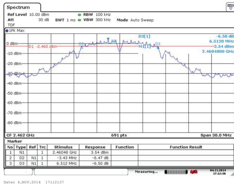
Fig. 99 Occupied 6dB Bandwidth (802.11b, Ch 11)
