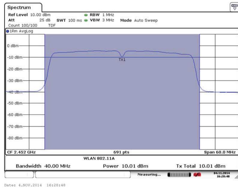
Fig. 81 Maximum Average Output Power (802.11n- 40MHz,Ch11,MCS6)
