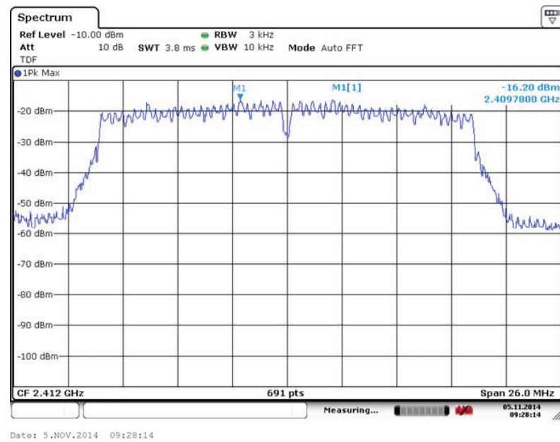
Fig. 91 Power Spectral Density (802.11n-20MHz, Ch 1)
