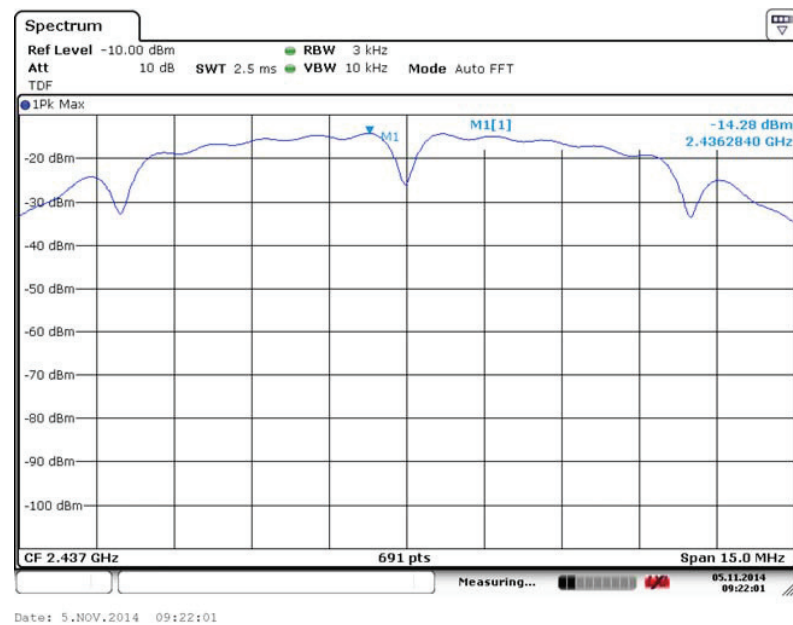
Fig. 86 Power Spectral Density (802.11b, Ch 6)
