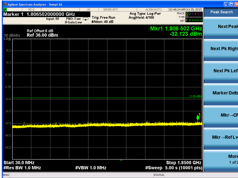
Channel 661, 30MHz~1850MHz
