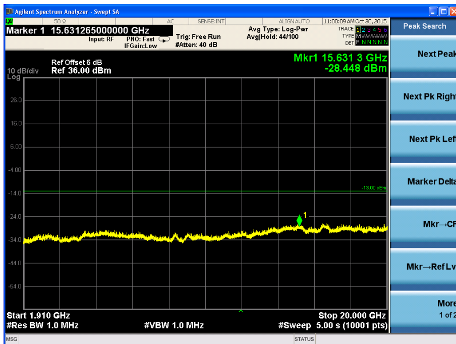
Channel 661, 1910MHz~20GHz
