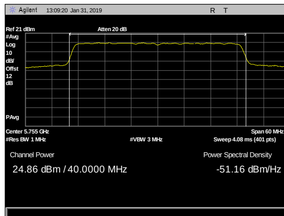
Plot 5. Output Power, 2dBi & 5dBi- 2x2, 5755MHz, c2
