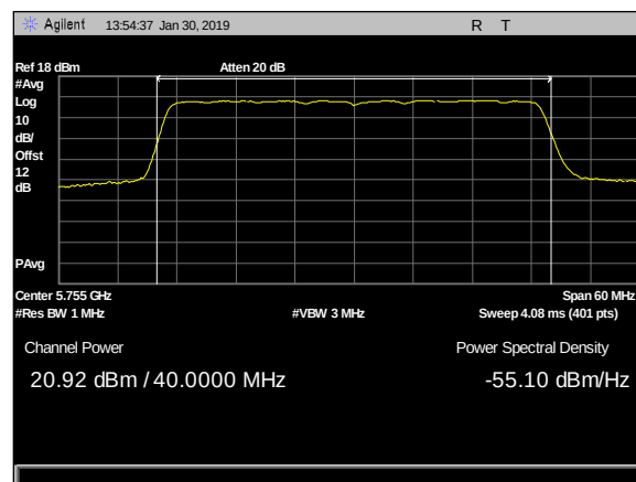
Plot 11. Output Power, 2dBi &amp; 5dBi 4x4, 5755MHz, c4
