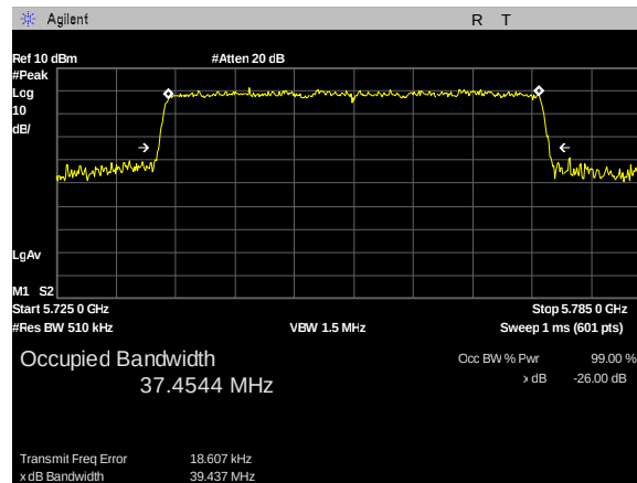
Plot 1. 26 dB Occupied Bandwidth, 40M, 5755 MHz
