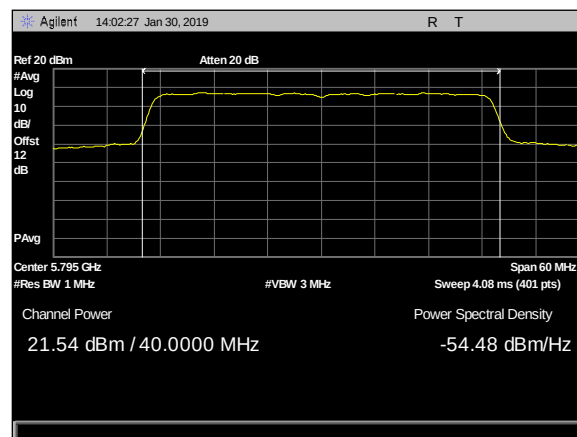
Plot 12. Output Power, 2dBi &amp; 5dBi 4x4, 5795MHz, c1
