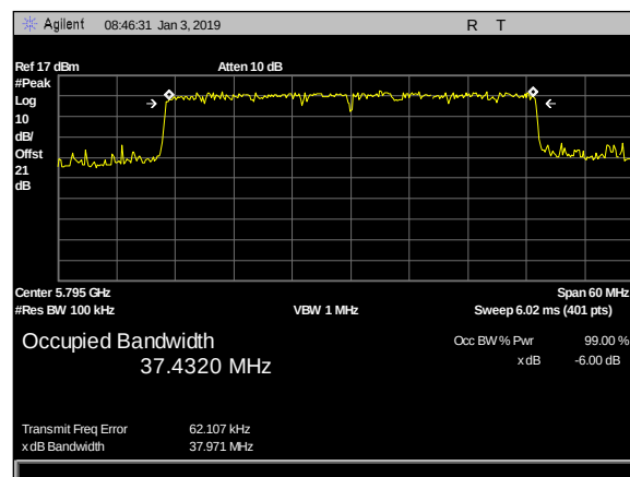
Plot 63. 6 dB Occupied Bandwidth, 40M, 5795 MHz
