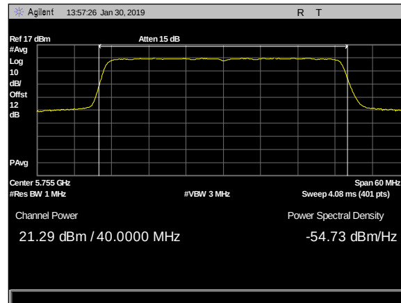
Plot 10. Output Power, 2dBi &amp; 5dBi 4x4, 5755MHz, c3
