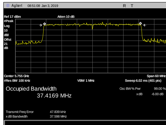
Plot 62. 6 dB Occupied Bandwidth, 40M, 5755 MHz
