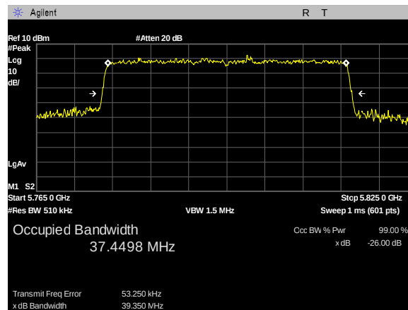
Plot 2. 26 dB Occupied Bandwidth, 40M, 5795 MHz
