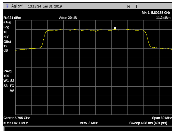
Plot 17. Power Spectral Density, 2dBi & 5dBi- 2x2, 5795MHz, c1
