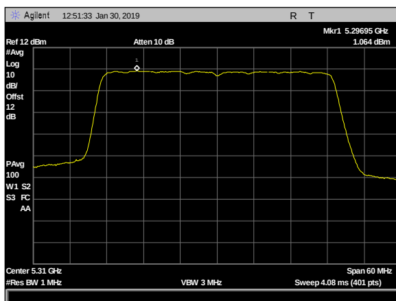
Plot 127. Power Spectral Density, 2dBi & 5dBi, 4x4, 5310MHz c4
