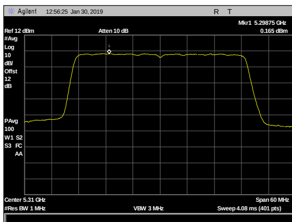
Plot 124. Power Spectral Density, 2dBi & 5dBi, 4x4, 5310MHz c1
