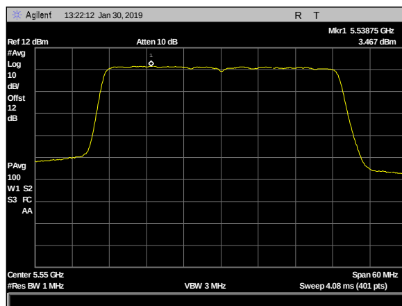
Plot 135. Power Spectral Density, 2dBi & 5dBi, 4x4, 5550MHz c4
