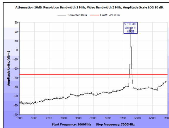
Plot 208. Radiated Emissions, -27dBm, 4x4, 5dBi, 5510, 1-7GHz
