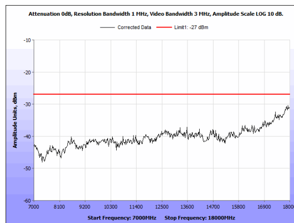
Plot 209. Radiated Emissions, -27dBm, 4x4, 5dBi, 5510, 7-18GHz
