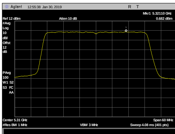
Plot 125. Power Spectral Density, 2dBi & 5dBi, 4x4, 5310MHz c2
