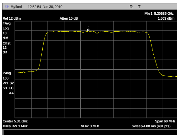
Plot 126. Power Spectral Density, 2dBi & 5dBi, 4x4, 5310MHz c3
