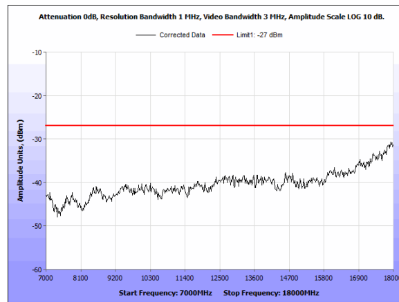
Plot 207. Radiated Emissions, -27dBm, 4x4, 5dBi, 5310, 7-18GHz
