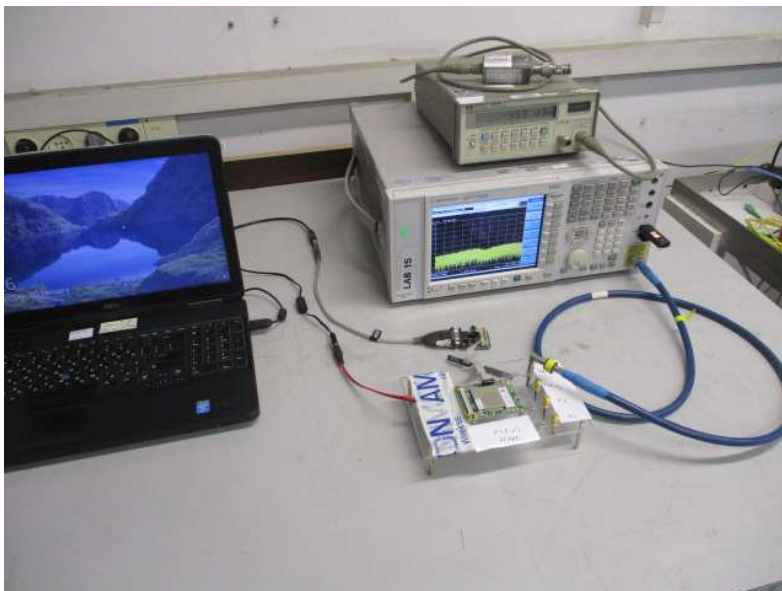
Figure 2. Conducted Emission Test (with Spectrum Analyzer)
