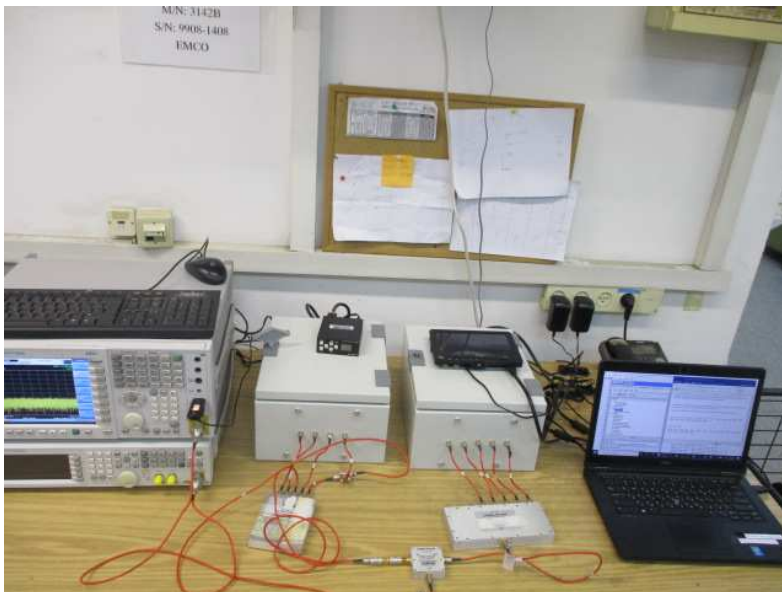
Figure 4. Contention Based Protocol Test
