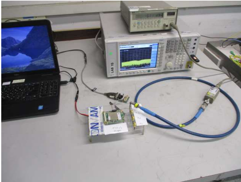
Figure 3. Conducted Emission Test (with Power Sensor)
