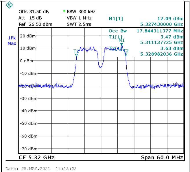
Figure 120. 5320.0MHz, 20MHz BW
