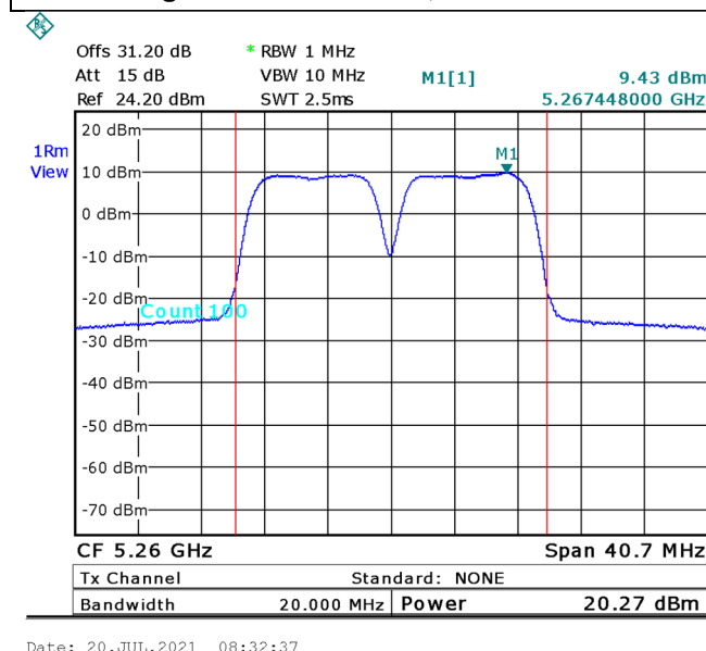
Figure 14. 5260.0MHz, 20MHz BW
