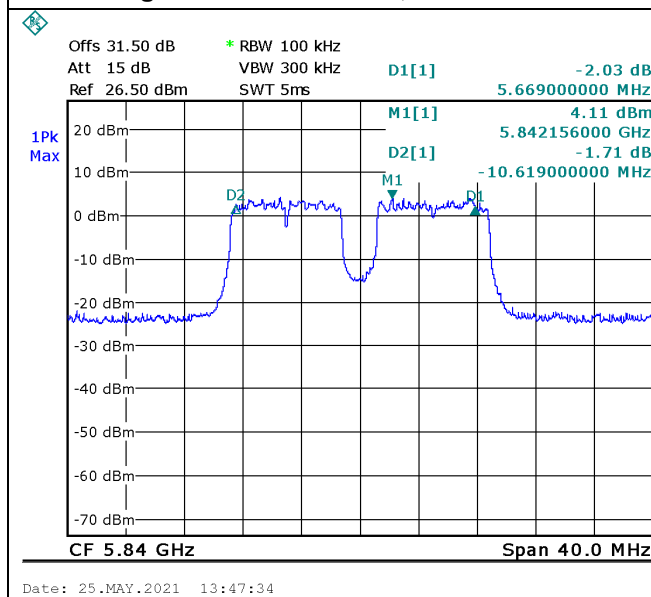
Figure 145. 5840.0MHz, 20MHz BW
