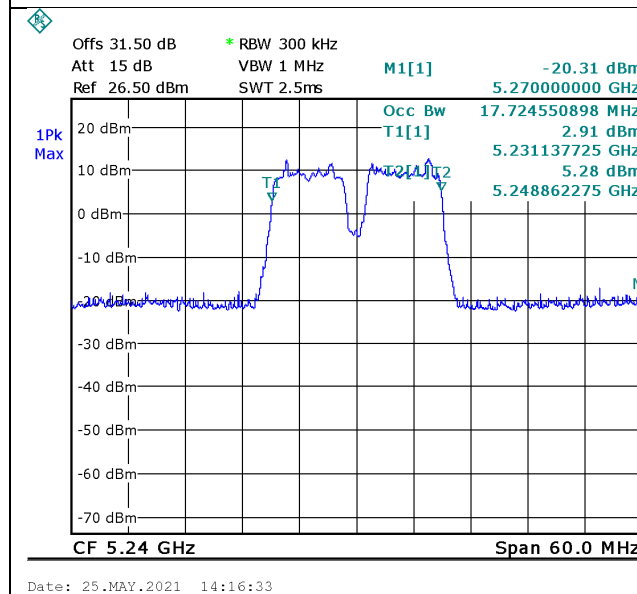
Figure 117. 5240.0MHz, 20MHz BW
