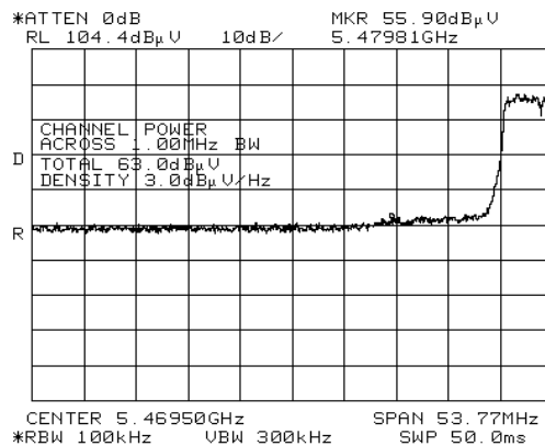
Figure 100: UNII 2C, 5.4695GHz, Rest. Band Peak [Vertical]
