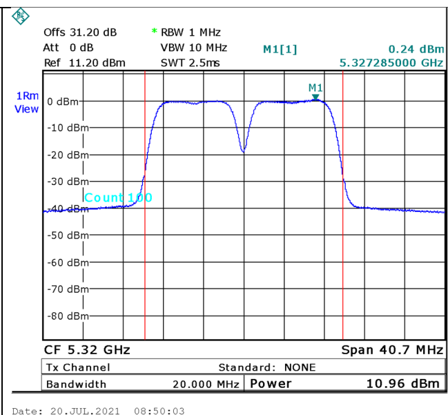
Figure 63. 5320.0MHz, 20MHz BW
