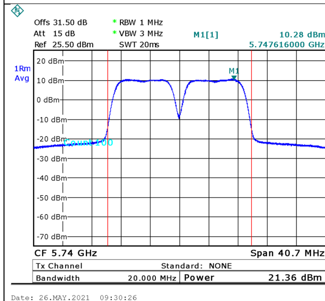
Figure 68. 5740.0MHz, 20MHz BW
