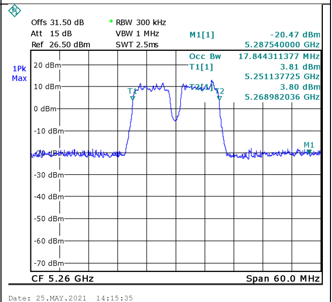
Figure 118. 5260.0MHz, 20MHz BW
