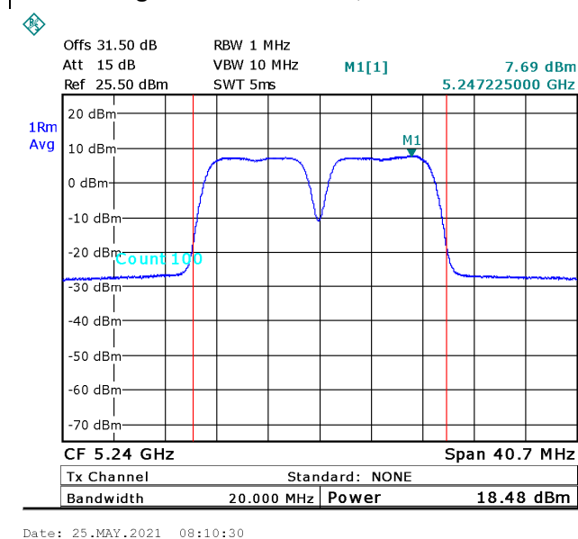
Figure 13. 5240.0MHz, 20MHz BW
