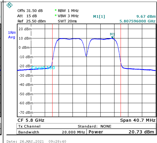
Figure 69. 5800.0MHz, 20MHz BW
