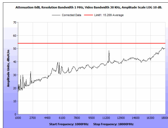
Plot 22. Unwanted Emissions, 2 dBi, Average, CF 5755 MHz, 1 – 18 GHz
