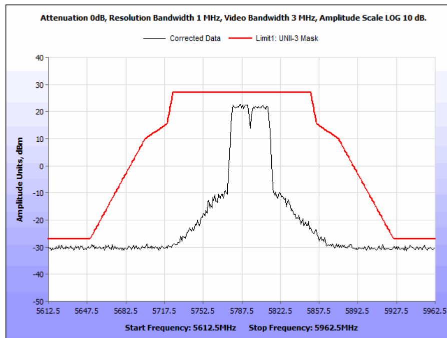
Plot 16. Radiated Band Edge, 5725 – 5850 MHz, BW 40, 5795 MHz, rx 11 dBi
