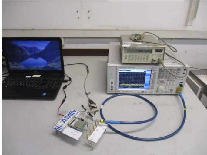
Figure 1: Conducted Emission Setup
