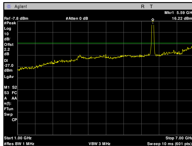
Plot 71. Radiated Spurious Emissions, 5590 MHz, 40 MHz, 1 GHz – 7 GHz
