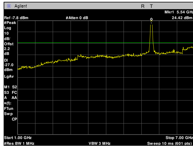
Plot 67. Radiated Spurious Emissions, 5540 MHz, 20 MHz, 1 GHz – 7 GHz
