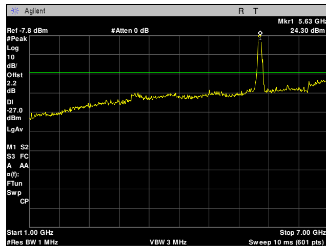
Plot 68. Radiated Spurious Emissions, 5620 MHz, 20 MHz, 1 GHz – 7 GHz
