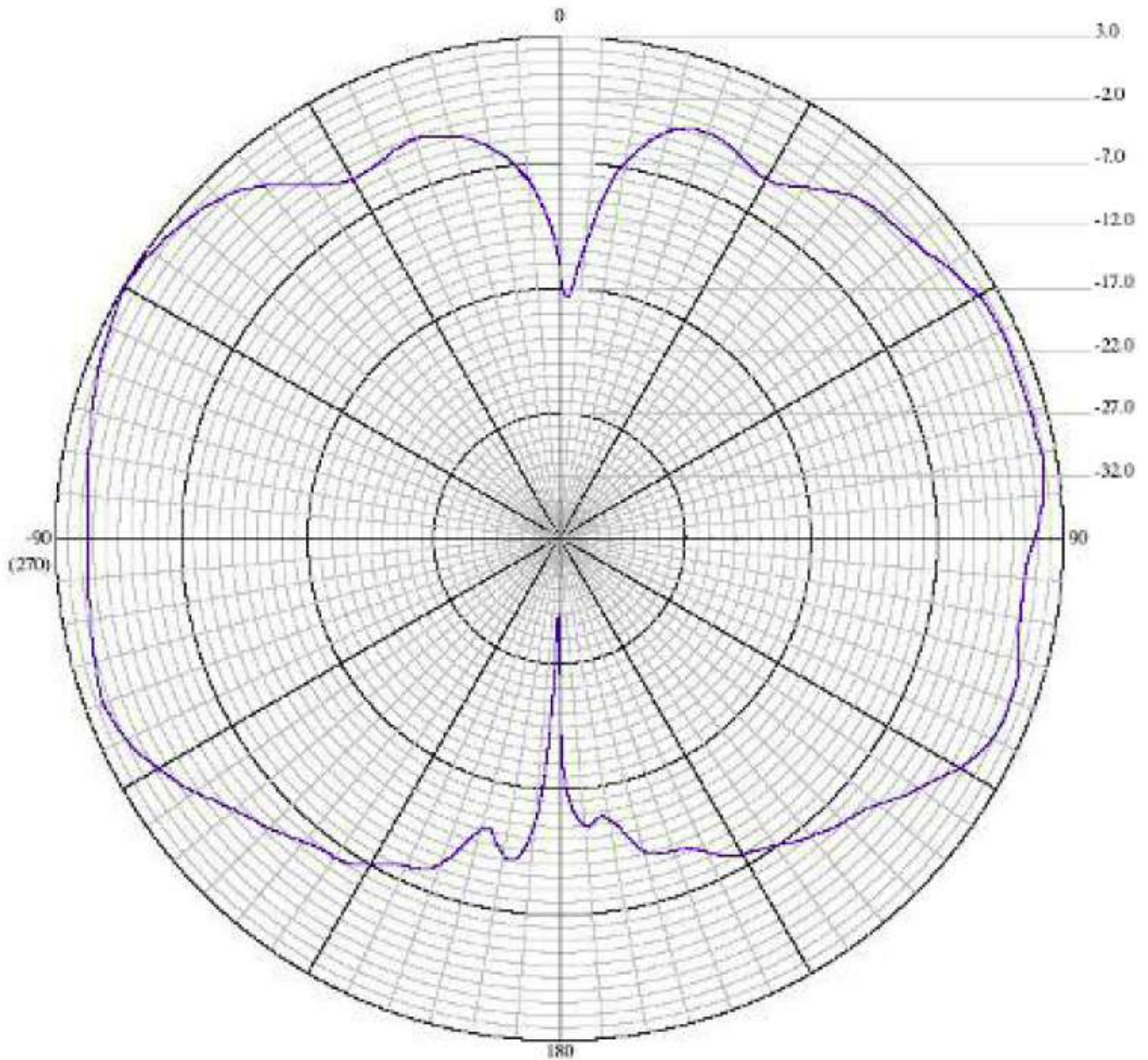
Elevation Pattern 2450MHz
