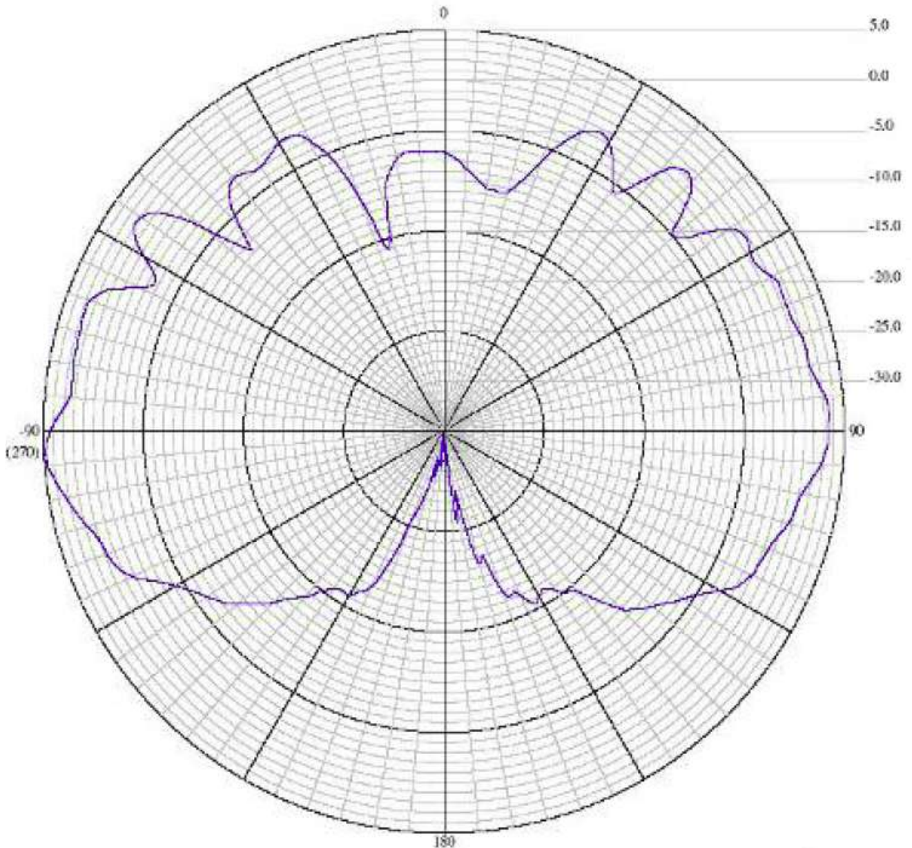
Elevation Pattern 5725MHz
