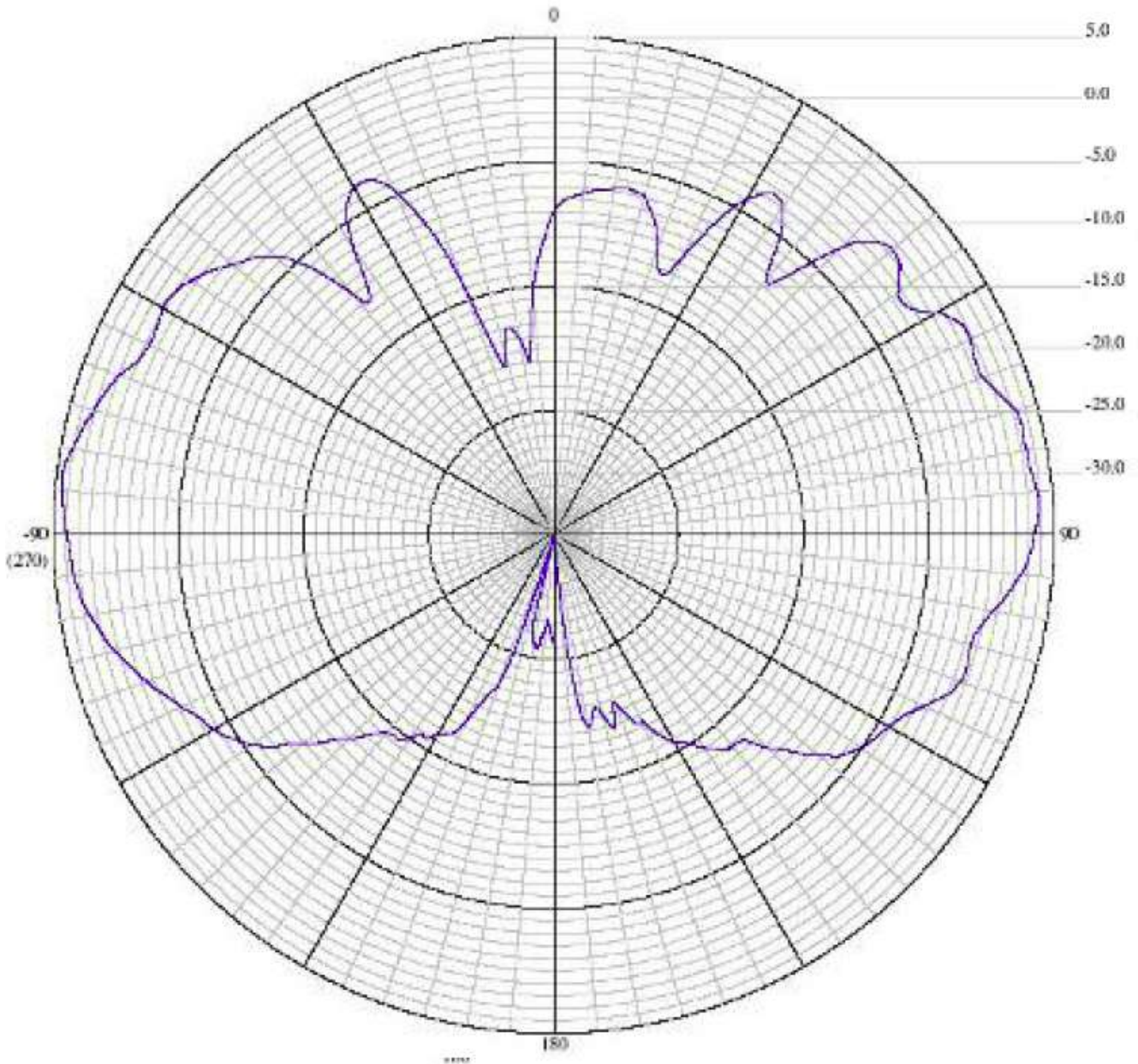
Elevation Pattern 5150MHz
