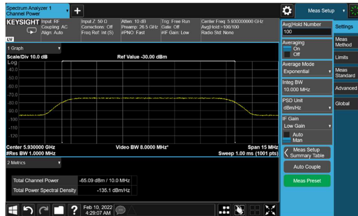
Figure 69. AWGN signal at 5930MHz
