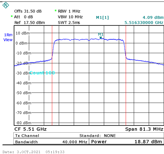
Figure 57. 5510.0MHz, 40MHz BW, port 1
