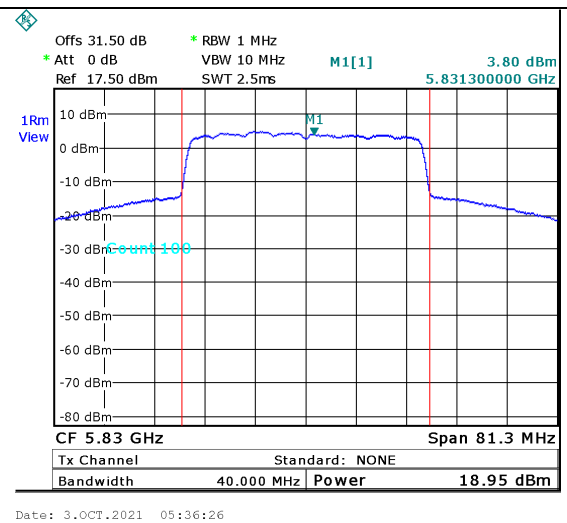
Figure 68. 5830.0MHz, 40MHz BW, port 2
