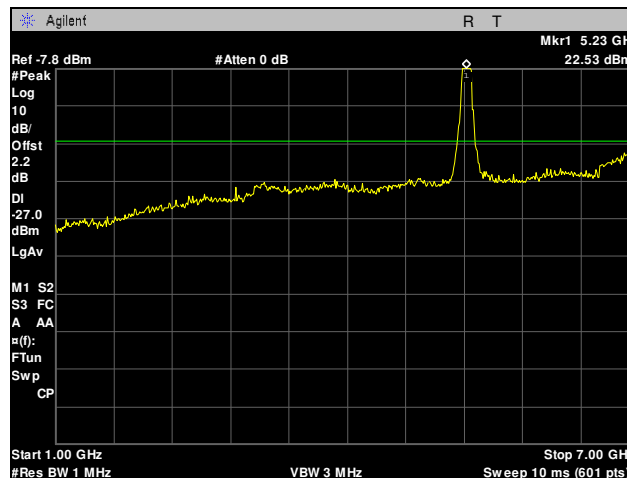
Plot 49. Radiated Spurious Emissions, High Channel, 40 MHz, 1 GHz – 7 GHz
