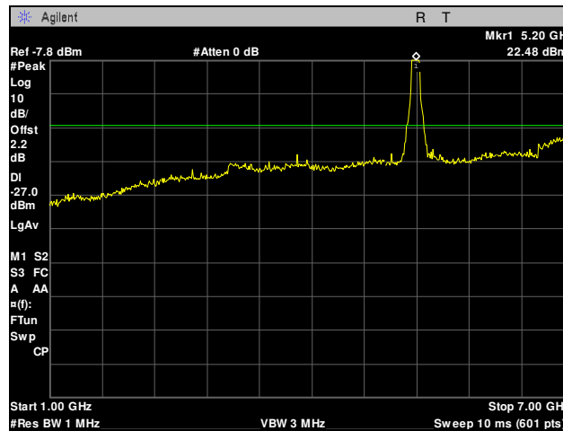
Plot 48. Radiated Spurious Emissions, Low Channel, 40 MHz, 1 GHz – 7 GHz
