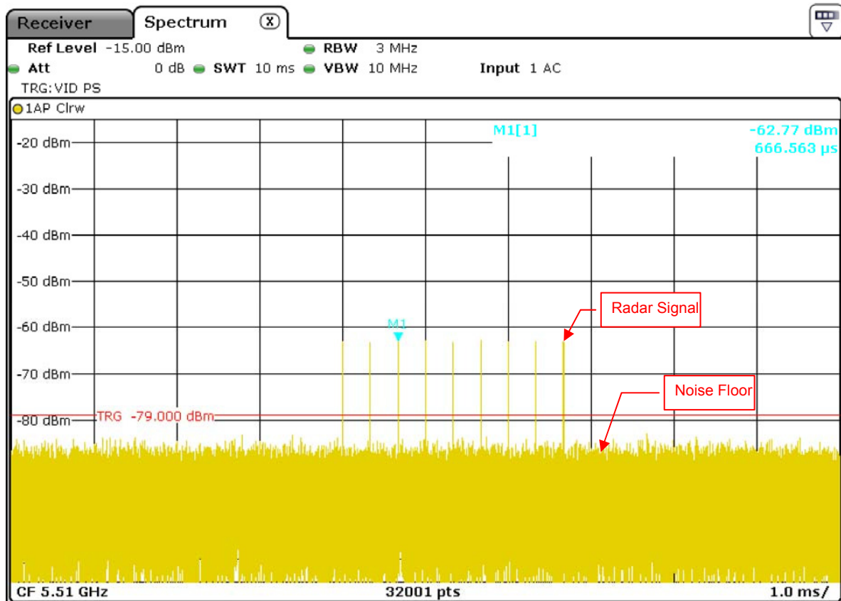
Radar Signal 6
