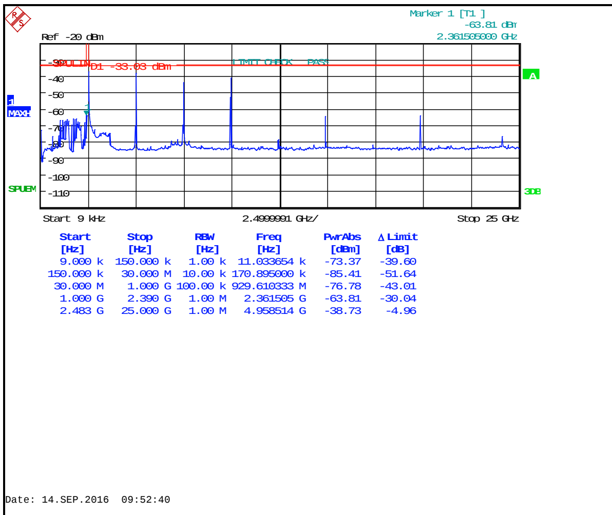
Plot 6-3: Antenna Conducted Spurious Emissions – 2480 MHz
