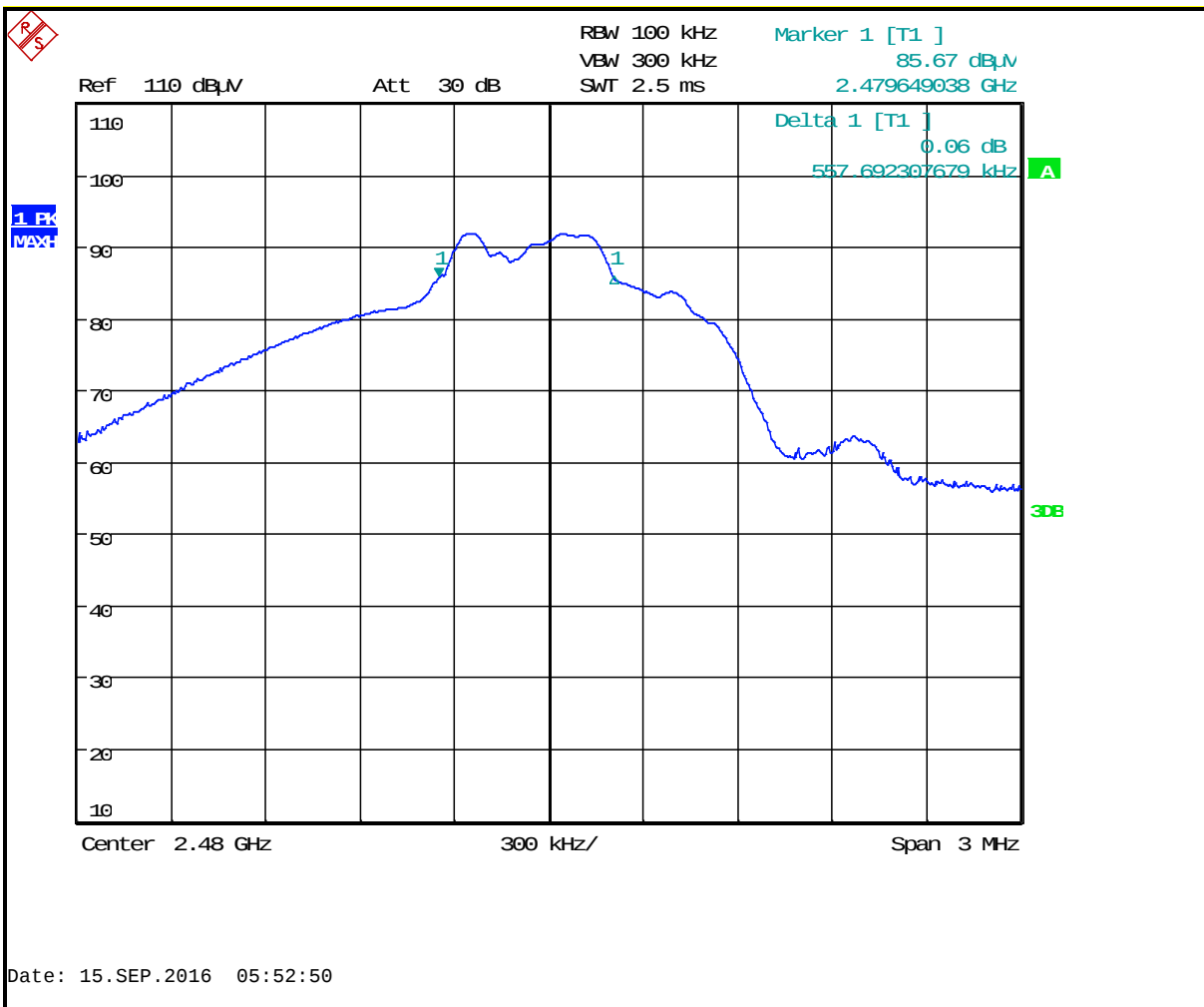
Plot 8-3: 6 dB Bandwidth – 2480 MHz
