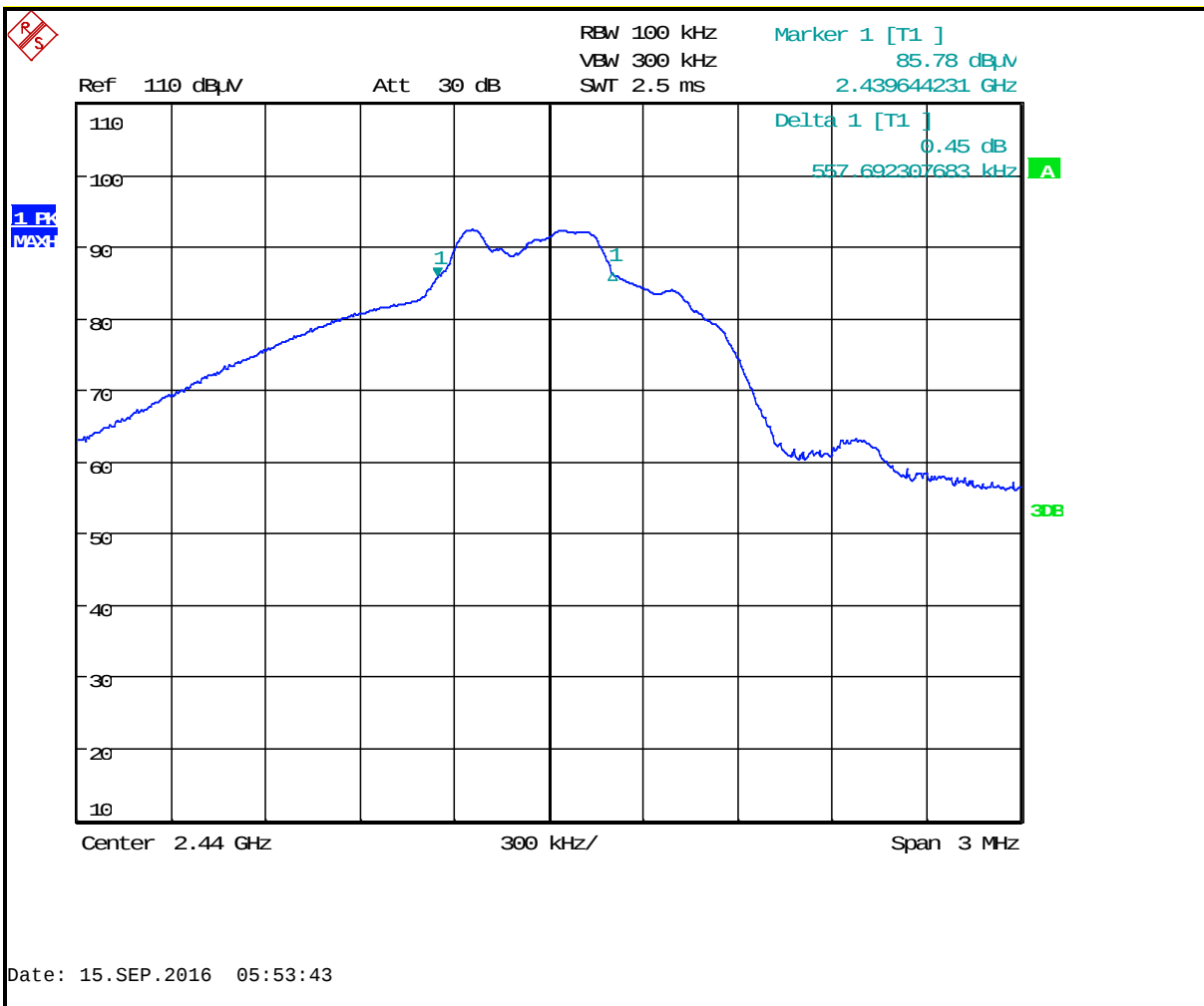
Plot 8-2: 6 dB Bandwidth – 2440 MHz
