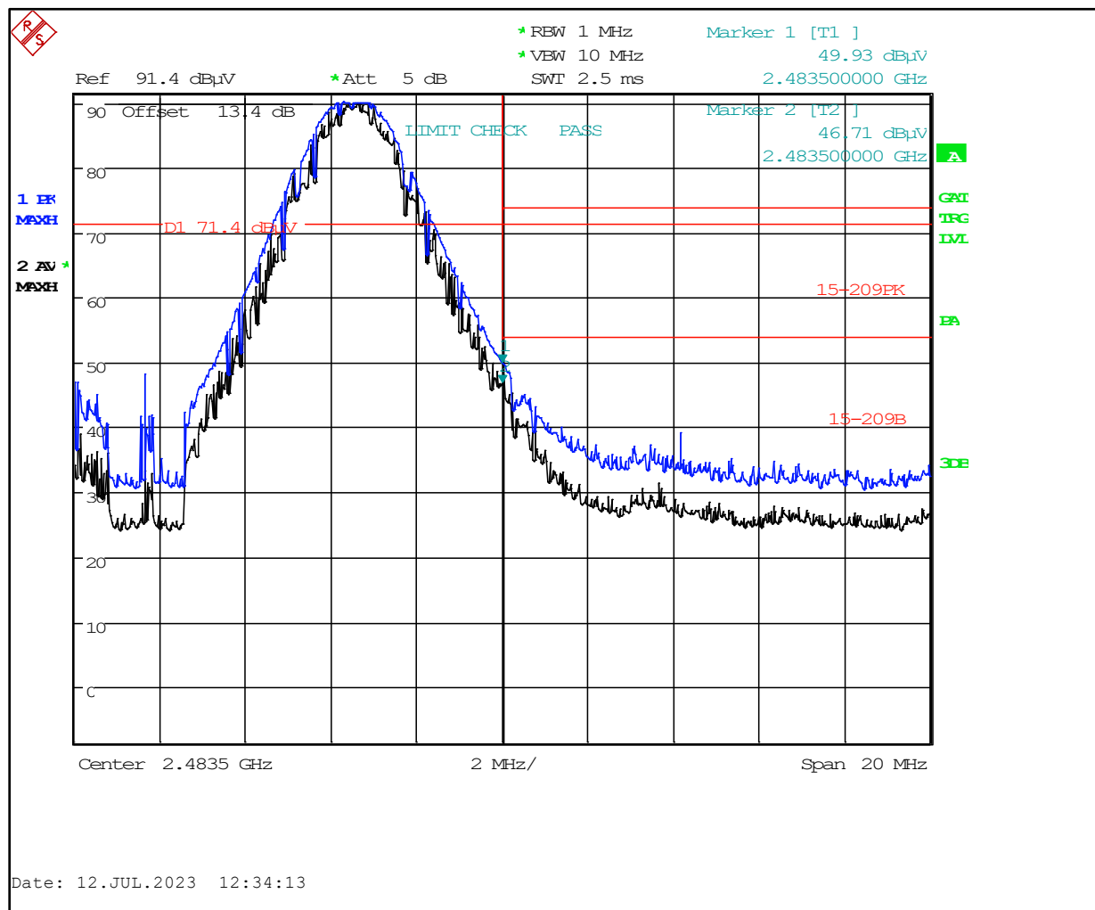
Plot 6-2: Upper Band Edge – Peak/Average
