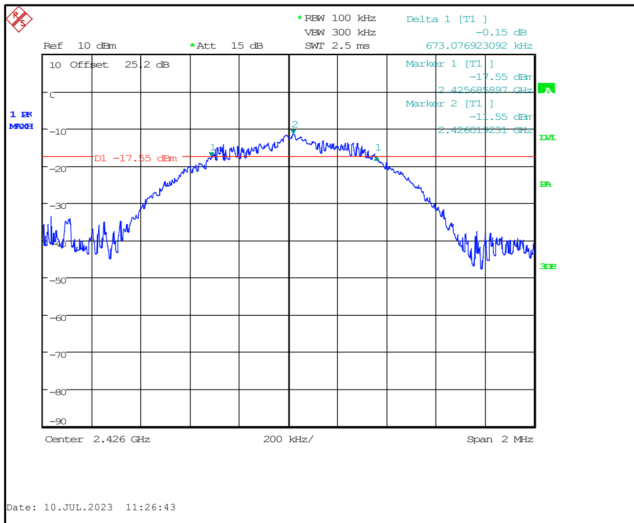
Plot 7-2: 6 dB Bandwidth – 2426 MHz
