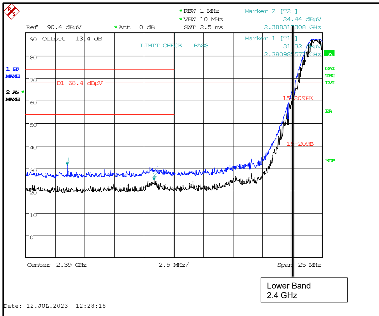
Plot 6-1: Lower Band Edge – Peak/Average
