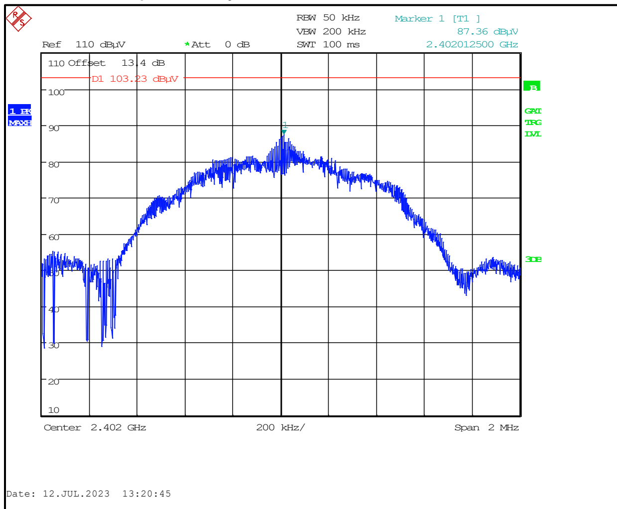
Plot 5-1: Peak Spectral Density – 2402 MHz
