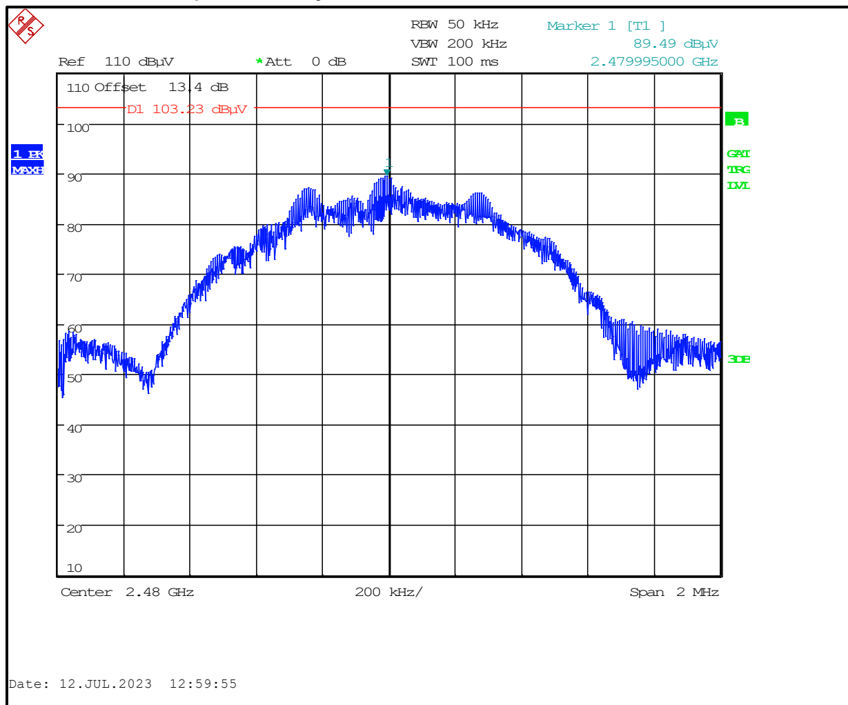
Plot 5-3: Peak Spectral Density – 2480 MHz
