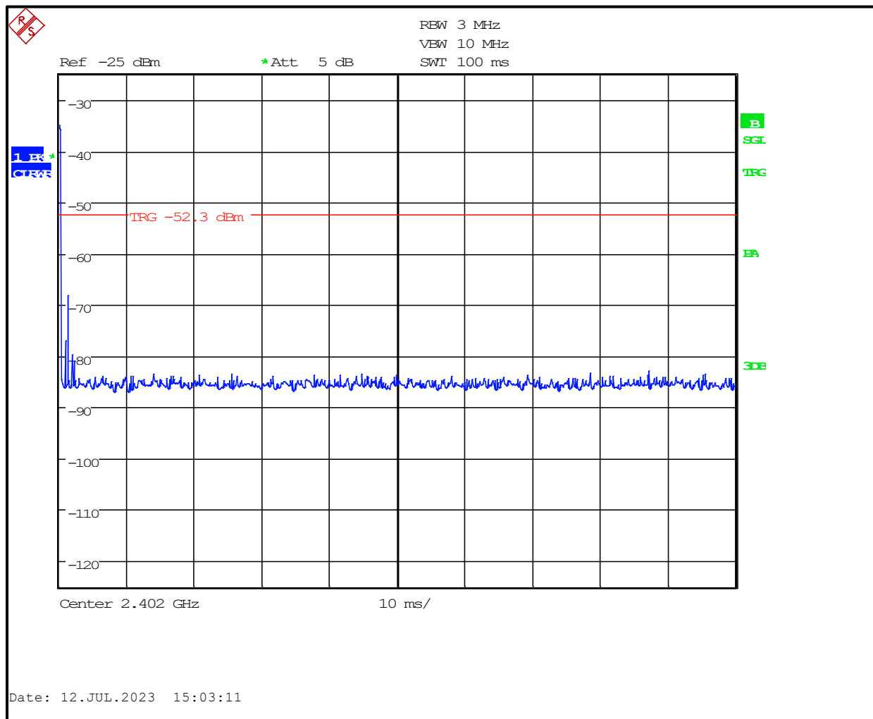
Plot 4-1: Duty Cycle (1 pulse in 100 ms)
