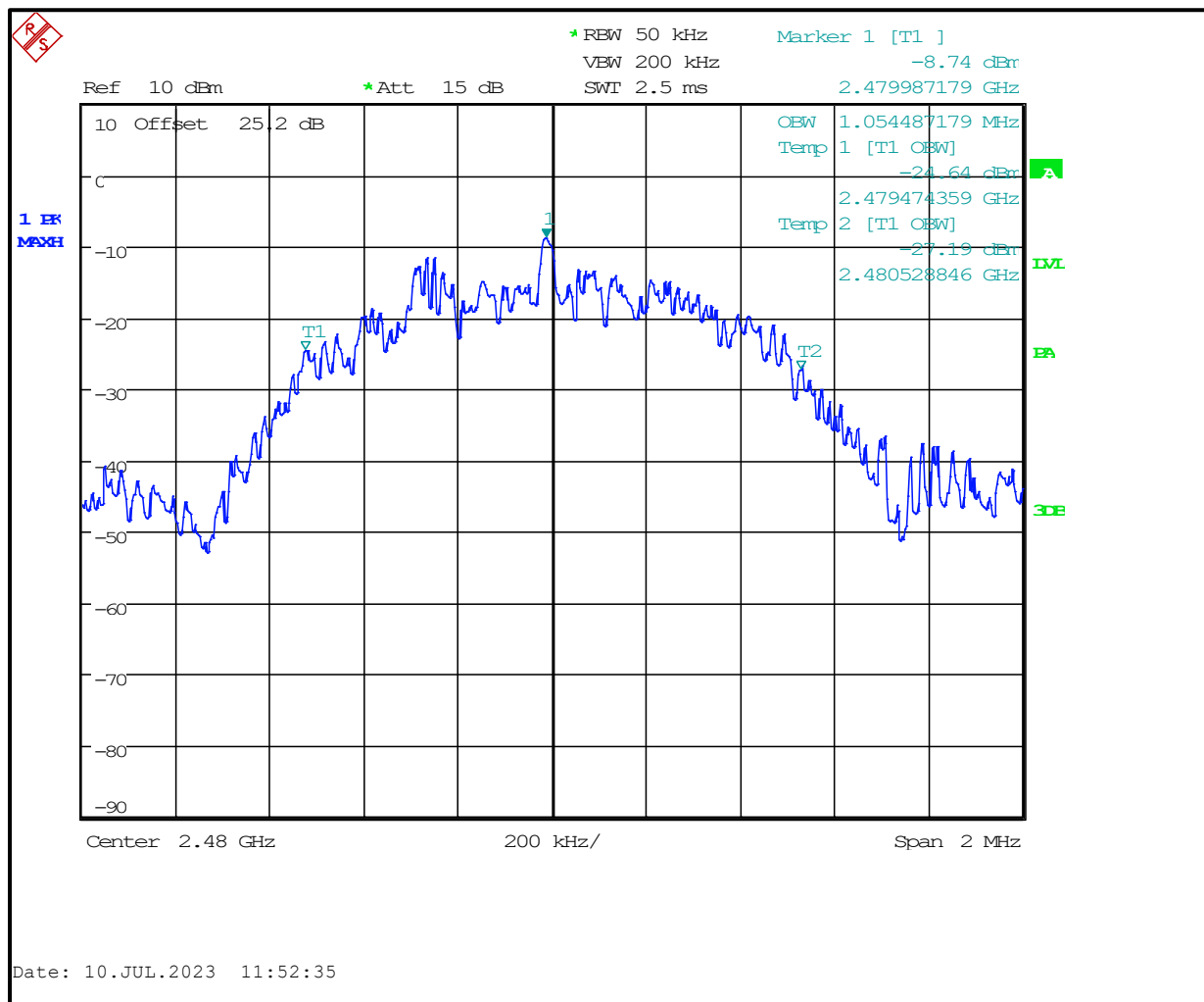
Plot 7-6: 99% Bandwidth – 2480 MHz
