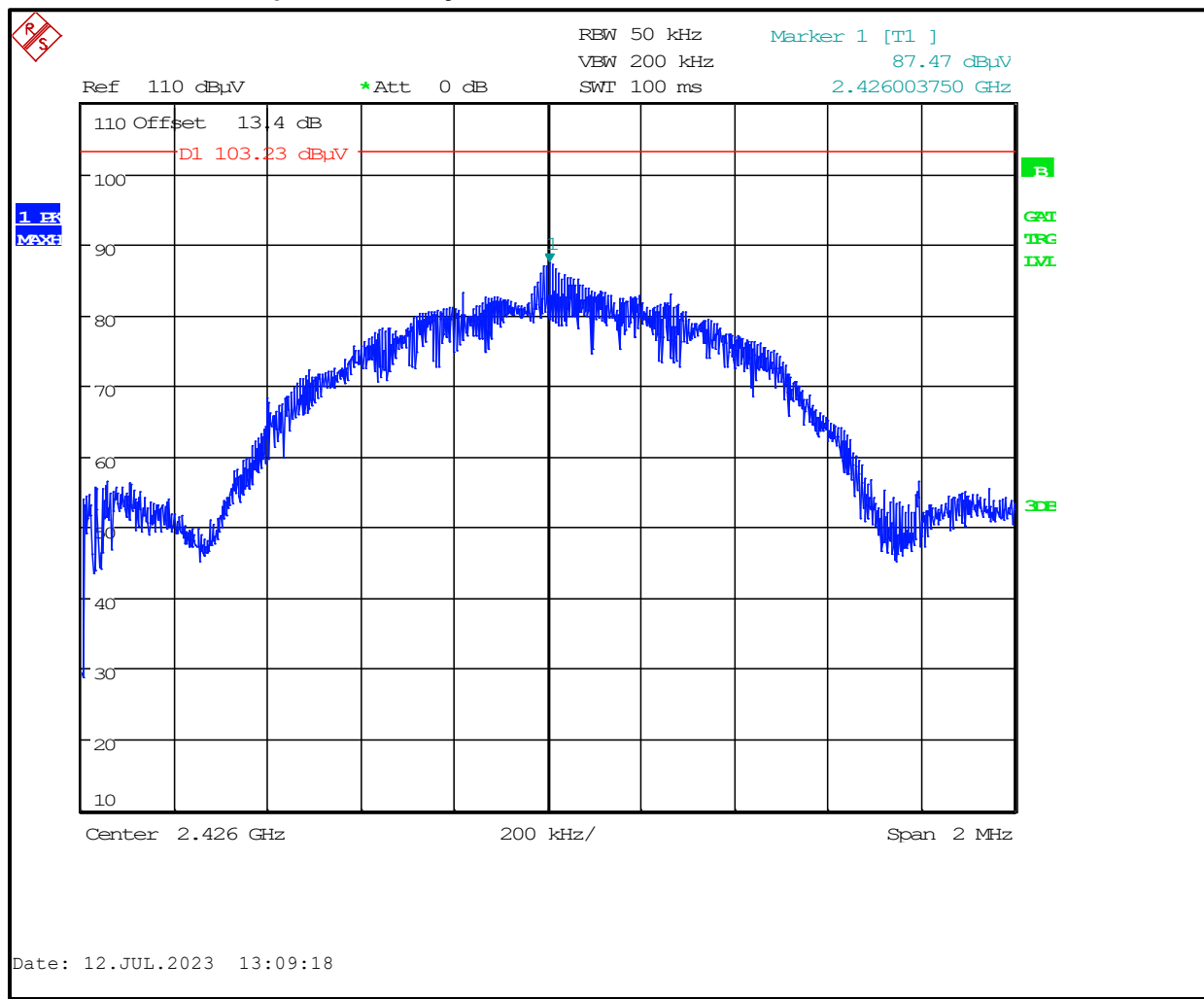
Plot 5-2: Peak Spectral Density – 2426 MHz
