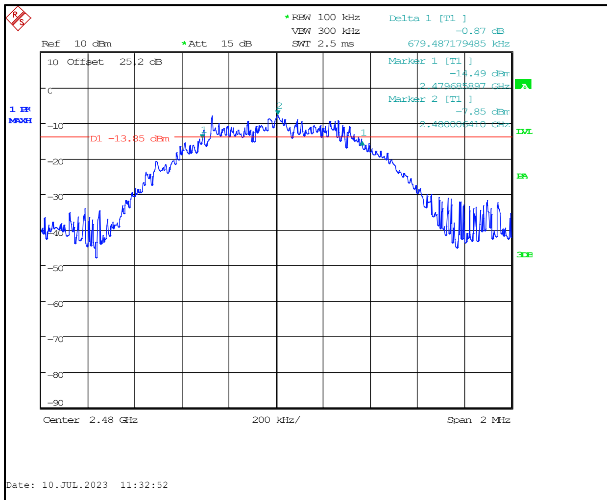
Plot 7-3: 6 dB Bandwidth – 2480 MHz
