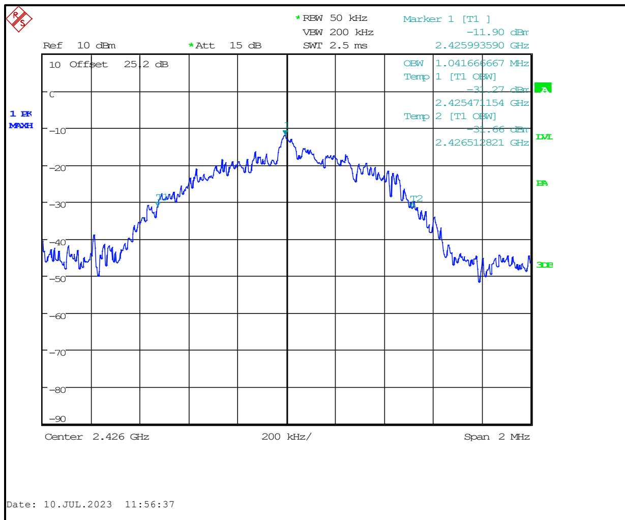
Plot 7-5: 99% Bandwidth – 2426 MHz
