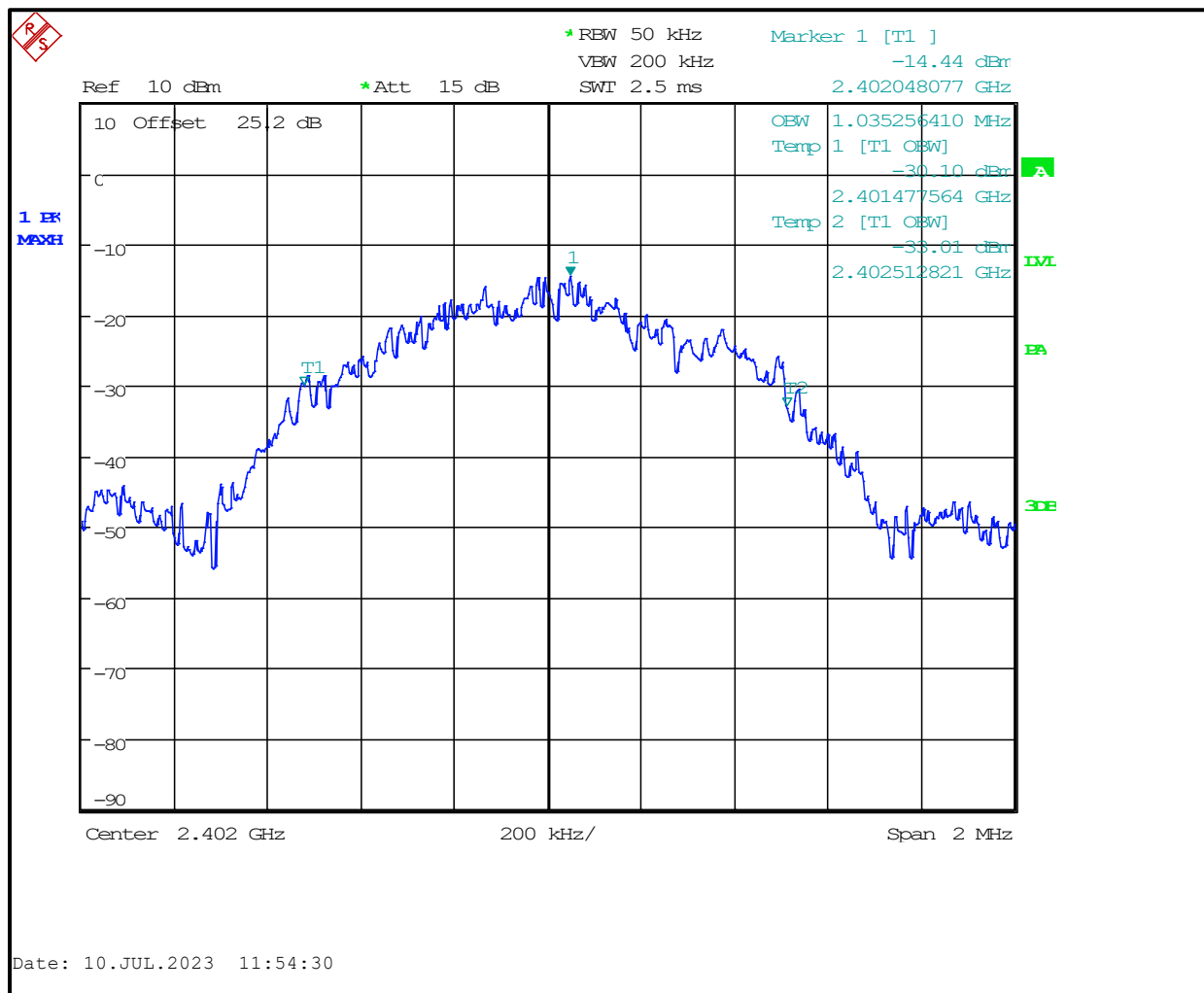
Plot 7-4: 99% Bandwidth – 2402 MHz
