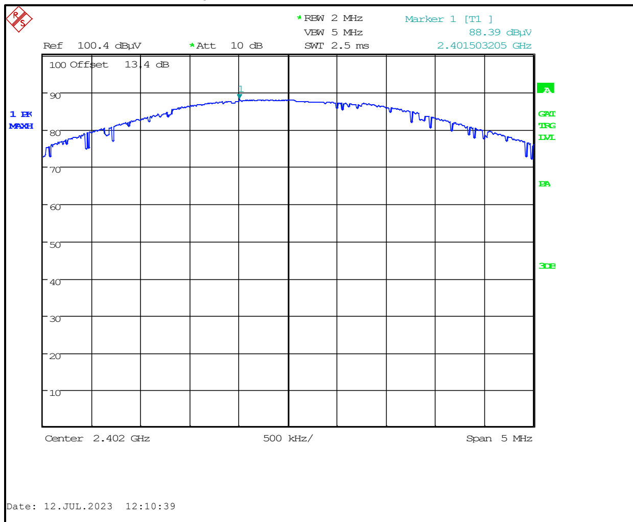
Plot 3-1: Peak Power Output - 2402 MHz
