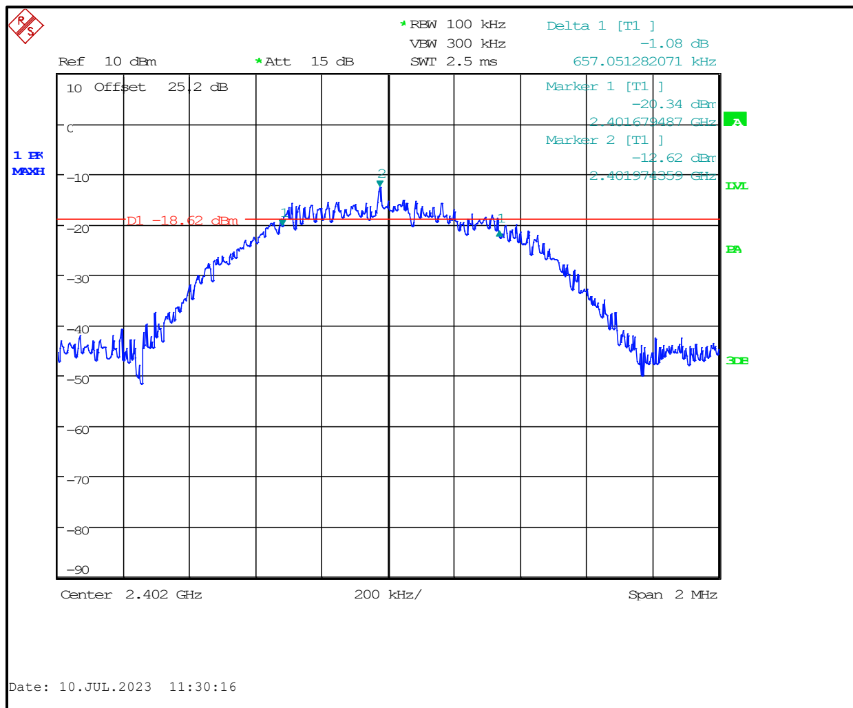
Plot 7-1: 6 dB Bandwidth – 2402 MHz
