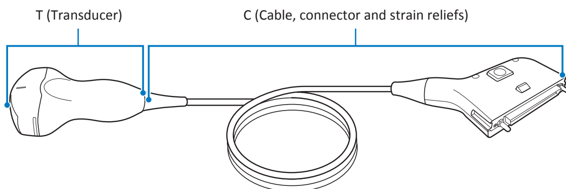
Figure 41 Transducer parts (Example transducer: C6-2)
