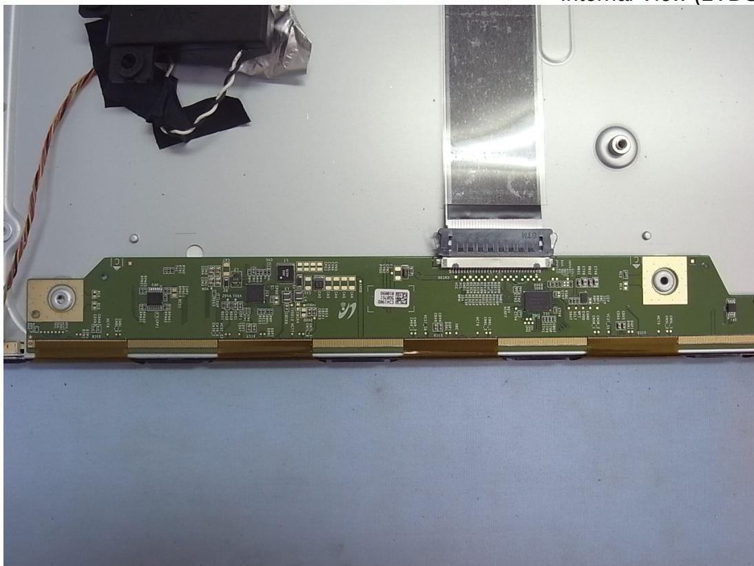
Figure 23 Internal View (LVDS Board)
