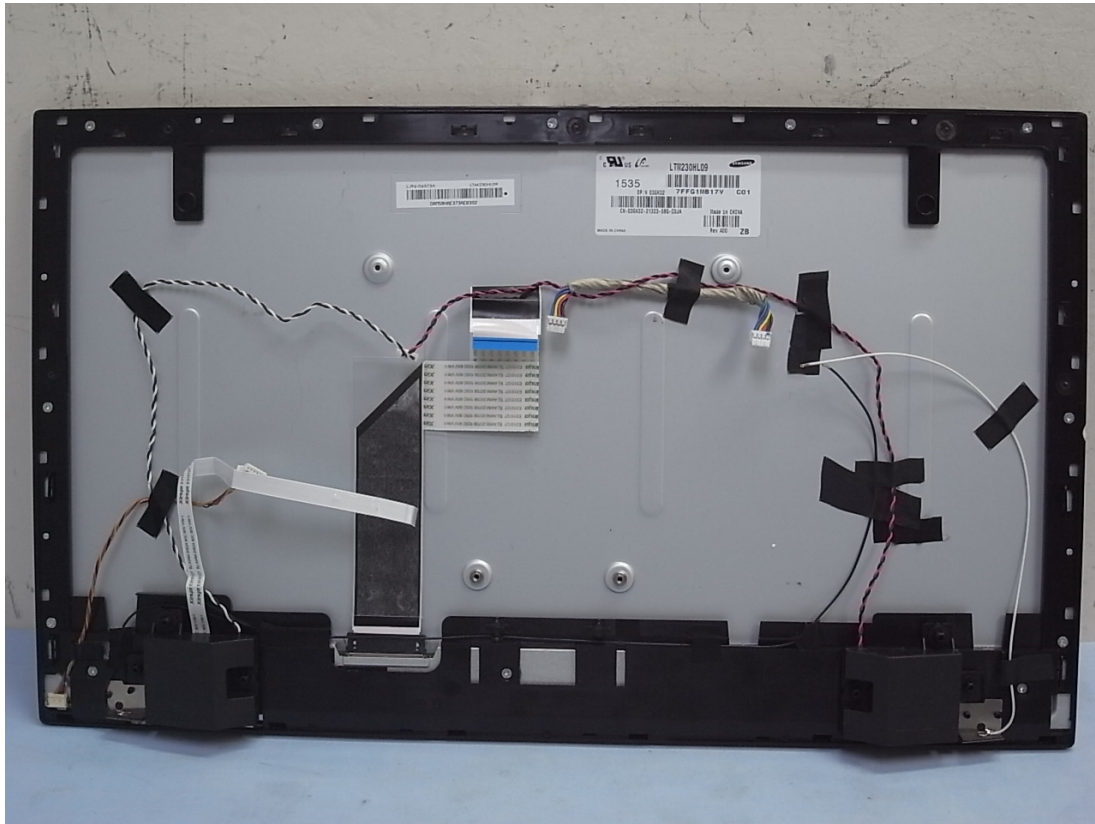
Figure 22 Internal View
