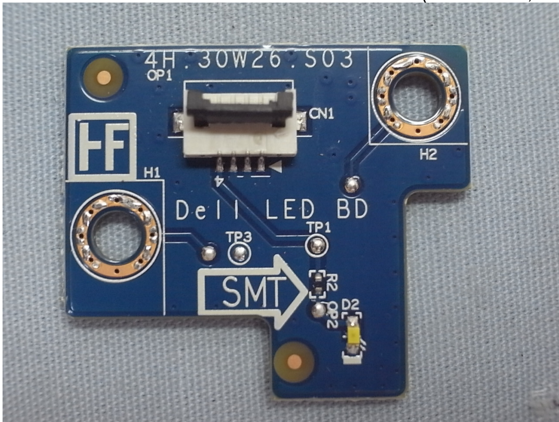
Figure 28 Internal View (Control Board, Front View)
