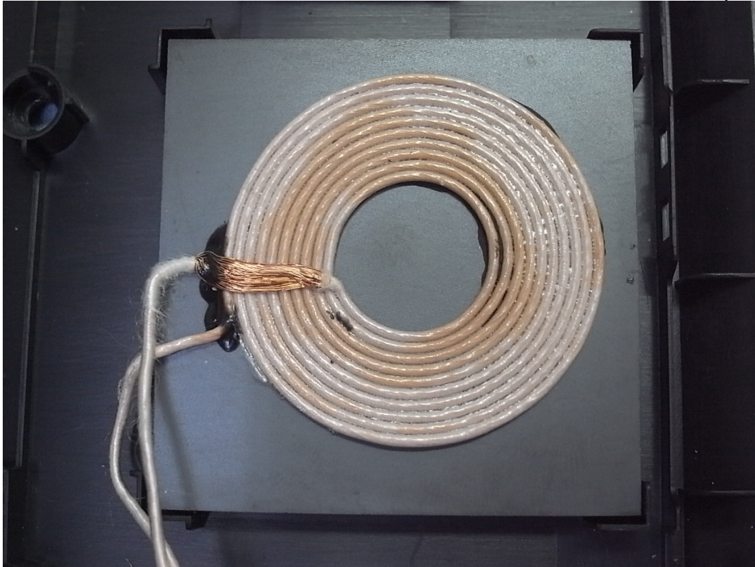
Figure 32 Internal View (Loop ANT)
