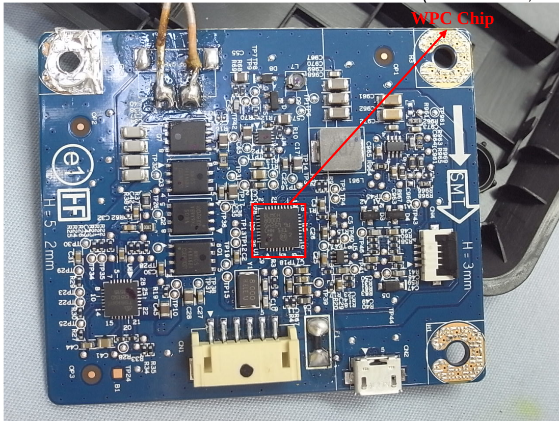
Figure 30 Internal View (Control Board, Front View)
