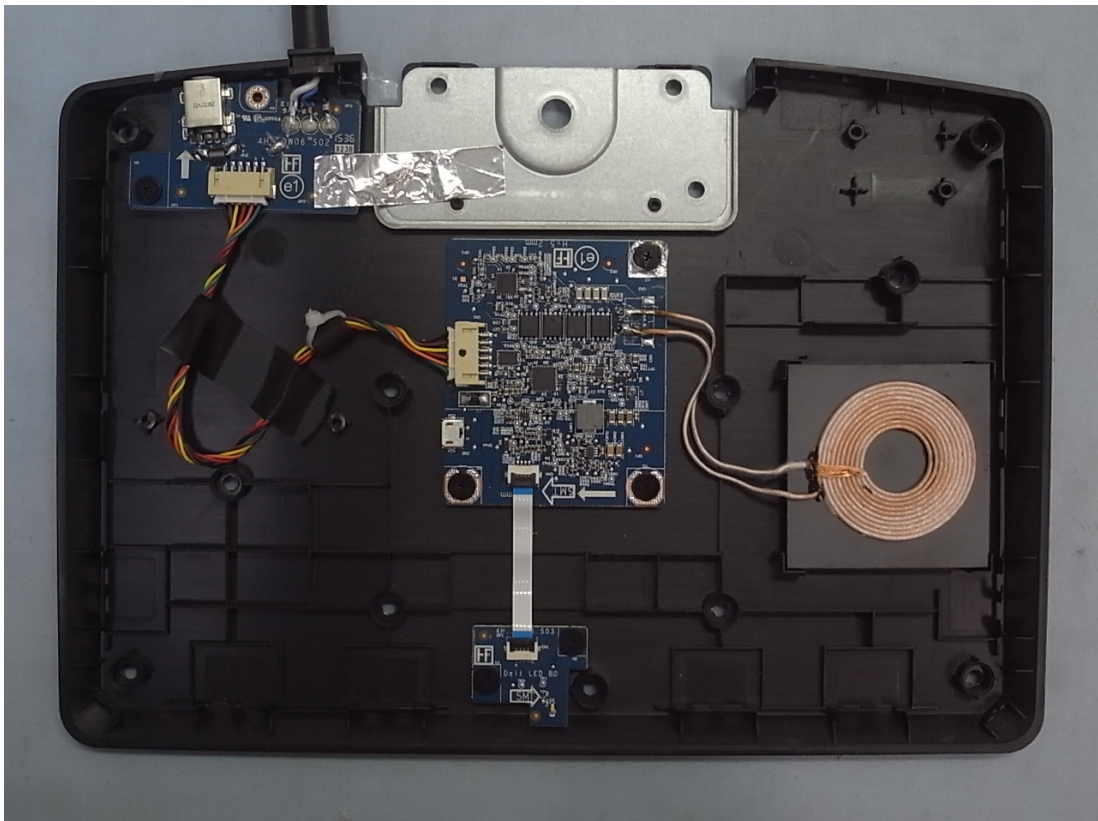
Figure 25 Internal View
