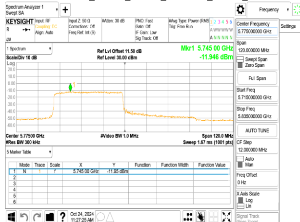
802.11ax_80MHz_Chain0_5775MHz_RU484_65
