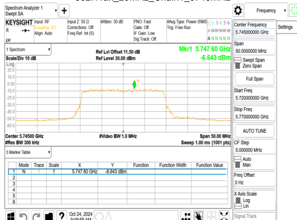
802.11ax_20MHz_Chain1_5745MHz_RU106_53
