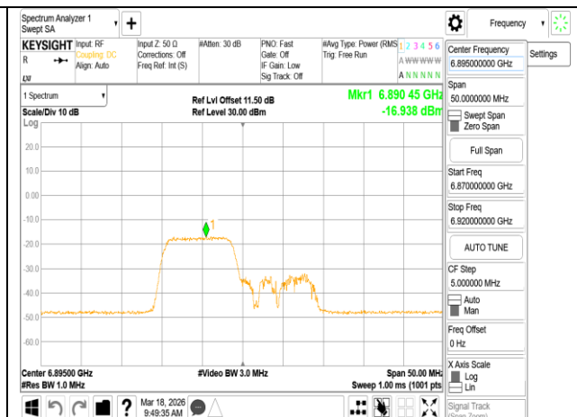
802.11ax_20MHz_Chain0_6895MHz_RU106_53
