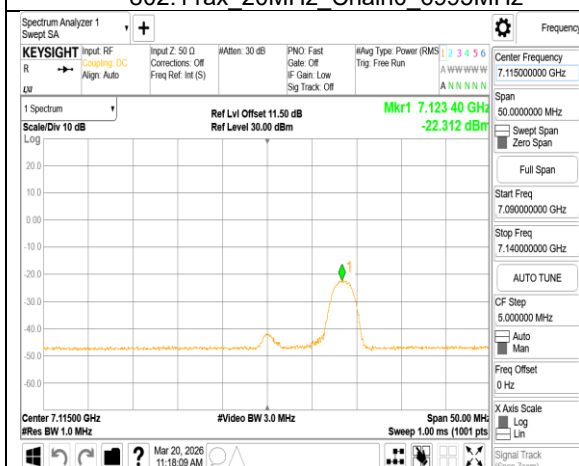
802.11ax_20MHz_Chain0_7115MHz_RU26_8
