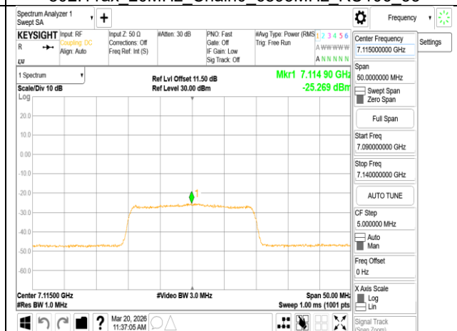
802.11ax_20MHz_Chain0_7115MHz
