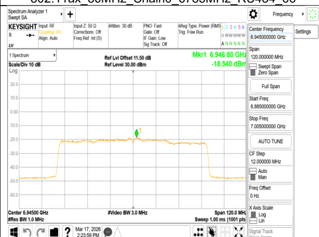
802.11ax 80MHz Chain0 6945MHz
