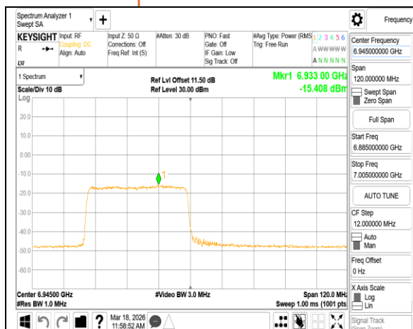
802.11ax 80MHz Chain0 6945MHz RU484 65
