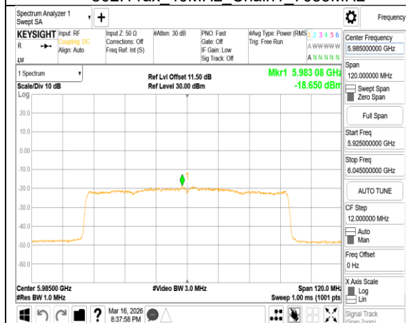
802.11ax_80MHz_Chain0_5985MHz
