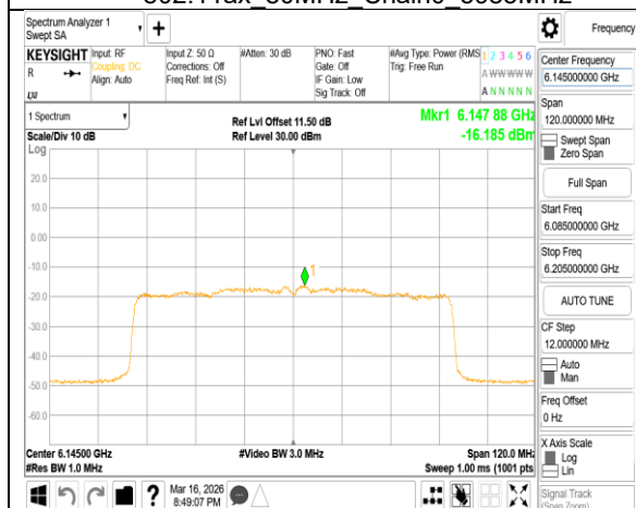
802.11ax_80MHz_Chain0_6145MHz
