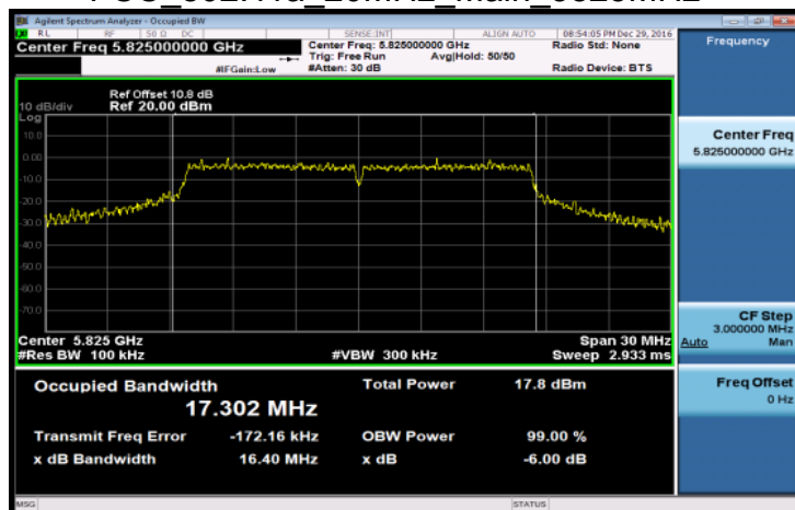
FCC_802.11a_20MHz_Main_5825MHz
