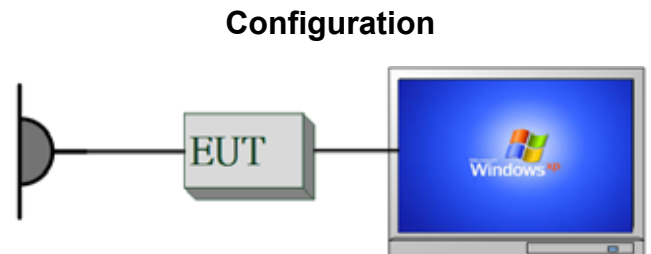
Fig 2-2 Radiated Emission
