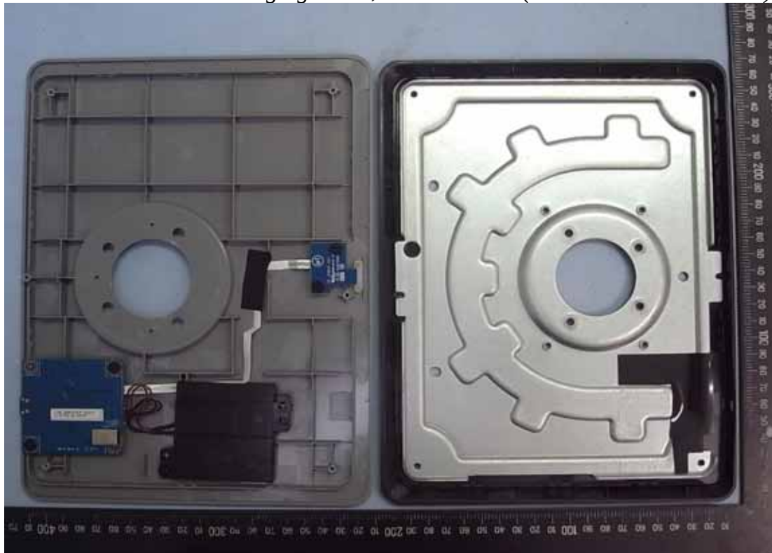
Figure 23 Wireless Charging Stand, Internal View (Removed Shielded Case)
