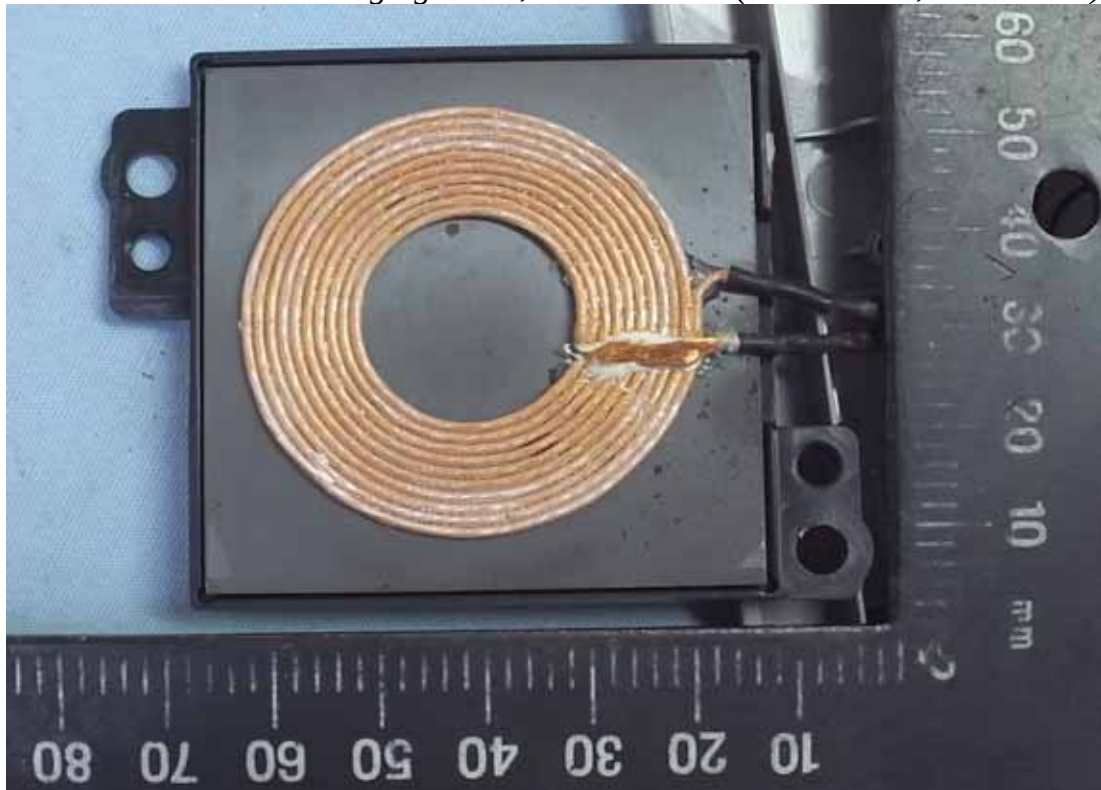
Figure 25 Wireless Charging Stand, Internal View (WPC Board, Front View)
