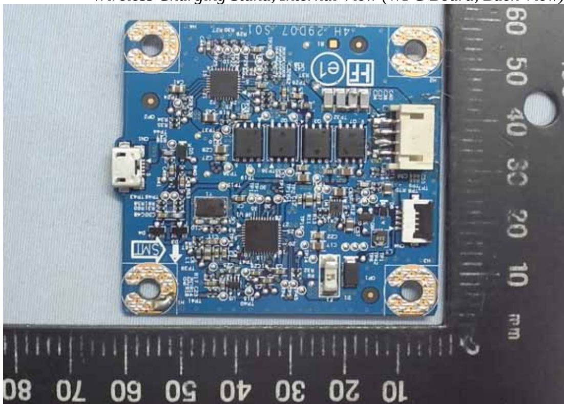
Figure 26 Wireless Charging Stand, Internal View (WPC Board, Back View)
