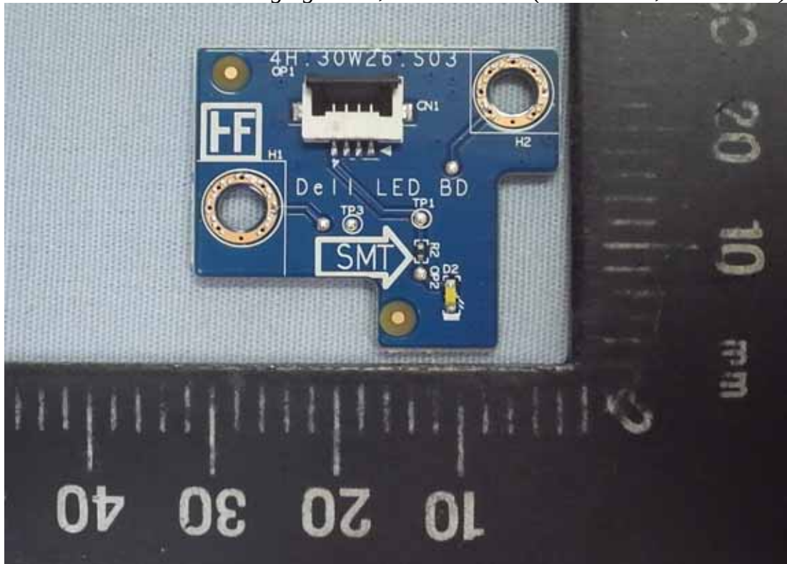
Figure 27 Wireless Charging Stand, Internal View (USB Board, Front View)
