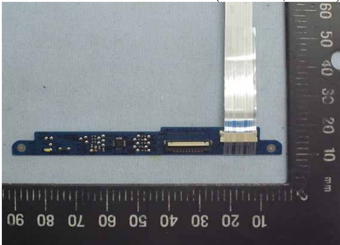
Figure 17 Internal View (Control Board, Front View)
