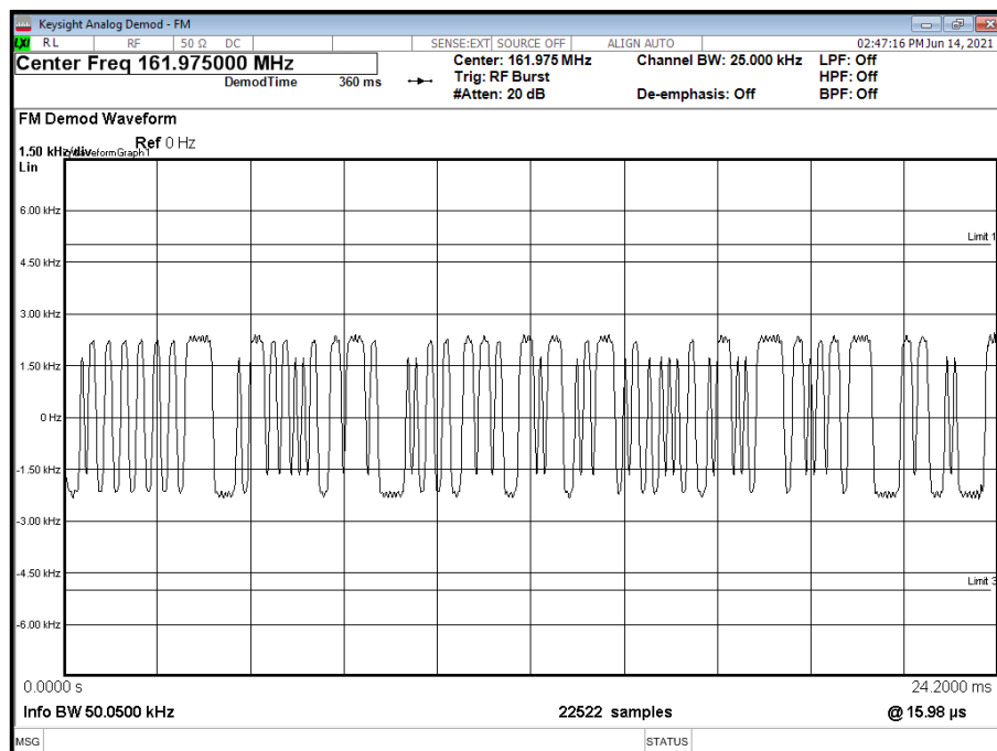
Figure 17- 161.975 MHz - PRBS
