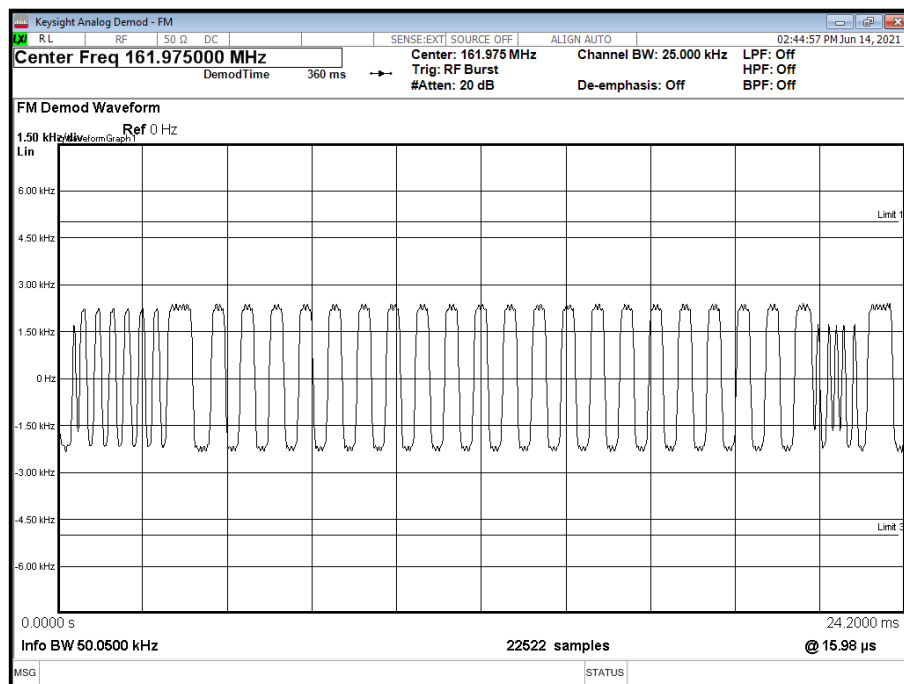
Figure 16- 161.975 MHz - 00001111
