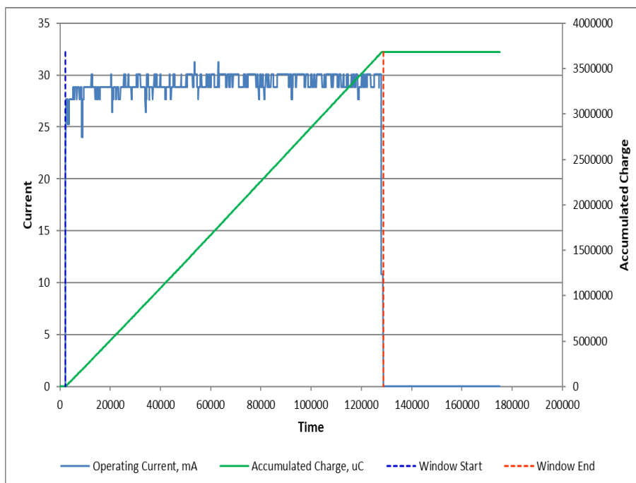
Float Free Case + VDR data link, GNSS Self-test (Timeout): B7
