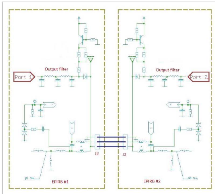
Figure 2: Measurement setup
