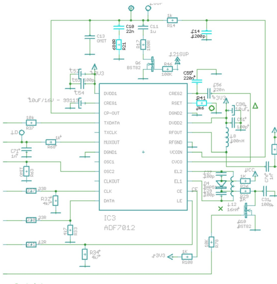
Figure 1: Loop filter
