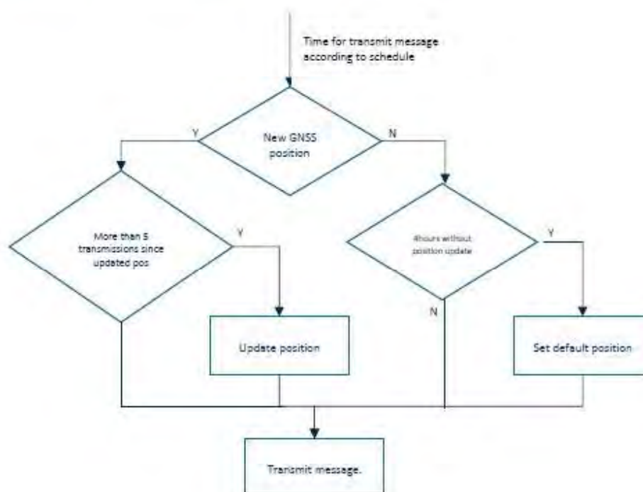
5 Simplified transmission of 406 message
