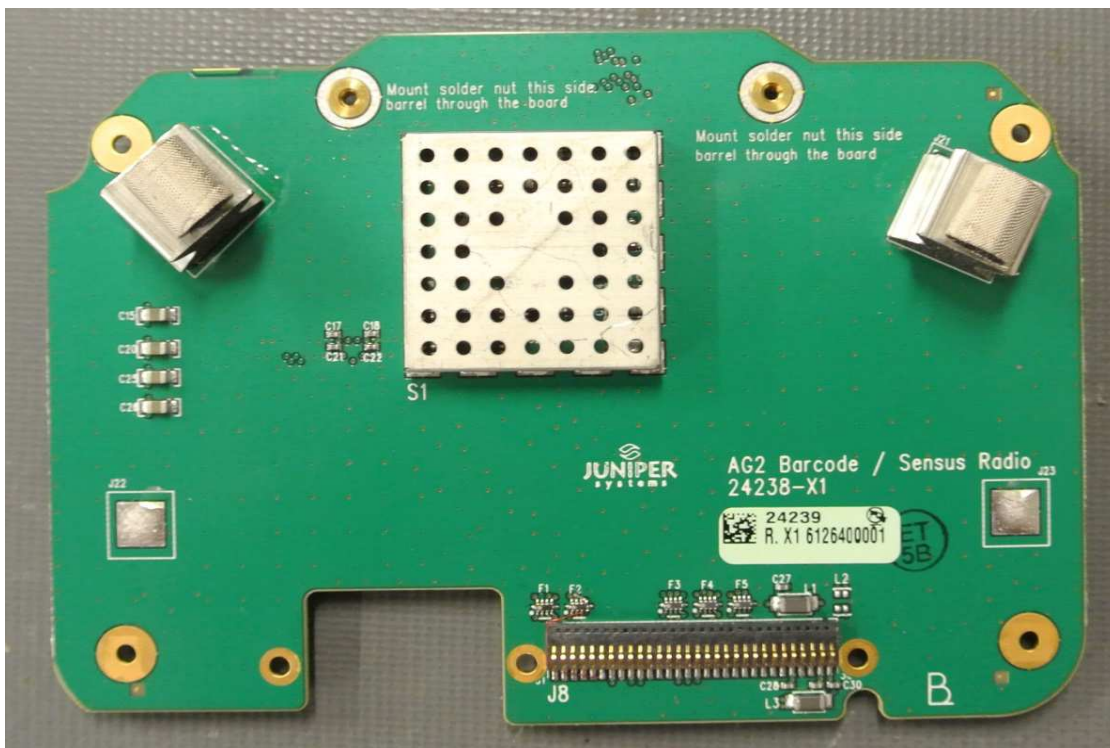
Sensus radio and barcode interface board (top)
