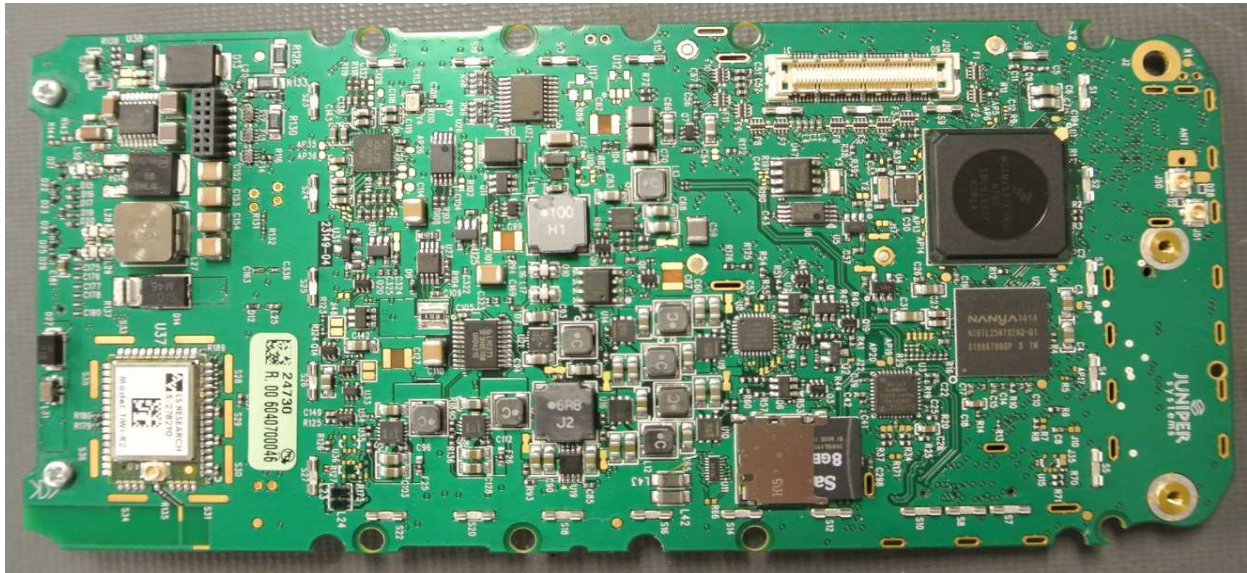
Mainboard top with shields removed
