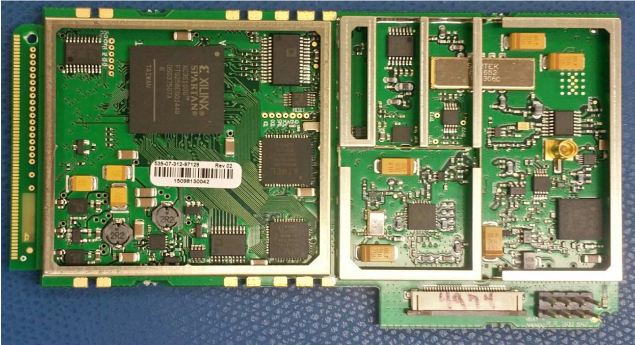
PRIU with LPL Top FL 6502
