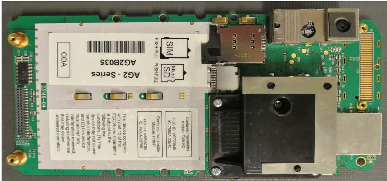
Mainboard bottom with shields and cellular antenna
