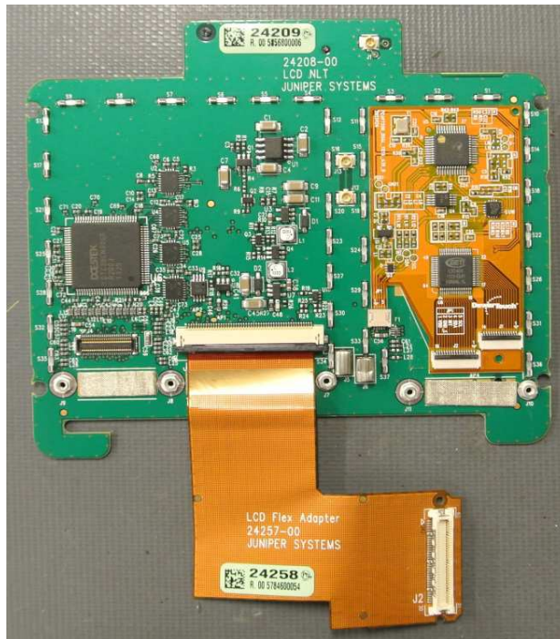
LCD adapter board (top) without shields
