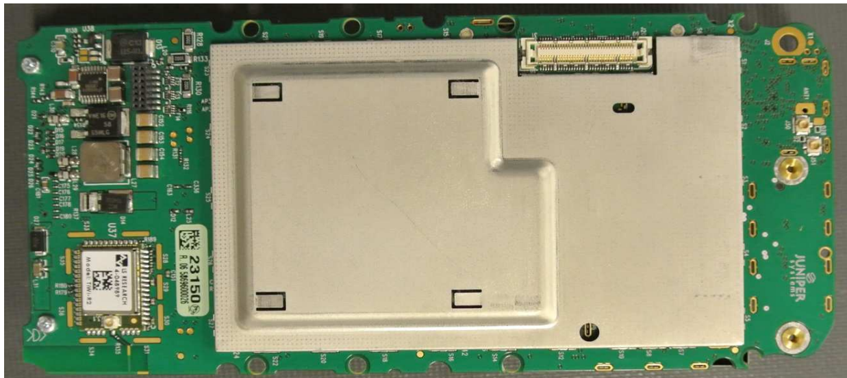
Mainboard top with shields
