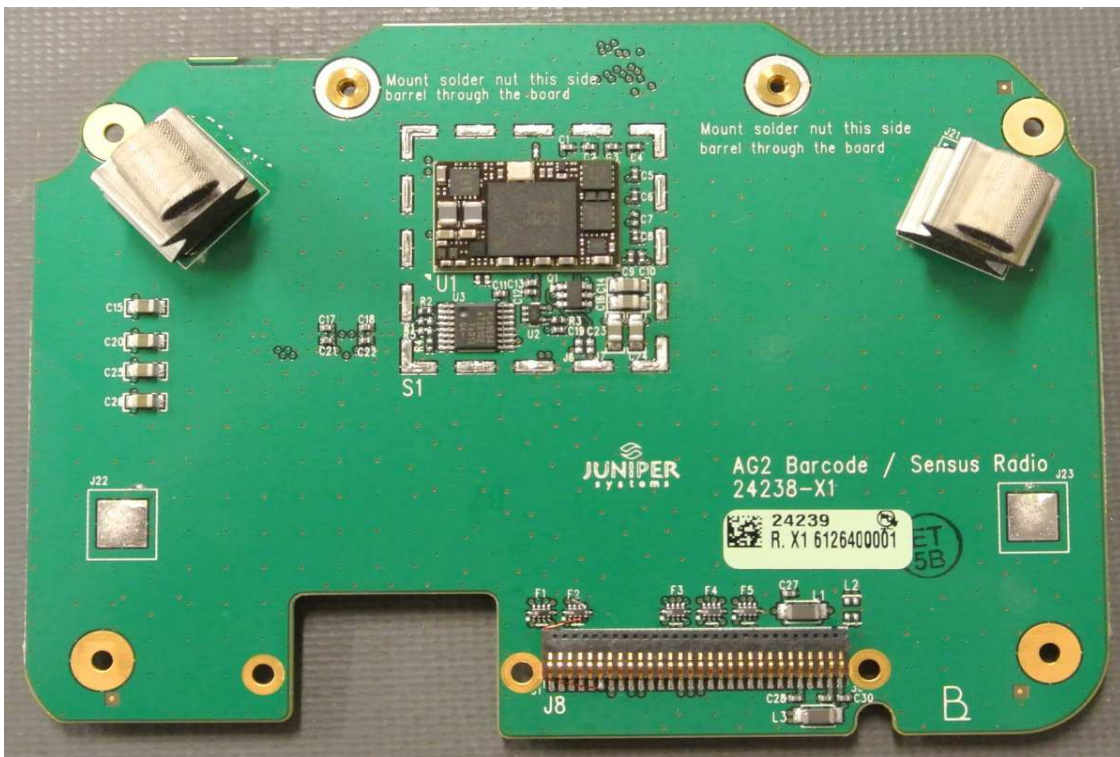
Sensus radio and barcode interface board (top) - shields removed
