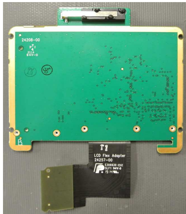
LCD adapter board (bottom) and tail
