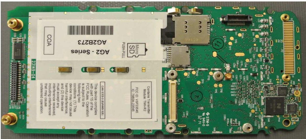
Mainboard bottom with shields removed
