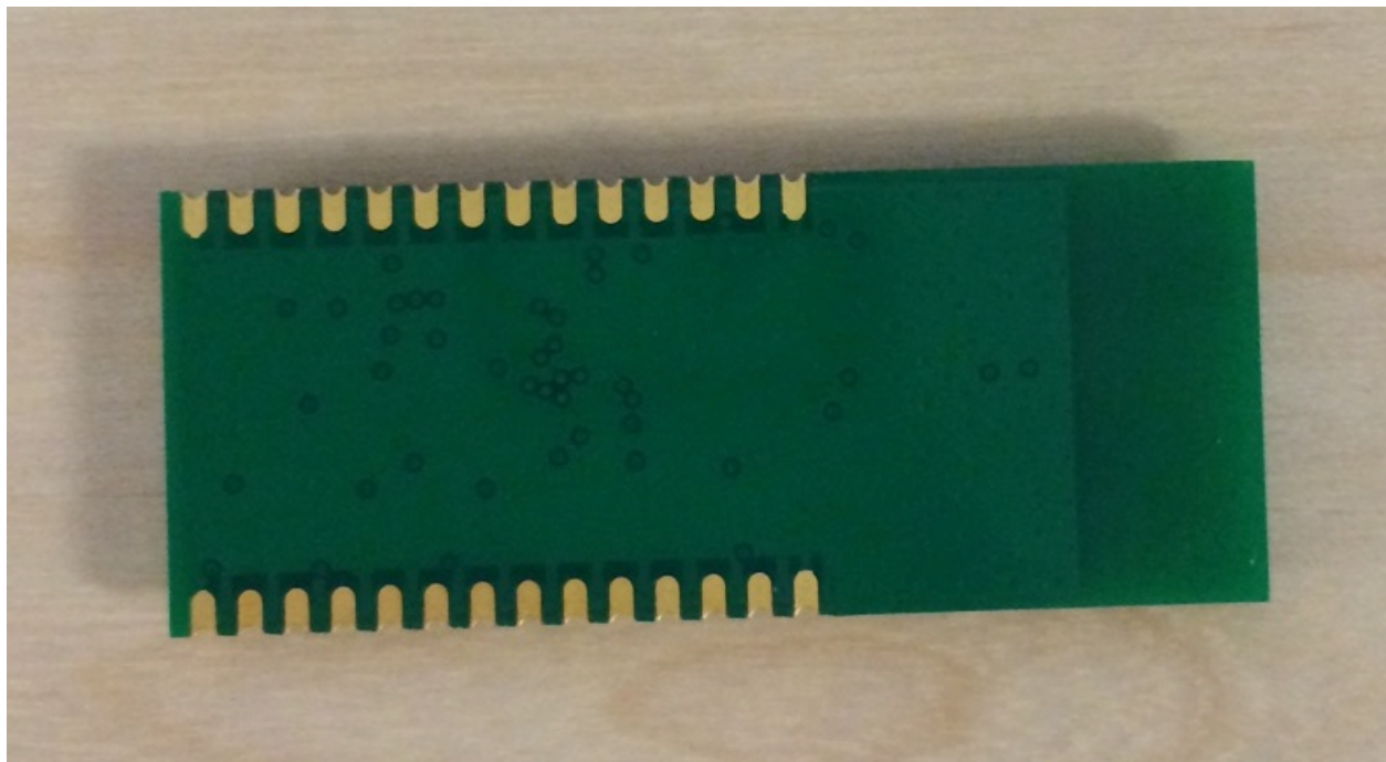
Figure 2: External Photo
