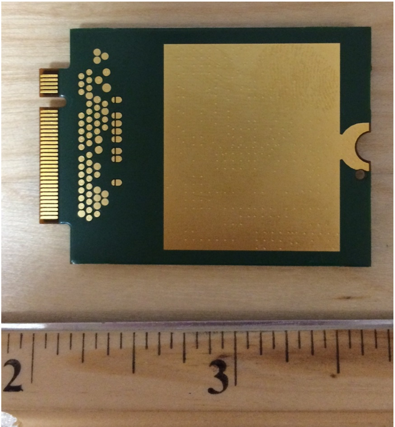
Figure 2: EM7355 – Bottom View
