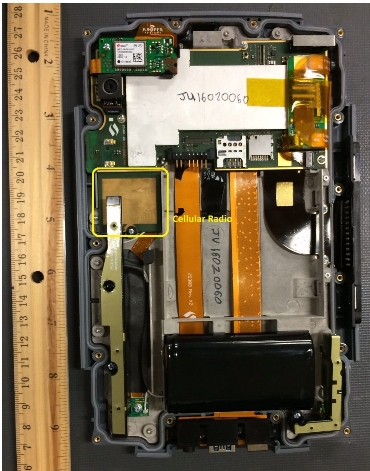
Figure 3: Assembled - View 1
