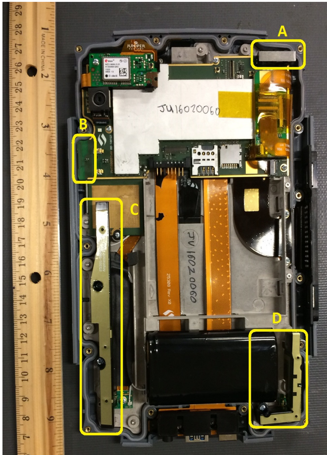
Figure 4: Assembled - View 2
