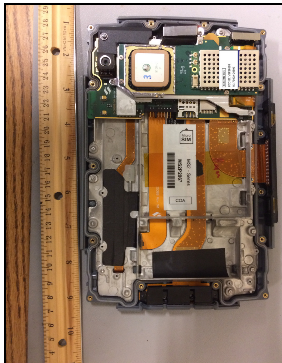
Figure 7: Module installed in Host
