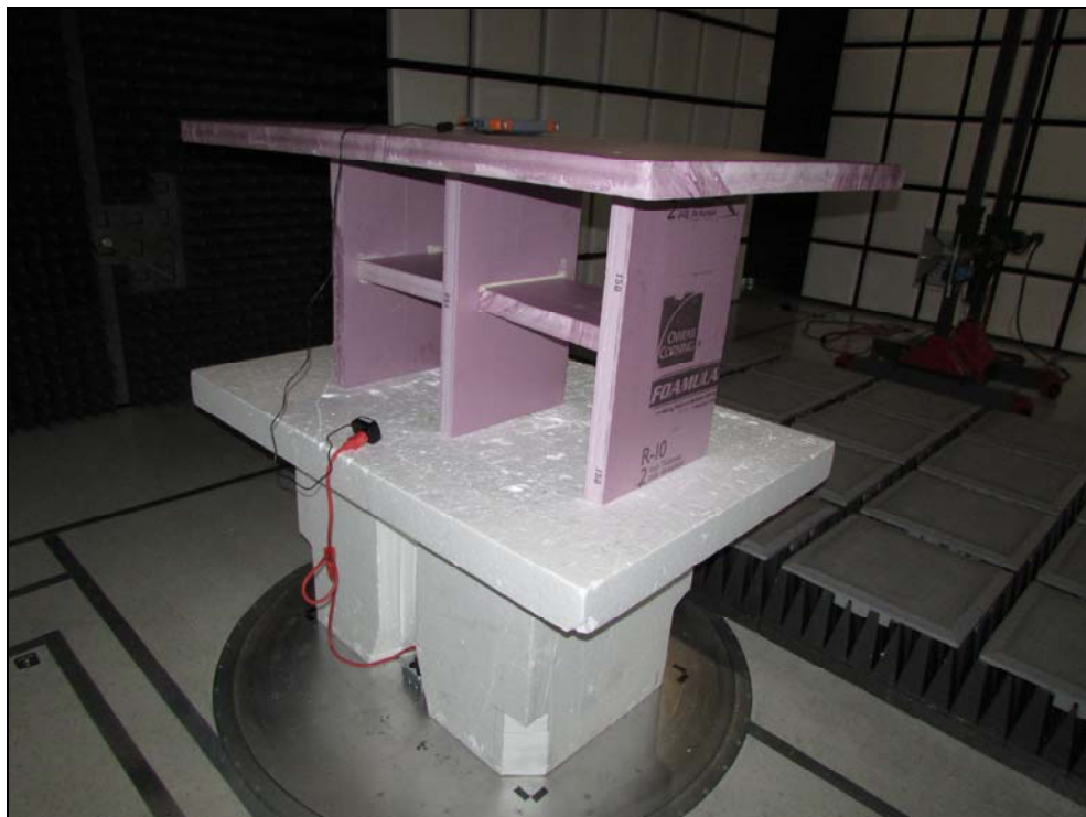
Figure 4: Radiated Spurious Emissions Above 1 GHz - Back
