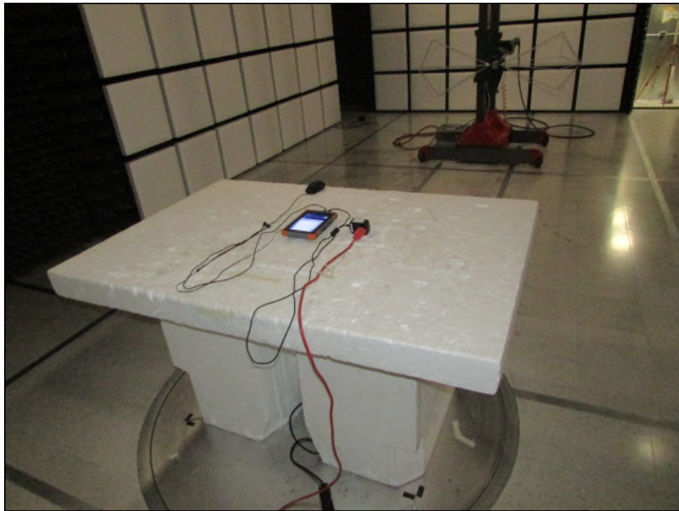
Figure 1: Radiated Emissions – Below 1GHz - Rear View
