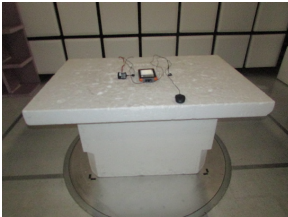
Figure 2: Radiated Emissions – Below 1 GHz – Front View
