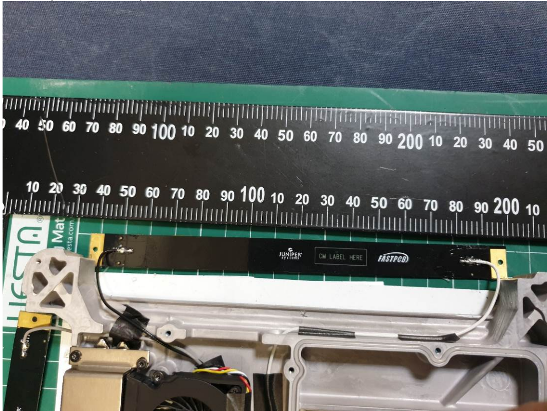
(38) EUT Photo (Main Antenna)
