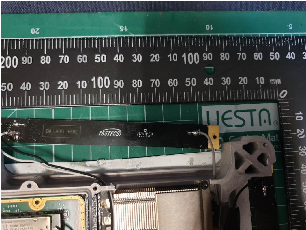
(35) EUT Photo (Cell Aux Antenna)
