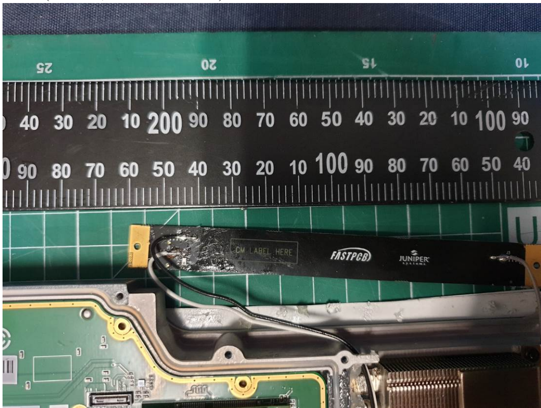
(34) EUT Photo (WiFi/BT, GPS Aux Antenna)
