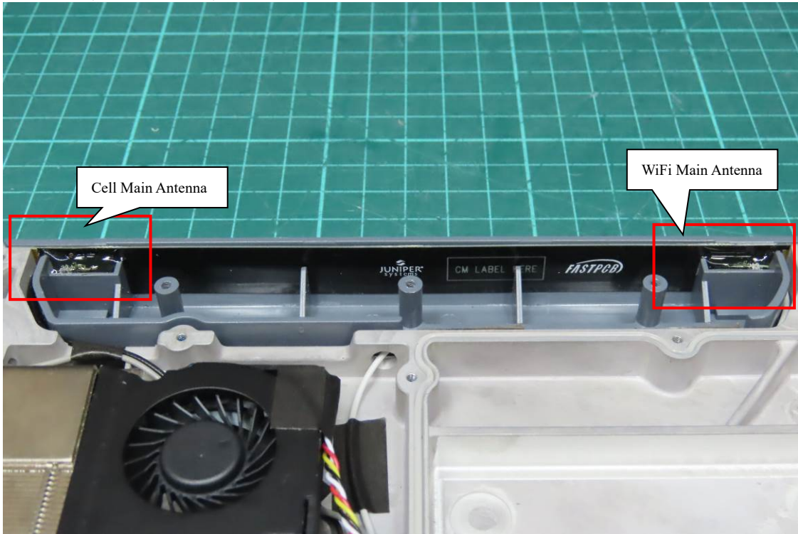
(37) EUT Photo (Main Antenna)
