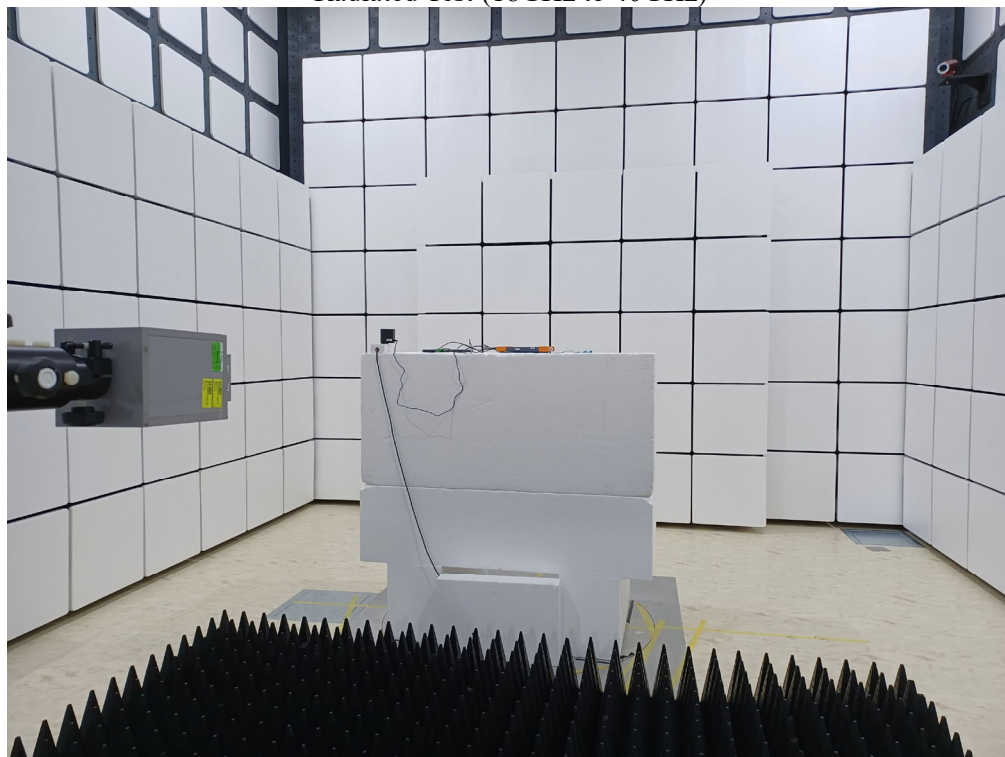
Radiated Test (18GHz to 40GHz)
