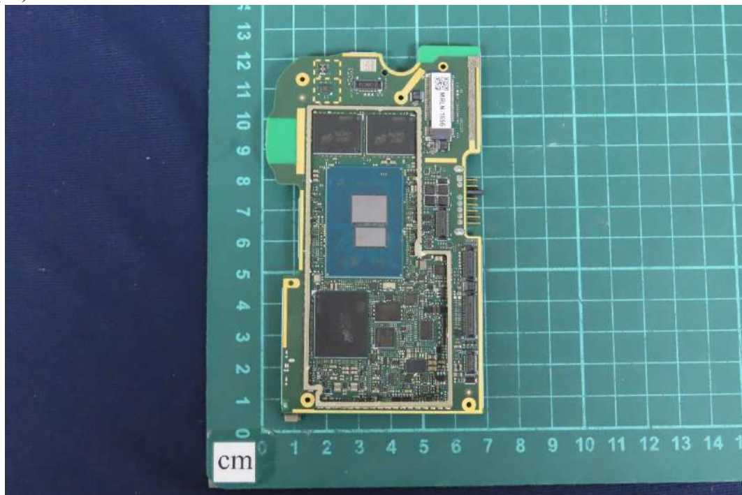
(89) EUT Photo
