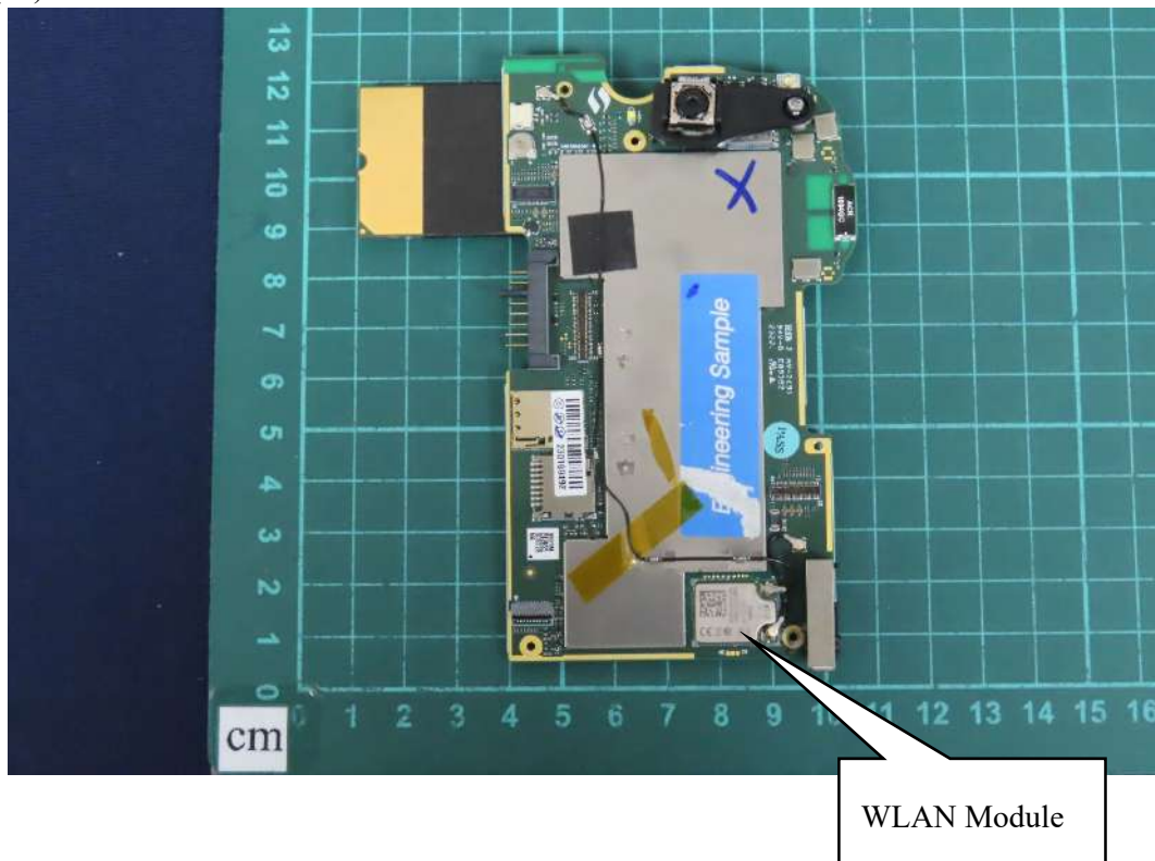
(35) EUT Photo
