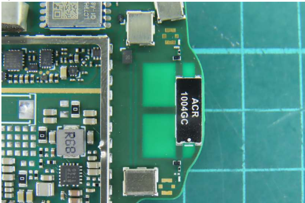
(42) EUT Photo
