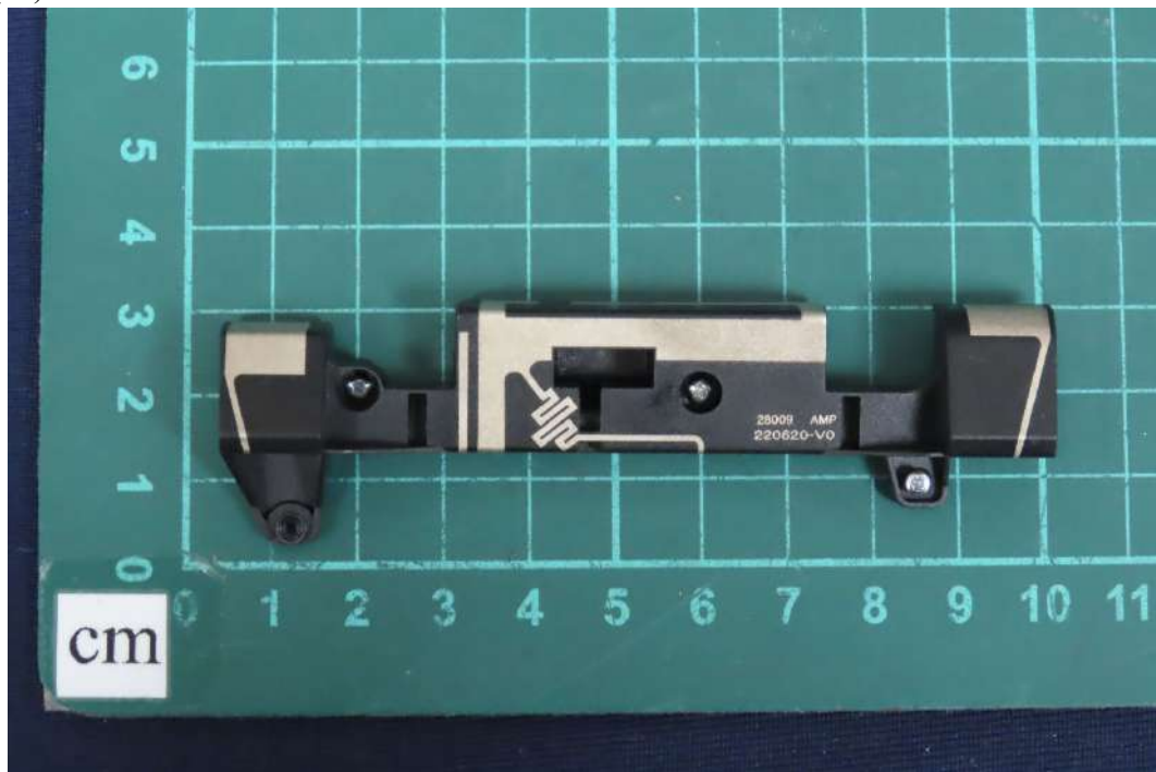
(73) EUT Photo
