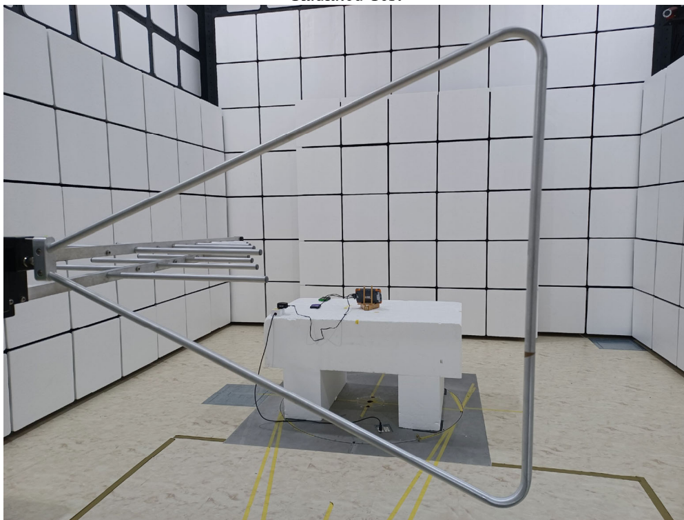
Radiated Test
