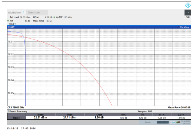
NTNV-N77-3700-3980-PC2-30-60-L-DFT-QPSK-Edge_1RB_Left-PASS
