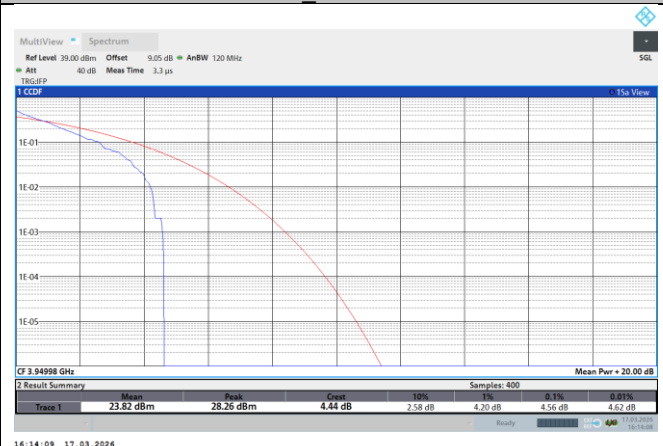
NTNV-N77-3700-3980-PC2-30-60-H-DFT-QPSK-Outer_Full-PASS
