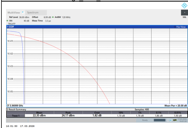
NTNV-N77-3700-3980-PC2-30-20-H-DFT-QPSK- Edge_1RB_Left-PASS
