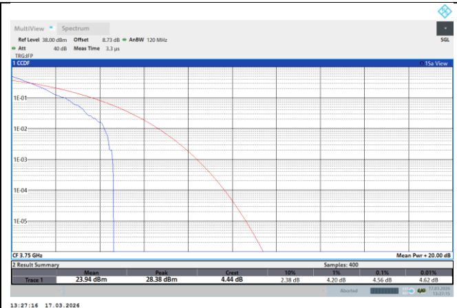
NTNV-N77-3700-3980-PC2-30-100-L-DFT-QPSK-Outer_Full-PASS
