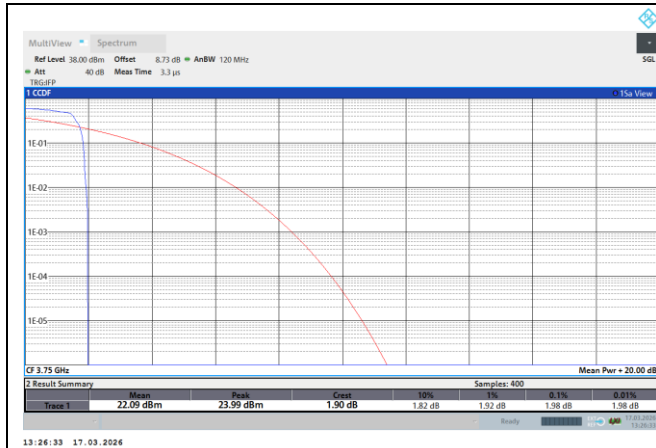
NTNV-N77-3700-3980-PC2-30-100-L-DFT-QPSK-Edge_1RB_Left-PASS
