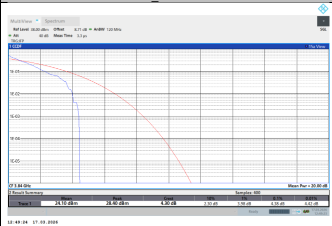
NTNV-N77-3700-3980-PC2-30-20-M-DFT-QPSK- Outer_Full-PASS
