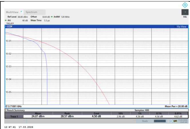
NTNV-N77-3700-3980-PC2-30-20-L-DFT-QPSK- Outer_Full-PASS
