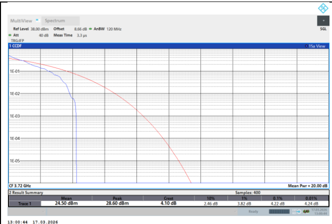
NTNV-N77-3700-3980-PC2-30-40-L-DFT-QPSK-Outer_Full-PASS
