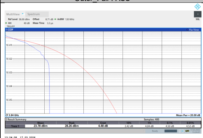
NTNV-N77-3700-3980-PC2-30-80-M-DFT-QPSK-Outer_Full-PASS
