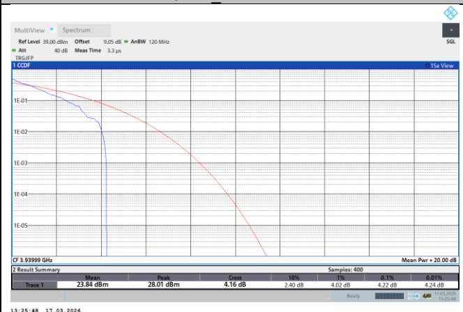
NTNV-N77-3700-3980-PC2-30-80-H-DFT-QPSK-Outer_Full-PASS
