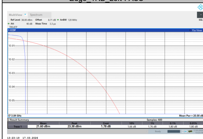
NTNV-N77-3700-3980-PC2-30-80-M-DFT-QPSK-Edge_1RB_Left-PASS
