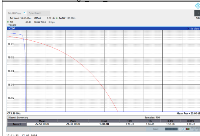
NTNV-N77-3700-3980-PC2-30-40-H-DFT-QPSK-Edge_1RB_Left-PASS
