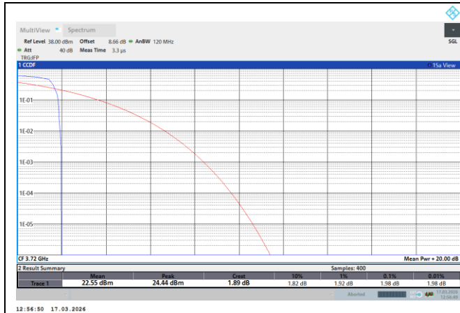
NTNV-N77-3700-3980-PC2-30-40-L-DFT-QPSK-Edge_1RB_Left-PASS
