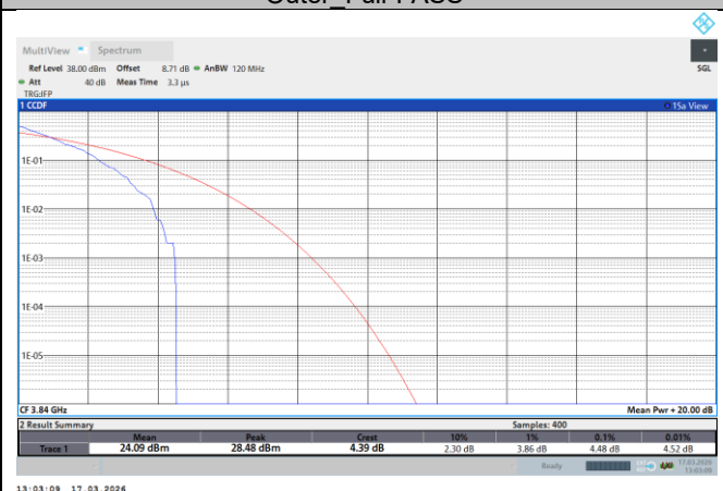
NTNV-N77-3700-3980-PC2-30-40-M-DFT-QPSK-Outer_Full-PASS
