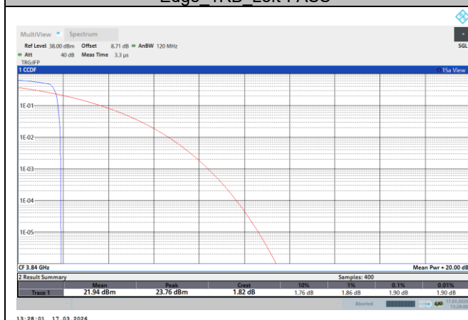
NTNV-N77-3700-3980-PC2-30-100-M-DFT-QPSK-Edge_1RB_Left-PASS
