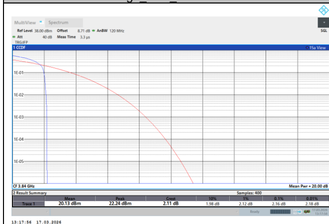
NTNV-N77-3700-3980-PC2-30-60-M-DFT-QPSK-Edge_1RB_Left-PASS
