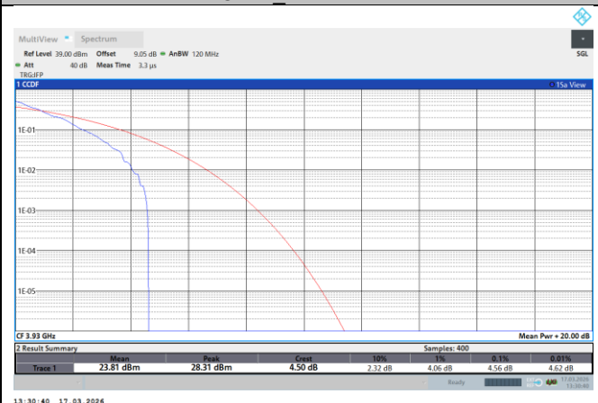
NTNV-N77-3700-3980-PC2-30-100-H-DFT-QPSK-Outer_Full-PASS
