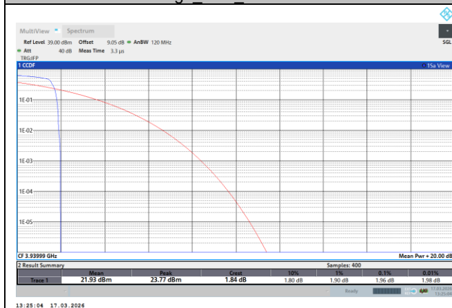
NTNV-N77-3700-3980-PC2-30-80-H-DFT-QPSK-Edge_1RB_Left-PASS
