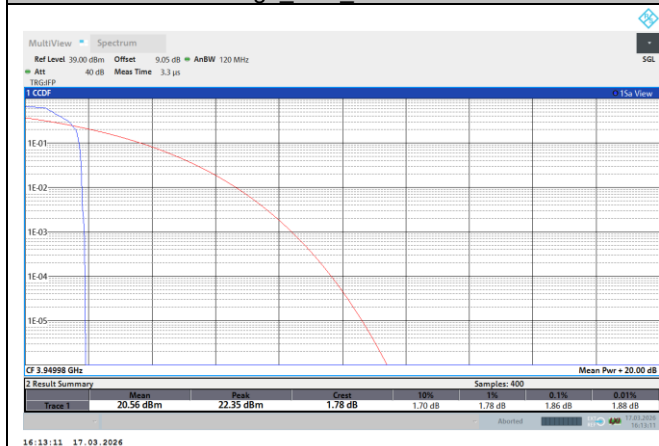
NTNV-N77-3700-3980-PC2-30-60-H-DFT-QPSK-Edge_1RB_Left-PASS
