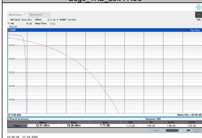
NTNV-N77-3700-3980-PC2-30-40-M-DFT-QPSK-Edge_1RB_Left-PASS
