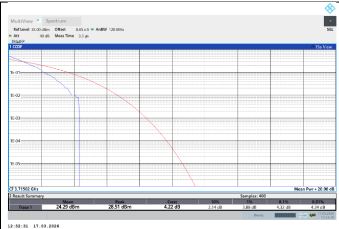
NTNV-N77-3700-3980-PC2-30-30-L-DFT-QPSK-Outer_Full-PASS
