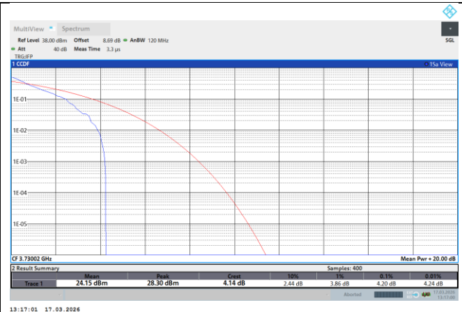
NTNV-N77-3700-3980-PC2-30-60-L-DFT-QPSK-Outer_Full-PASS
