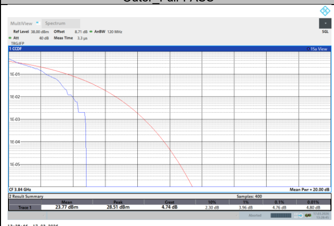
NTNV-N77-3700-3980-PC2-30-100-M-DFT-QPSK-Outer_Full-PASS
