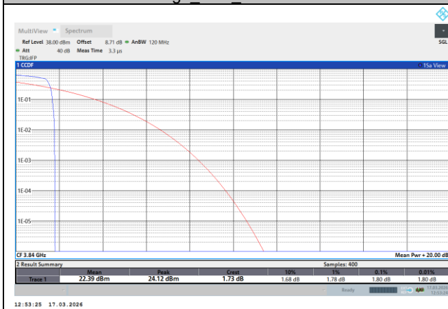
NTNV-N77-3700-3980-PC2-30-30-M-DFT-QPSK-Edge_1RB_Left-PASS
