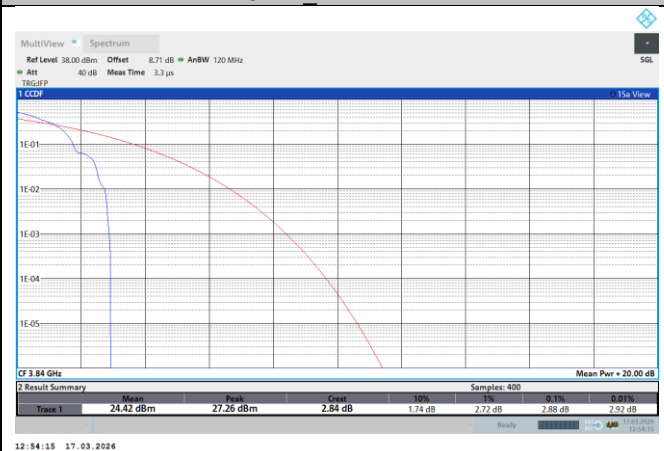
NTNV-N77-3700-3980-PC2-30-30-M-DFT-QPSK-Outer_Full-PASS
