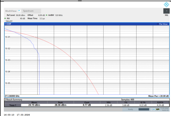
NTNV-N77-3700-3980-PC2-30-20-H-DFT-QPSK- Outer_Full-PASS
