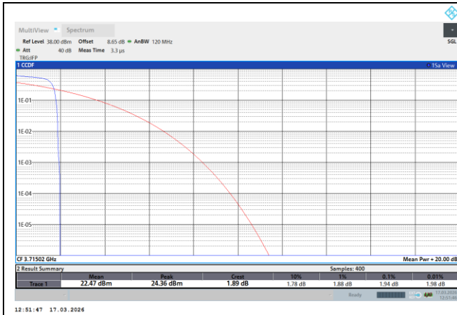
NTNV-N77-3700-3980-PC2-30-30-L-DFT-QPSK-Edge_1RB_Left-PASS
