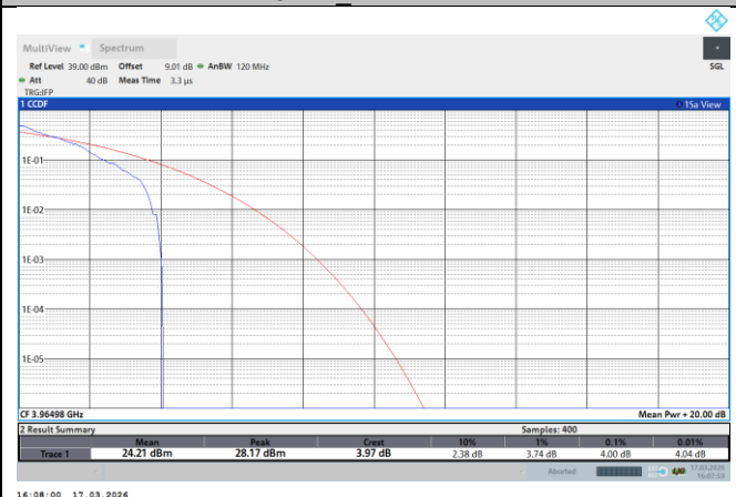
NTNV-N77-3700-3980-PC2-30-30-H-DFT-QPSK-Outer_Full-PASS
