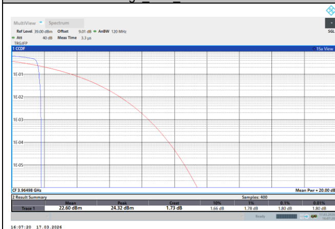
NTNV-N77-3700-3980-PC2-30-30-H-DFT-QPSK-Edge_1RB_Left-PASS
