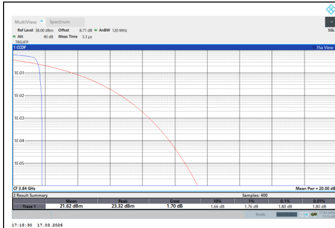
NTNV-N77-3700-3980-PC2-30-80-L-DFT-QPSK-Edge_1RB_Left-PASS
