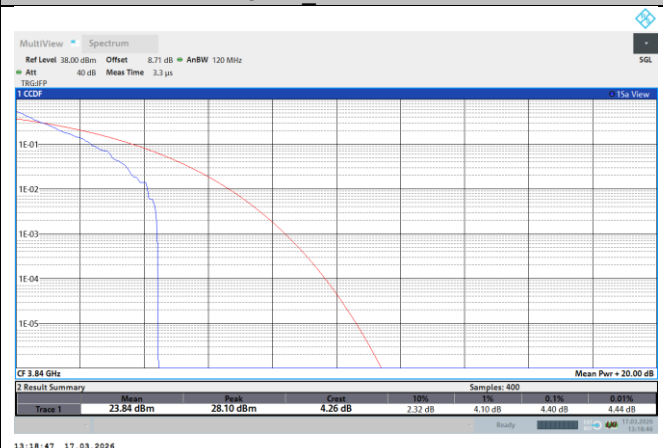
NTNV-N77-3700-3980-PC2-30-60-M-DFT-QPSK-Outer_Full-PASS
