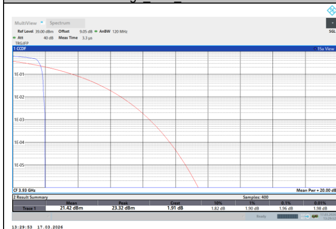
NTNV-N77-3700-3980-PC2-30-100-H-DFT-QPSK-Edge_1RB_Left-PASS
