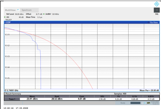
NTNV-N77-3700-3980-PC2-30-80-L-DFT-QPSK-Outer_Full-PASS
