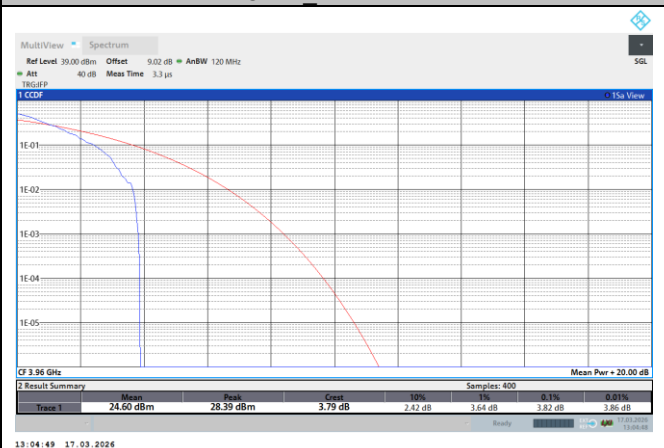
NTNV-N77-3700-3980-PC2-30-40-H-DFT-QPSK-Outer_Full-PASS
