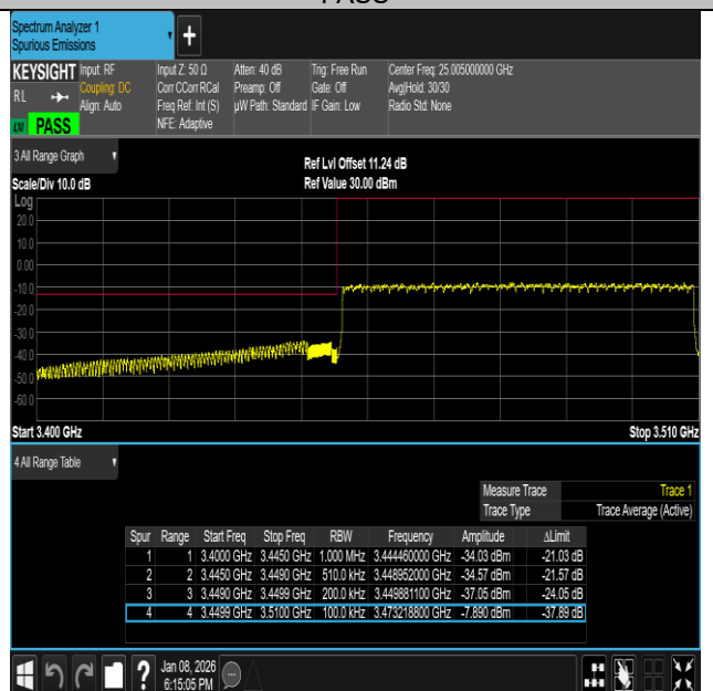
NTNV-n77(3450-3550)-PC2-30-60-H-DFT-QPSK-Outer_Full- PASS
