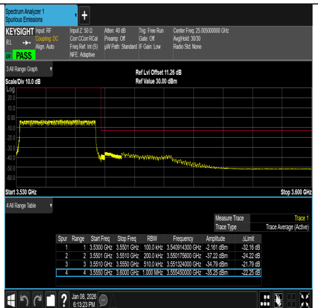
NTNV-n77(3450-3550)-PC2-30-60-L-DFT-QPSK-Outer_Full- PASS
