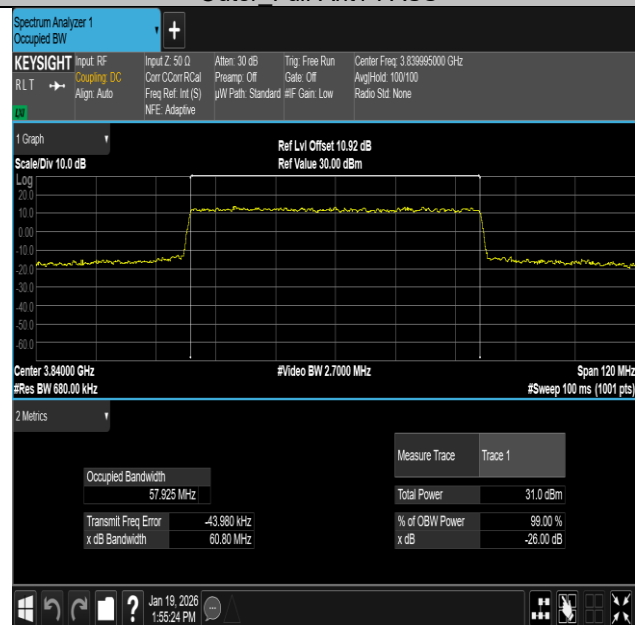
NTNV-n77(3700-3980)-PC2-30-60-M-DFT-16QAM- Outer_Full-Ant1-PASS
