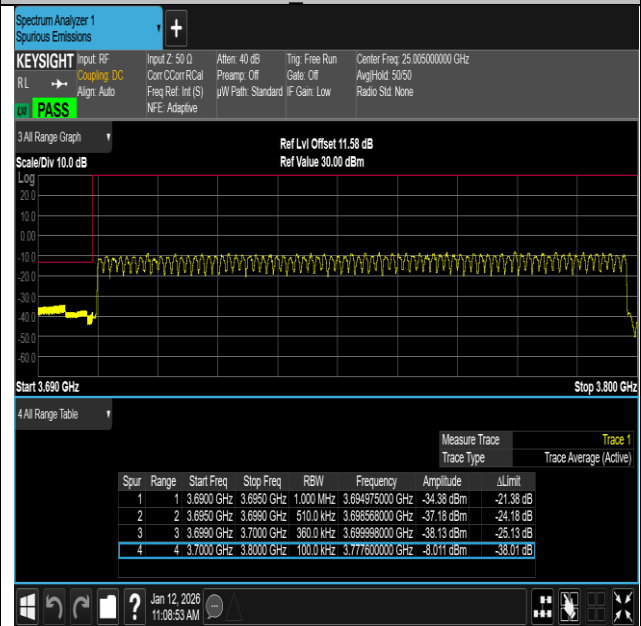
NTNV-n77(3700-3980)-PC2-30-100-H-DFT-QPSK- Outer Full-PASS
