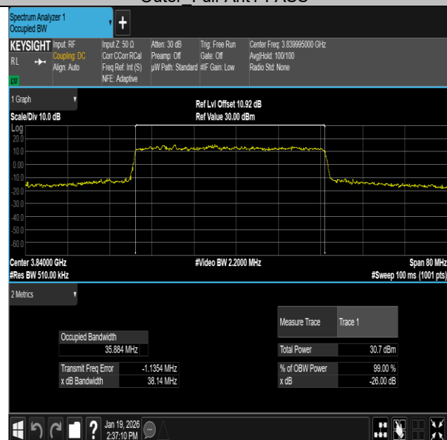
NTNV-n77(3700-3980)-PC2-30-40-M-DFT-64QAM- Outer_Full-Ant1-PASS
