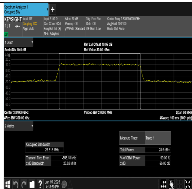
NTNV-n77(3700-3980)-PC2-30-40-M-DFT-QPSK- Outer_Full-Ant1-PASS
