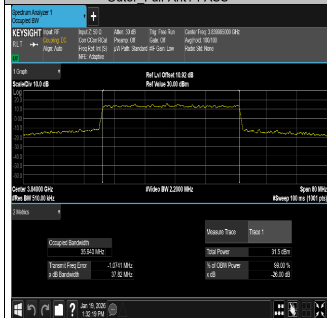
NTNV-n77(3700-3980)-PC2-30-40-M-DFT-256QAM- Outer_Full-Ant1-PASS
