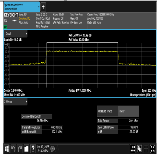
NTNV-n77(3700-3980)-PC2-30-100-M-DFT-256QAM- Outer_Full-Ant1-PASS
