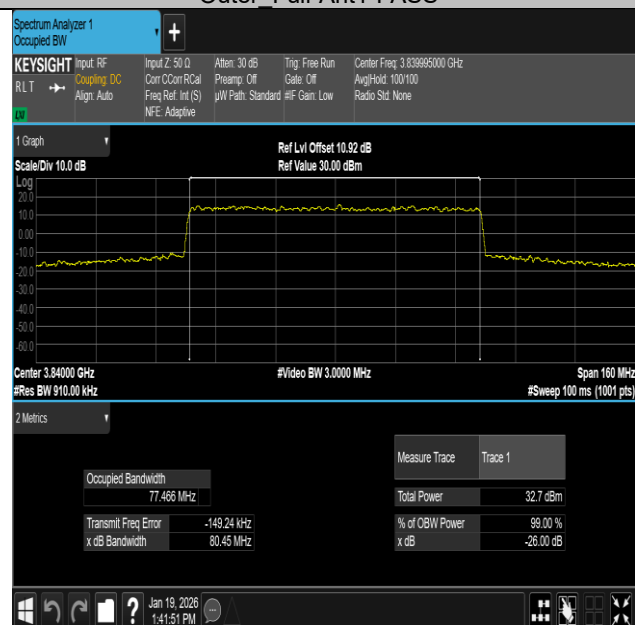
NTNV-n77(3700-3980)-PC2-30-80-M-DFT-64QAM- Outer_Full-Ant1-PASS
