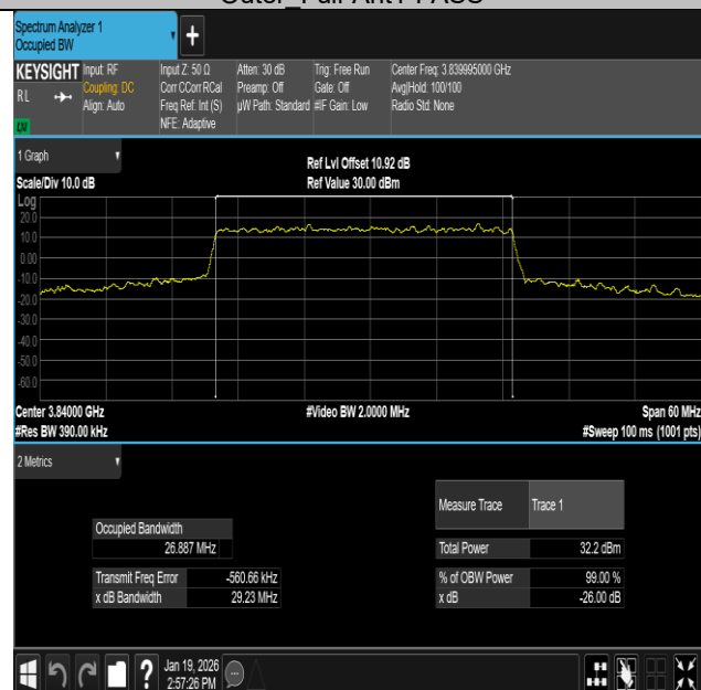
NTNV-n77(3700-3980)-PC2-30-30-M-DFT-16QAM- Outer_Full-Ant1-PASS
