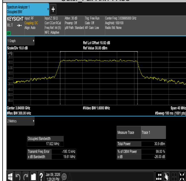
NTNV-n77(3700-3980)-PC2-30-30-M-DFT-QPSK- Outer_Full-Ant1-PASS
