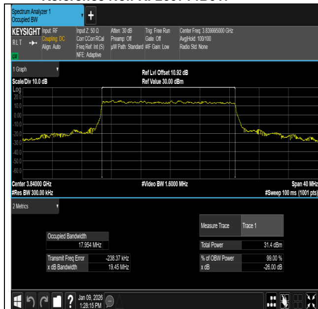
NTNV-n77(3700-3980)-PC2-30-20-M-DFT-256QAM- Outer_Full-Ant1-PASS
