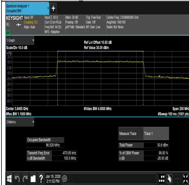
NTNV-n77(3700-3980)-PC2-30-100-M-DFT-64QAM- Outer_Full-Ant1-PASS
