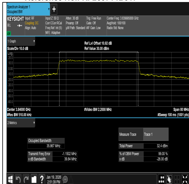
NTNV-n77(3700-3980)-PC2-30-40-M-DFT-16QAM- Outer_Full-Ant1-PASS
