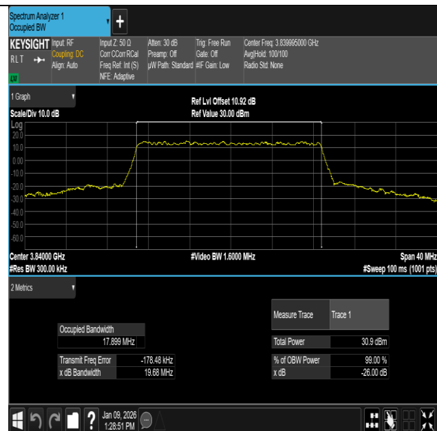
NTNV-n77(3700-3980)-PC2-30-30-M-DFT-BPSK- Outer_Full-Ant1-PASS
