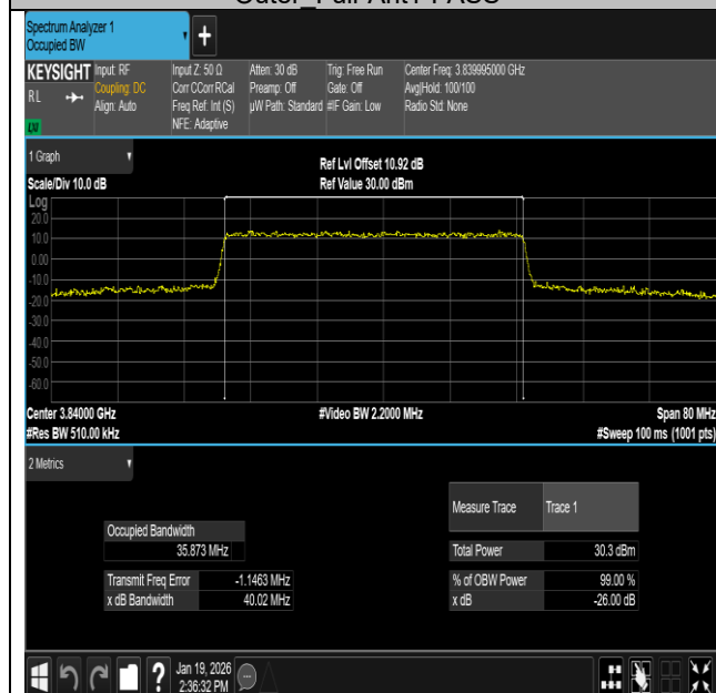
NTNV-n77(3700-3980)-PC2-30-40-M-DFT-16QAM- Outer_Full-Ant1-PASS
