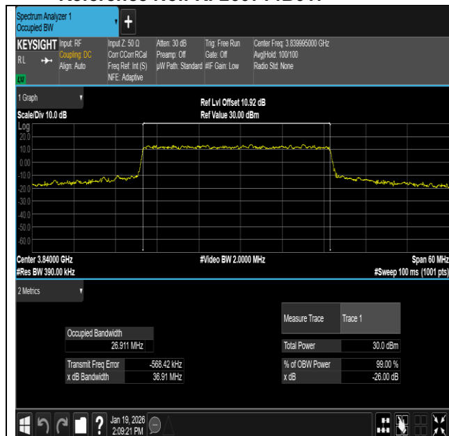
NTNV-n77(3700-3980)-PC2-30-40-M-DFT-BPSK- Outer_Full-Ant1-PASS
