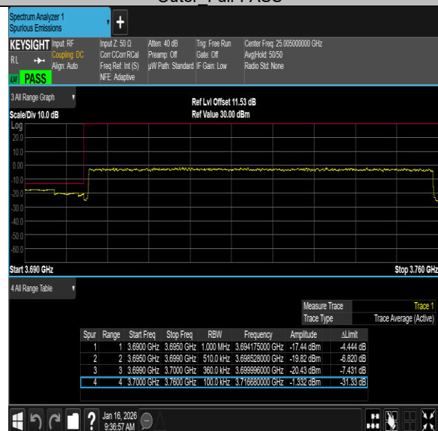
NTNV-n77(3700-3980)-PC2-30-60-H-DFT-QPSK- Outer Full-PASS
