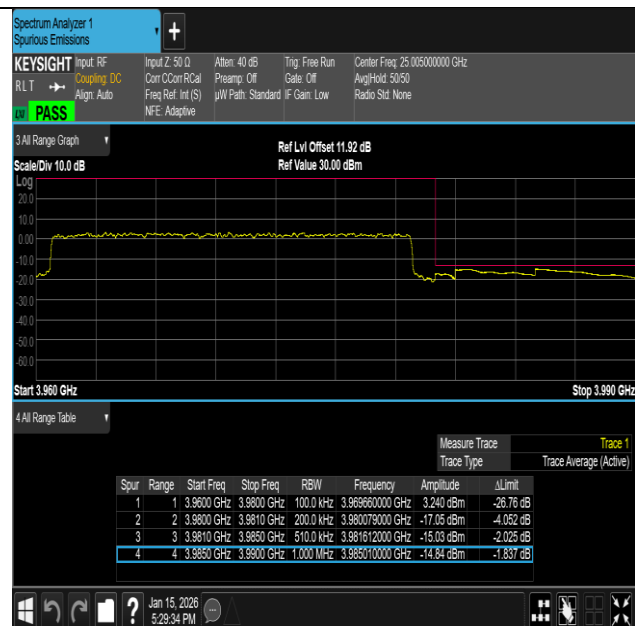
NTNV-n77(3700-3980)-PC2-30-60-L-DFT-QPSK- Outer Full-PASS
