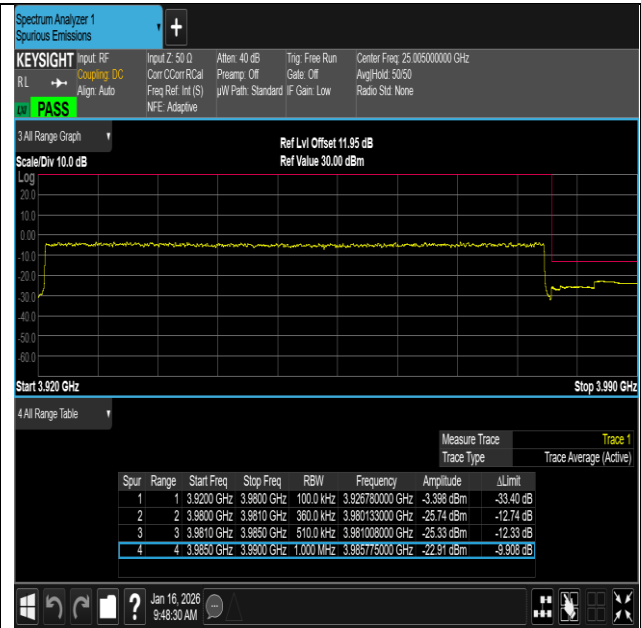
NTNV-n77(3700-3980)-PC2-30-100-L-DFT-QPSK- Outer Full-PASS
