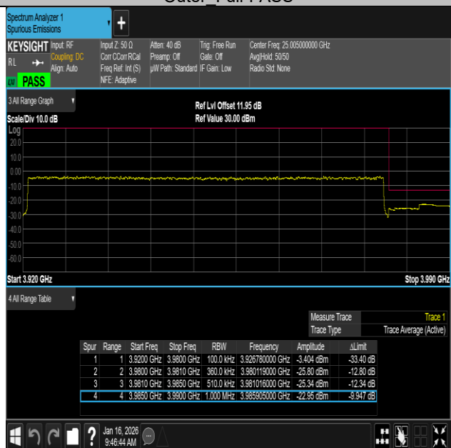
NTNV-n77(3700-3980)-PC2-30-100-L-DFT-QPSK- Outer Full-PASS
