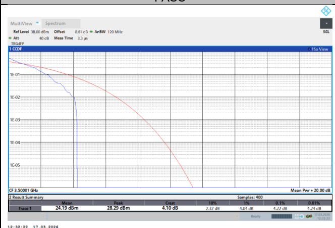
NTNV-N77-3450-3550-PC2-30-60-M-DFT-QPSK-Outer_Full-PASS
