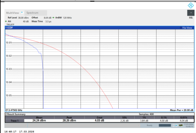
NTNV-N78-3450-3550-PC2-70-50-L-DFT-QPSK-Outer_Full-PASS
