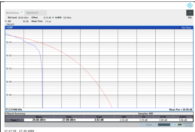
NTNV-N78-3450-3550-PC2-70-70-H-DFT-QPSK-Outer_Full-PASS
