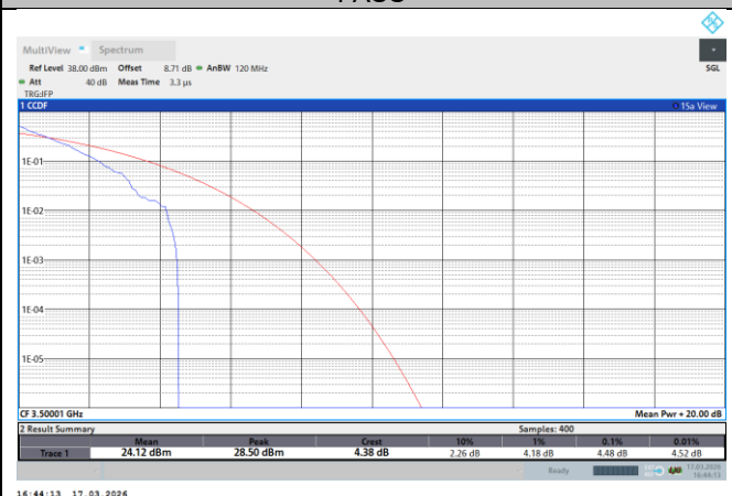
NTNV-N78-3450-3550-PC2-70-90-M-DFT-QPSK-Outer_Full-PASS
