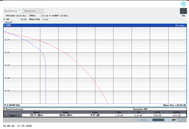
NTNV-N78-3450-3550-PC2-70-90-H-DFT-QPSK-Outer_Full-PASS
