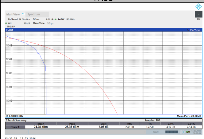
NTNV-N77-3450-3550-PC2-30-80-M-DFT-QPSK-Outer_Full-PASS
