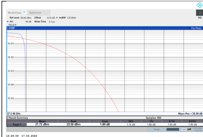
NTNV-N77-3450-3550-PC2-30-60-L-DFT-QPSK-Edge_1RB_Left-PASS
