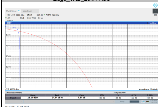
NTNV-N77-3450-3550-PC2-30-60-M-DFT-QPSK-Edge_1RB_Left-PASS
