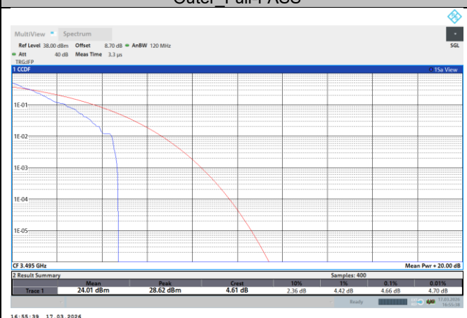
NTNV-N78-3450-3550-PC2-70-90-L-DFT-QPSK-Outer_Full-PASS
