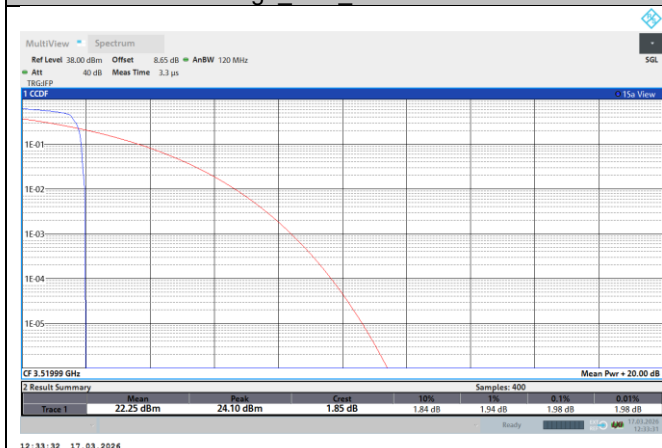
NTNV-N77-3450-3550-PC2-30-60-H-DFT-QPSK-Edge_1RB_Left-PASS
