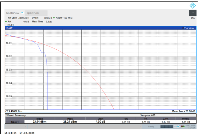
NTNV-N77-3450-3550-PC2-30-80-L-DFT-QPSK-Outer_Full-PASS
