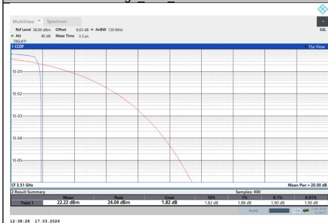
NTNV-N77-3450-3550-PC2-30-80-H-DFT-QPSK-Edge_1RB_Left-PASS
