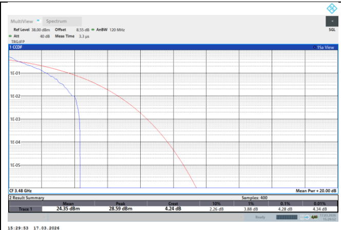
NTNV-N77-3450-3550-PC2-30-60-L-DFT-QPSK-Outer_Full-PASS
