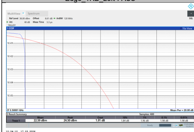
NTNV-N77-3450-3550-PC2-30-40-M-DFT-QPSK-Edge_1RB_Left-PASS
