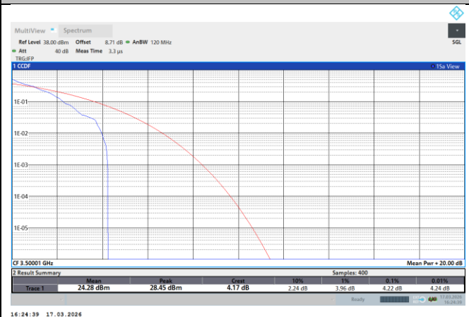
NTNV-N78-3450-3550-PC2-70-50-M-DFT-QPSK-Outer_Full-PASS
