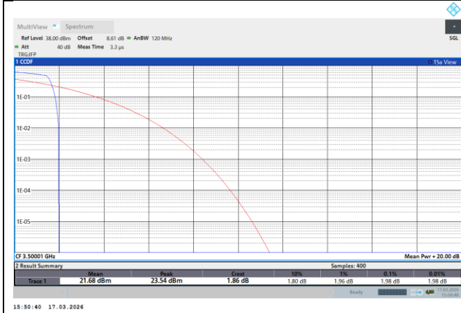
NTNV-N77-3450-3550-PC2-30-100-M-DFT-QPSK-Edge_1RB_Left-PASS
