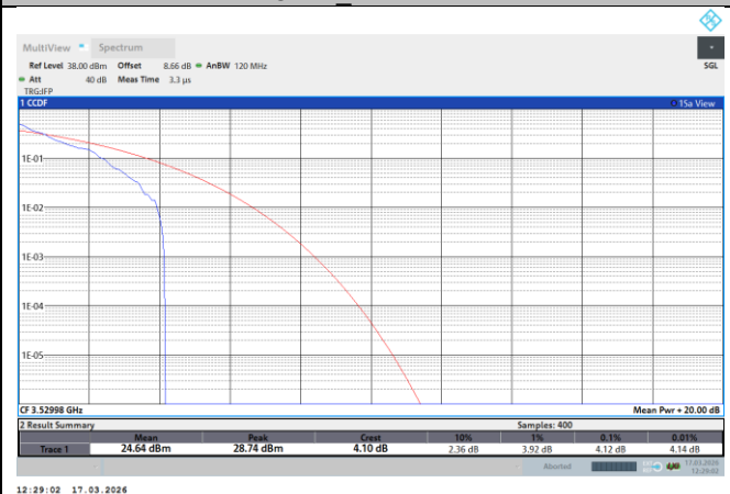
NTNV-N77-3450-3550-PC2-30-40-H-DFT-QPSK-Outer_Full-PASS
