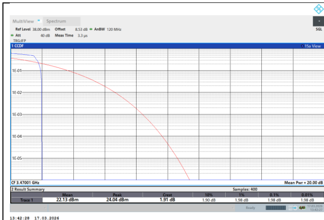
NTNV-N77-3450-3550-PC2-30-40-L-DFT-QPSK-Edge_1RB_Left-PASS
