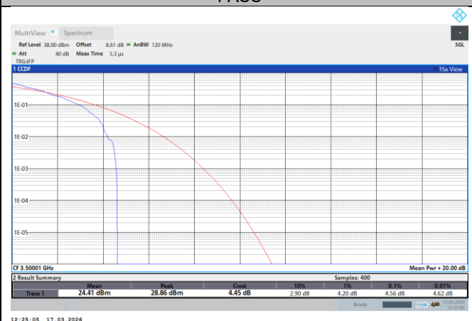
NTNV-N77-3450-3550-PC2-30-40-M-DFT-QPSK-Outer_Full-PASS
