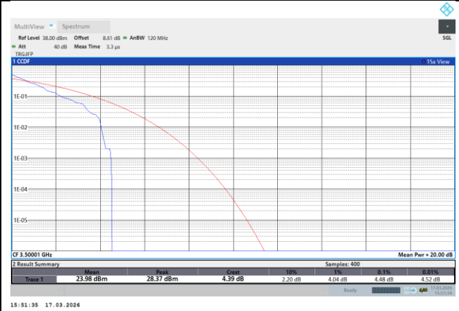
NTNV-N77-3450-3550-PC2-30-100-M-DFT-QPSK-Outer_Full-PASS
