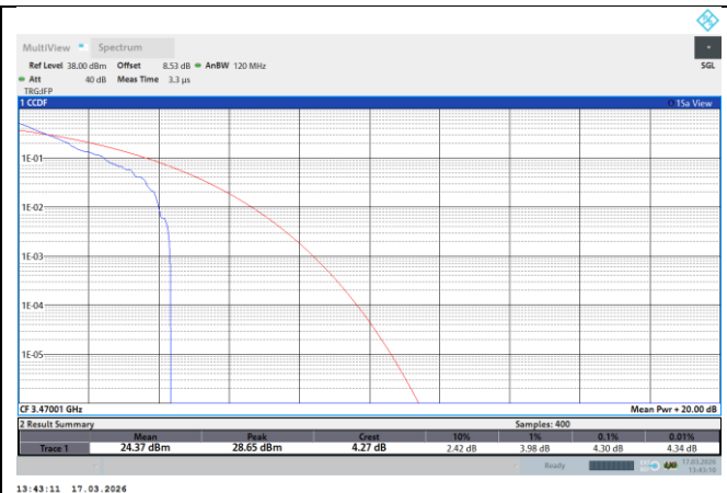
NTNV-N77-3450-3550-PC2-30-40-L-DFT-QPSK-Outer_Full-PASS
