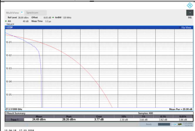
NTNV-N77-3450-3550-PC2-30-60-H-DFT-QPSK-Outer_Full-PASS
