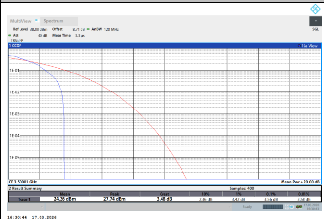
NTNV-N78-3450-3550-PC2-70-70-M-DFT-QPSK-Outer_Full-PASS
