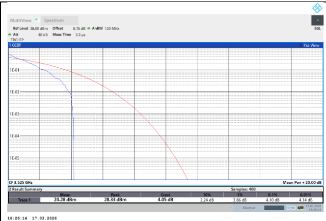
NTNV-N78-3450-3550-PC2-70-50-H-DFT-QPSK-Outer_Full-PASS
