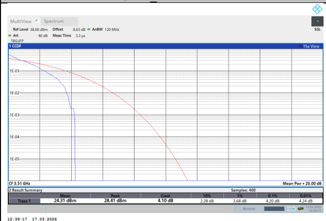
NTNV-N77-3450-3550-PC2-30-80-H-DFT-QPSK-Outer_Full-PASS
