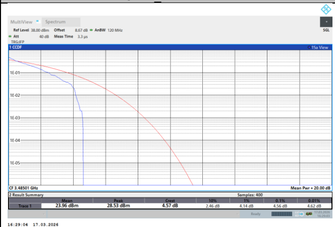
NTNV-N78-3450-3550-PC2-70-70-L-DFT-QPSK-Outer_Full-PASS
