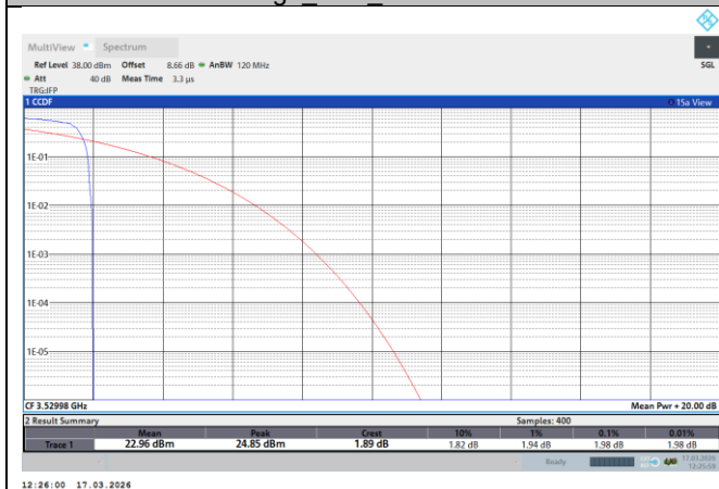
NTNV-N77-3450-3550-PC2-30-40-H-DFT-QPSK-Edge_1RB_Left-PASS
