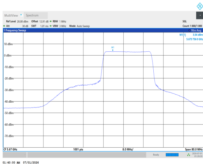
11BE40MIMO_Ant1_5710_UNII-2C_242Tone_RU61
