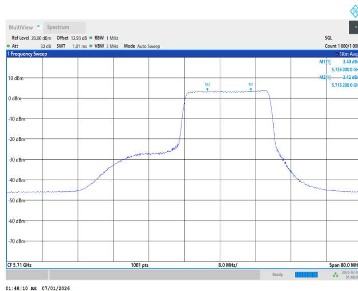
11BE40MIMO_Ant1_5710_UNII-3_242Tone_RU61
