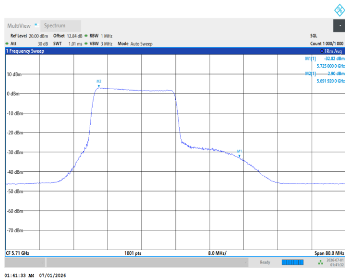
11BE40MIMO_Ant1_5710_UNII-2C_242Tone_RU62
