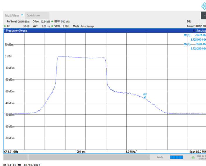
11BE40MIMO_Ant1_5710_UNII-3_242Tone_RU62
