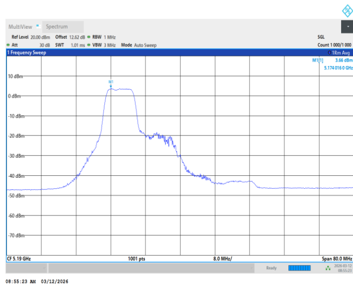
11BE40MIMO_Ant2_5190_26+106Tone_ /
