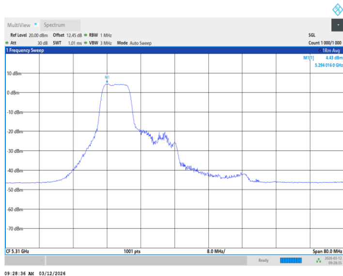
11BE40MIMO_Ant1_5310_26+106Tone_ /
