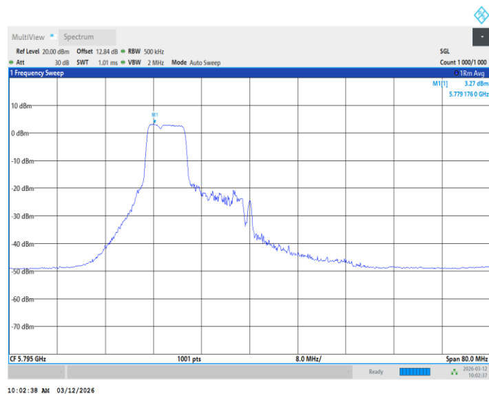
11BE40MIMO_Ant1_5795_26+106Tone_ /
