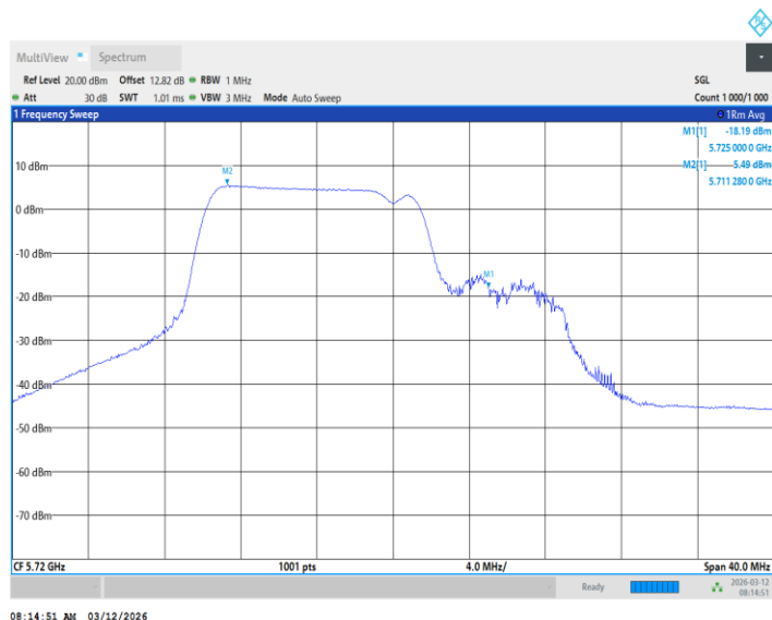
11BE20MIMO_Ant1_5720_UNII-3_26+52Tone_ /
