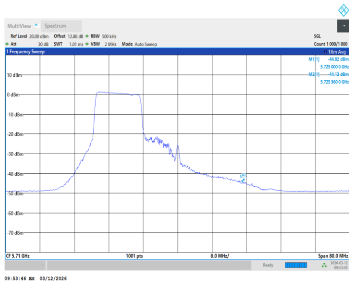
11BE40MIMO_Ant2_5710_UNII-3_26+52Tone_ /
