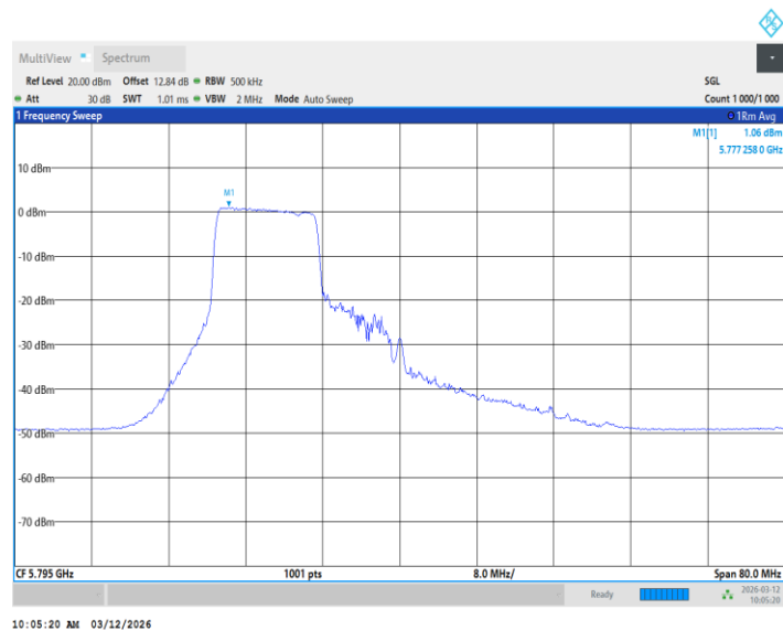
11BE40MIMO_Ant2_5795_26+52Tone_ /
