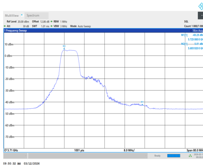
11BE40MIMO_Ant1_5710_UNII-2C_26+106Tone_ /
