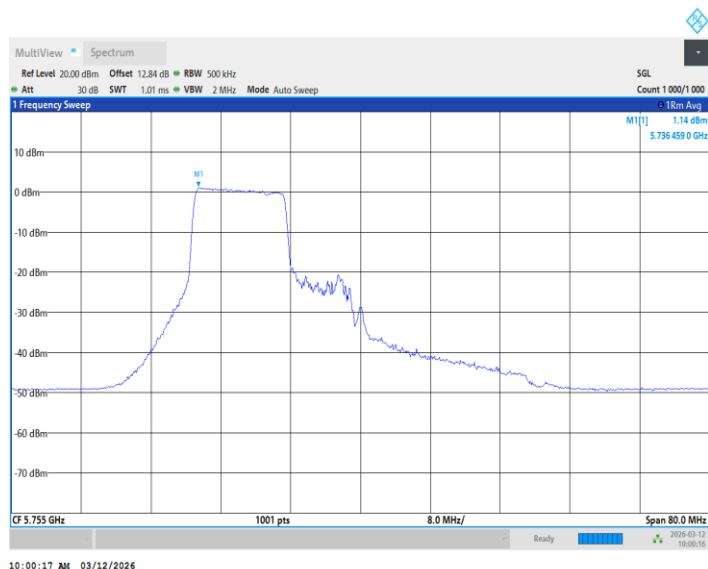
11BE40MIMO_Ant2_5755_26+52Tone_ /
