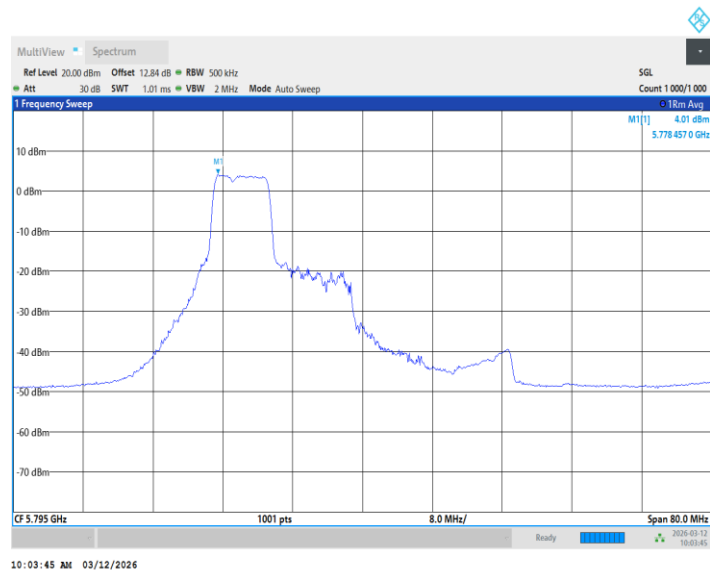
11BE40MIMO_Ant2_5795_26+106Tone_ /
