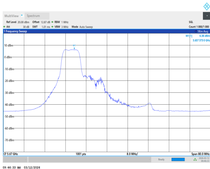
11BE40MIMO_Ant2_5670_26+106Tone_ /
