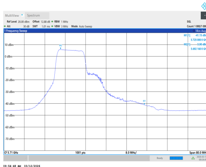
11BE40MIMO_Ant1_5710_UNII-3_26+52Tone_ /
