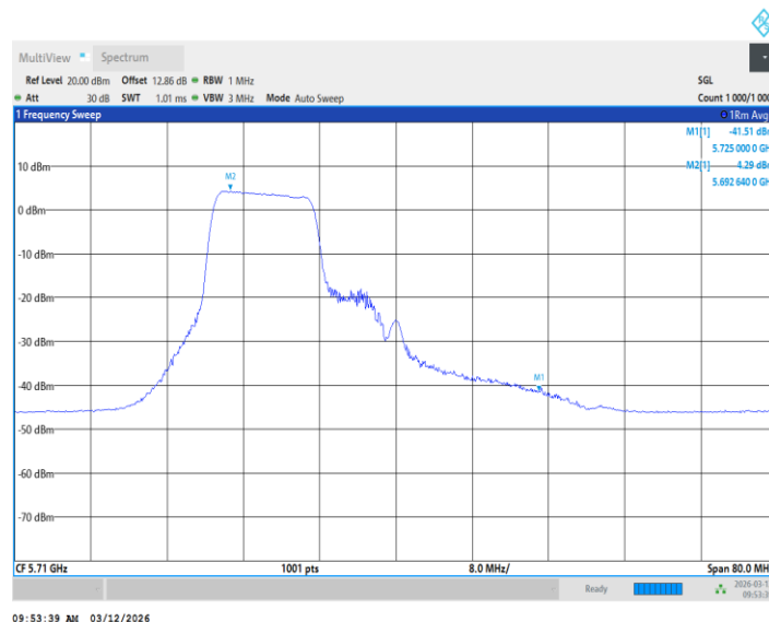
11BE40MIMO_Ant2_5710_UNII-2C_26+52Tone_ /
