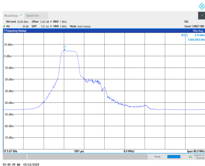
11BE40MIMO_Ant1_5670_26+106Tone_ /
