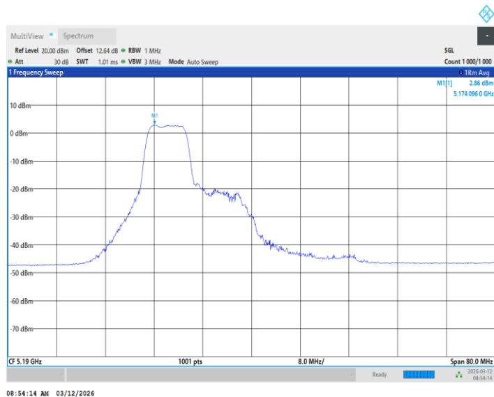
11BE40MIMO_Ant1_5190_26+106Tone_ /
