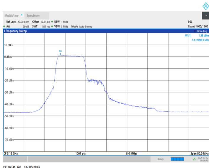
11BE40MIMO_Ant2_5190_26+52Tone_ /
