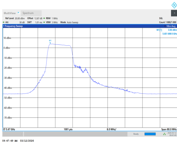
11BE40MIMO_Ant2_5670_26+52Tone_ /
