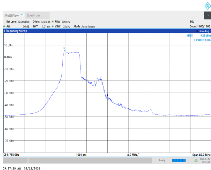
11BE40MIMO_Ant2_5755_26+106Tone_ /
