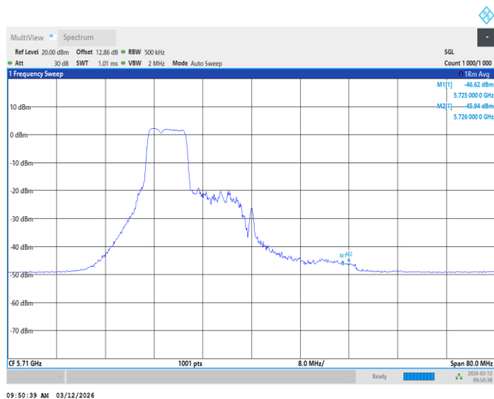
11BE40MIMO_Ant1_5710_UNII-3_26+106Tone_ /
