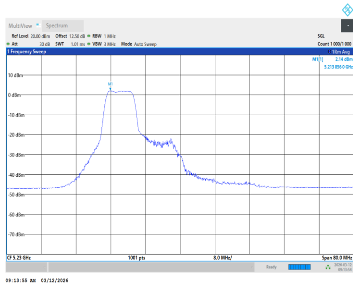
11BE40MIMO_Ant1_5230_26+106Tone_ /
