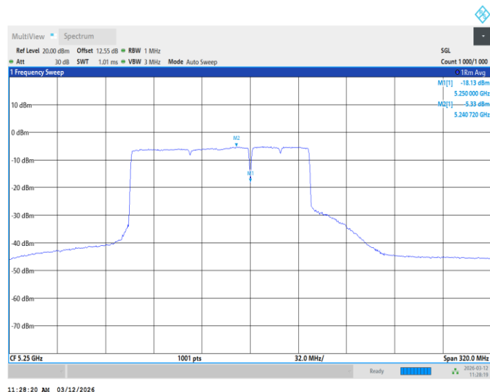
11BE160MIMO_Ant1_5250_UNII-2A_484+996Tone_ /
