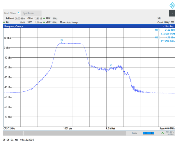
11BE20MIMO_Ant1_5720_UNII-2C_26+106Tone_ /
