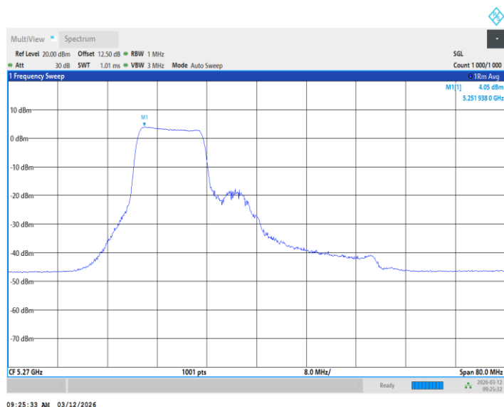
11BE40MIMO_Ant2_5270_26+52Tone_ /
