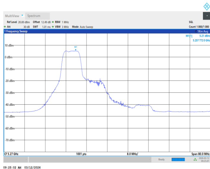
11BE40MIMO_Ant2_5270_26+106Tone_ /
