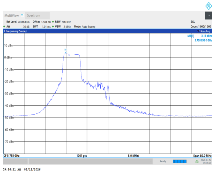
11BE40MIMO_Ant1_5755_26+106Tone_ /
