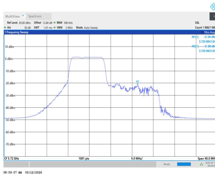
11BE20MIMO_Ant1_5720_UNII-3_26+106Tone_ /
