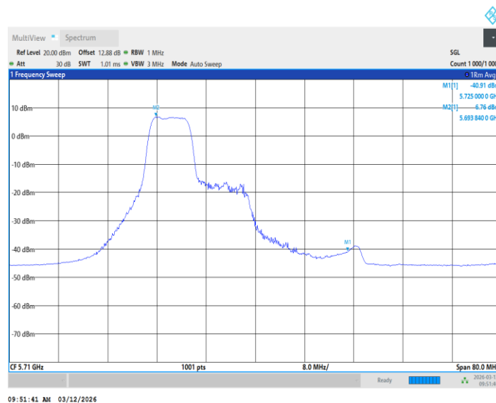
11BE40MIMO_Ant2_5710_UNII-2C_26+106Tone_ /
