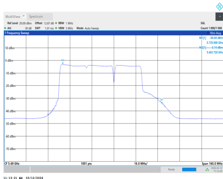
11BE80MIMO_Ant2_5690_UNII-2C_26+52Tone_ /
