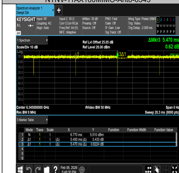
NTNV-11AX160MIMO-Ant6-6345
