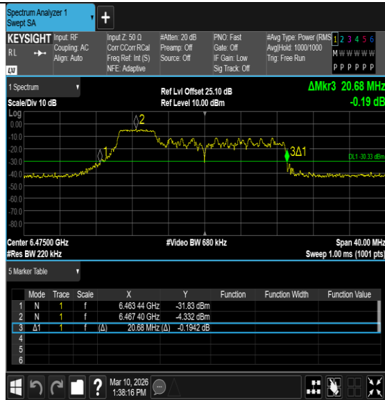
11BE20MIMO-Ant6-6475-52Tone-RU38-PASS
