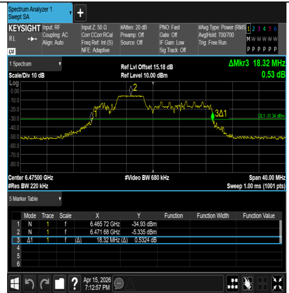
11BE20MIMO-Ant7-6475-52Tone-RU40-PASS
