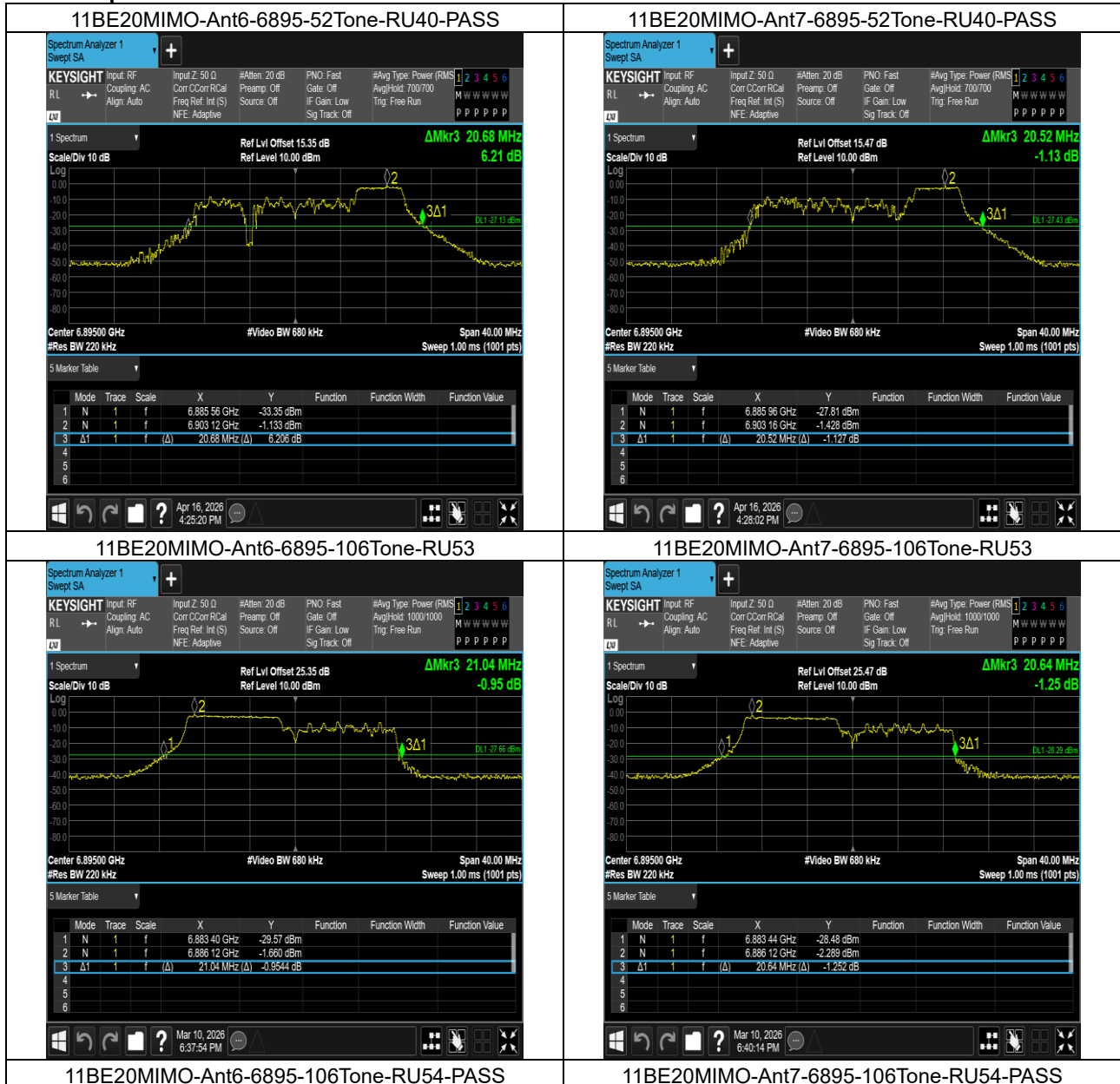
11BE20MIMO-Ant6-6895-106Tone-RU54-PASS
