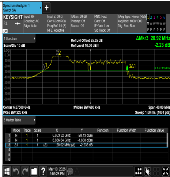
11BE20MIMO-Ant6-6875-52Tone-RU38-PASS
