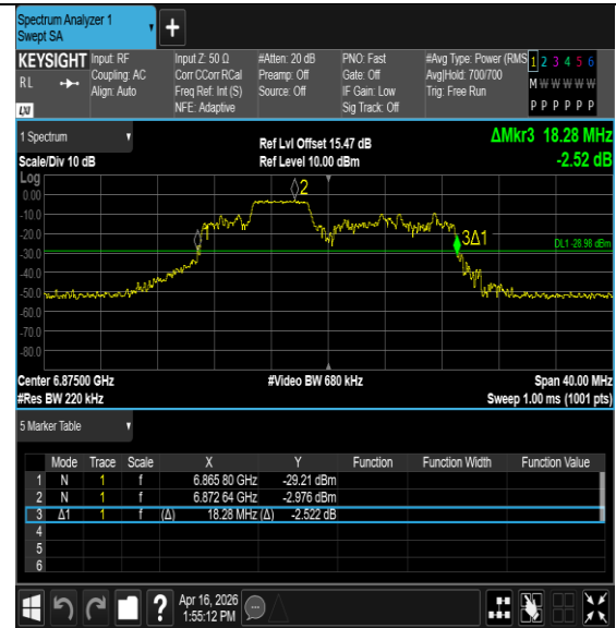
11BE20MIMO-Ant7-6875-52Tone-RU40-PASS
