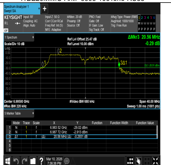
11BE20MIMO-Ant7-6995-106Tone-RU53
